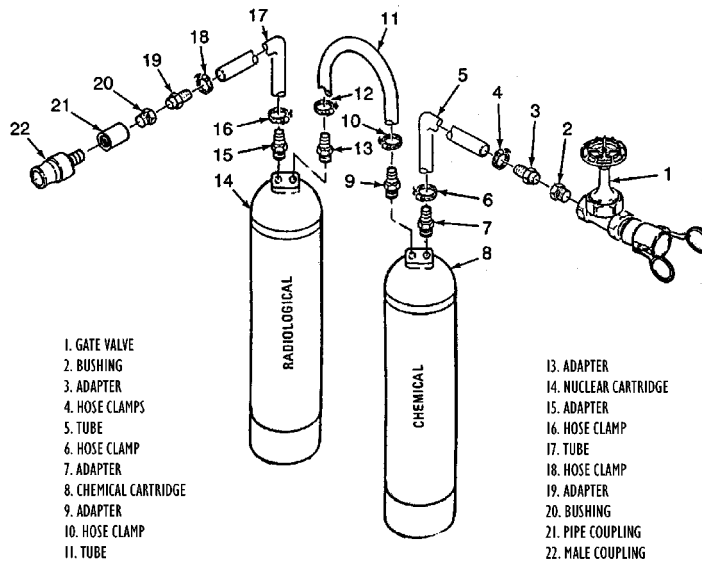
Figure 53. Deionization Cartridge Assembly.
