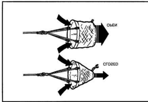
Figure 16-2. Sea anchor.
