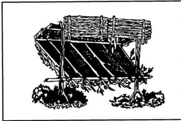
Figure 2-8. Field-expedient lean-to and fire reflector.
