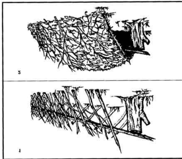
Figure 2-11. Deep pit
