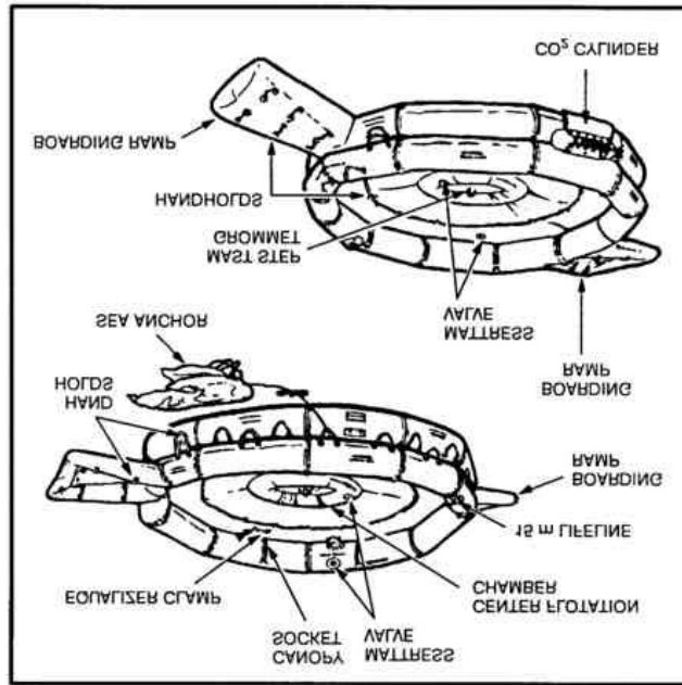
Figure 10-12. Twenty-man raft
