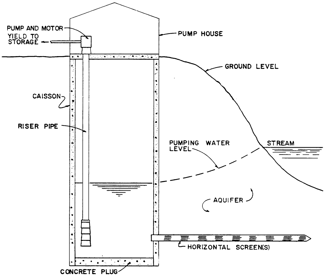
Figure 5-2. Driven well.
