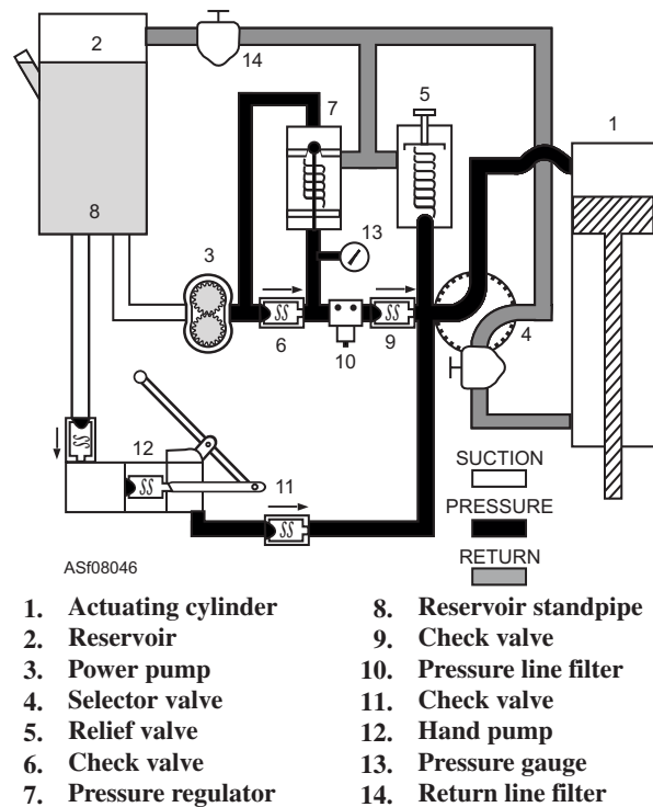
Figure 8-46.—Complete hydraulic system.
