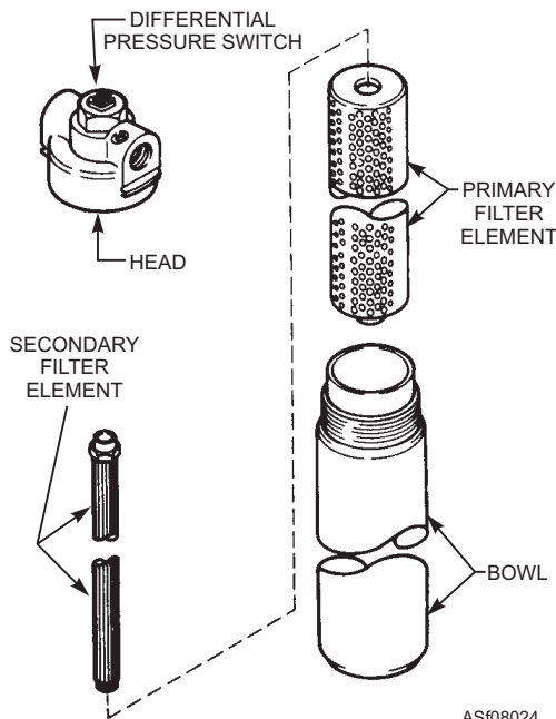
Figure 8-24.—High-pressure filter.
