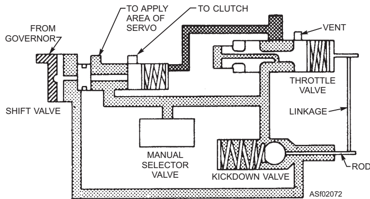
Figure 2-72.—Functional shift valve controls.
