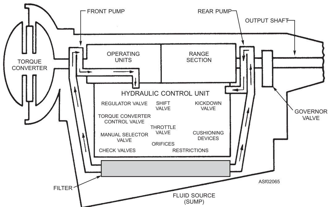
Figure 2-65.—Typical hydraulic control unit and its components.
