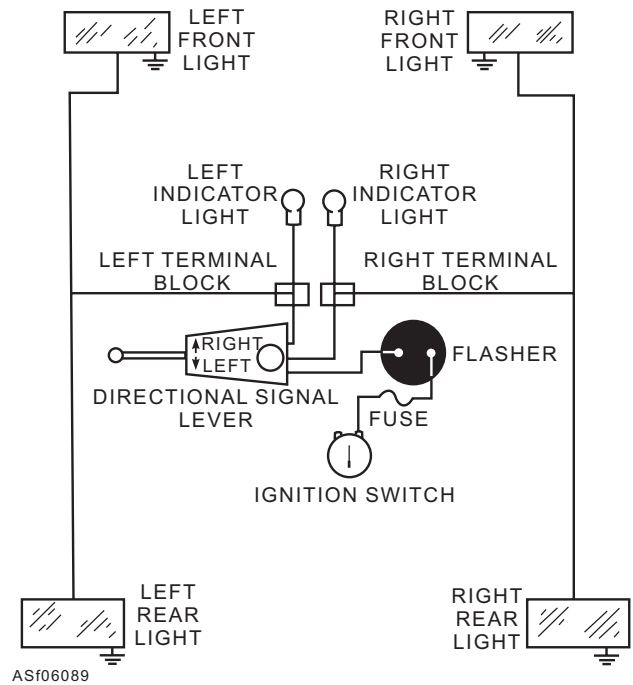
Figure 6-89.—Pictorial diagram of a directional signal system.
