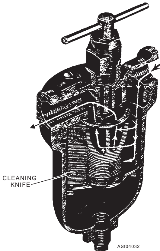
Figure 4-32.—Metal disc fuel filter.
