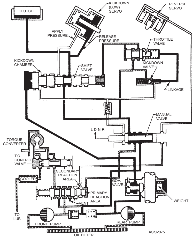
POWER FLOW IN DIRECT DRIVE
