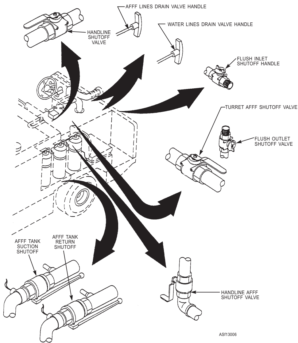
Figure 13-6.—Controls and indicators.
