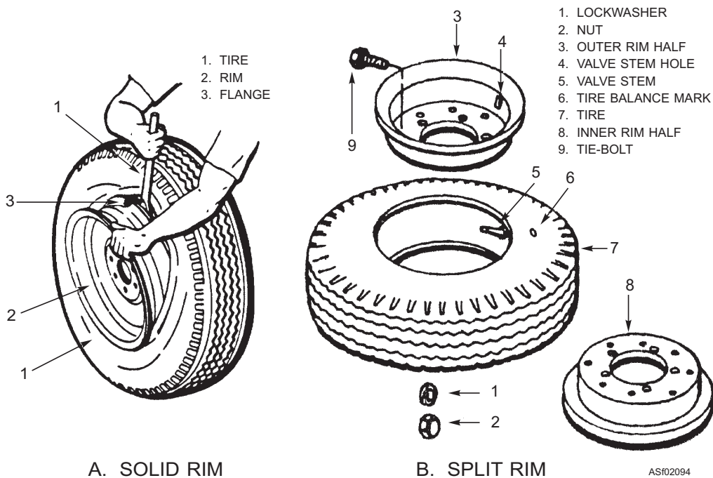
Figure 2-94.—Solid and split rims.
