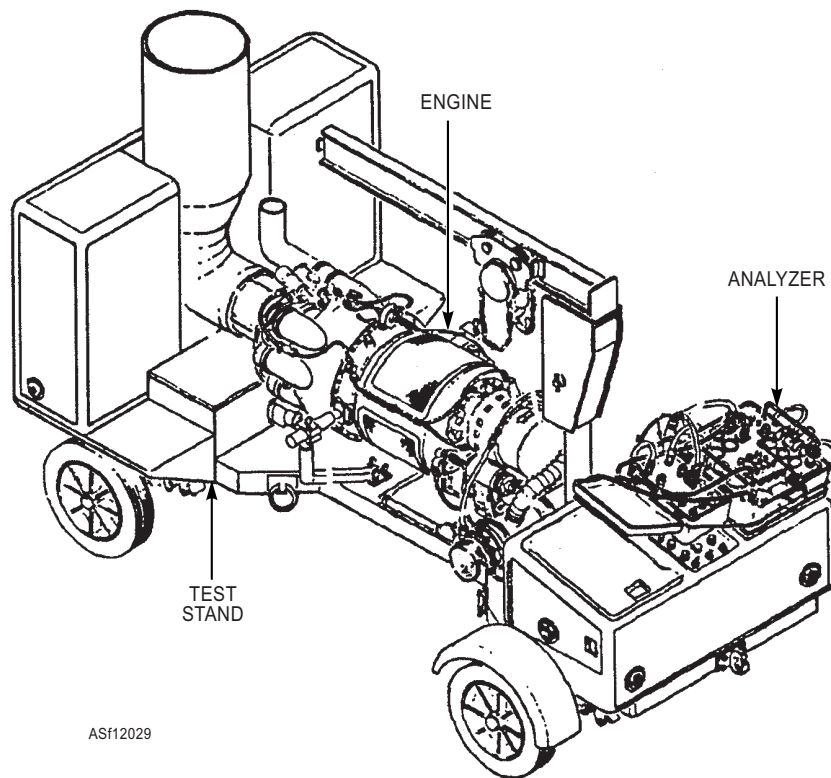
Figure 12-29.—Analyzer connected to engine installed in test stand.
