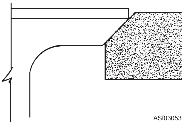
Figure 3-53.—Valve seat too wide and low in block.
