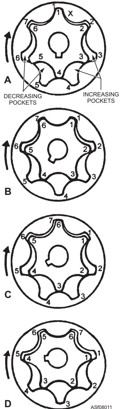
Figure 8-11.—Principles of operation of the internal gear group.
