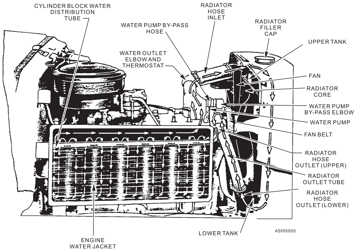
Figure 5-2.—Liquid-cooling system.
