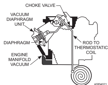
Figure 4-21.—Automatic choke with thermostatic coil mounted in manifold.
