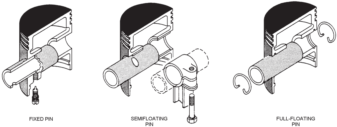
Figure 3-29.—Piston pin types.
