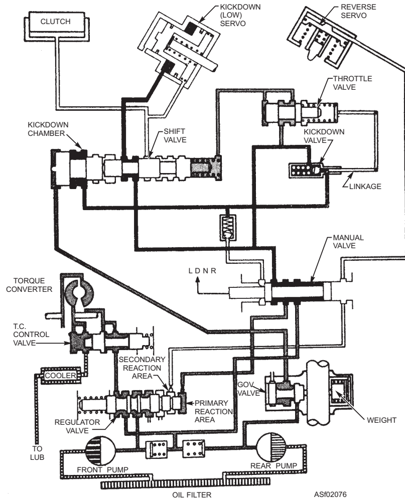
Figure 2-76.—“Kickdown” forced shift position.
