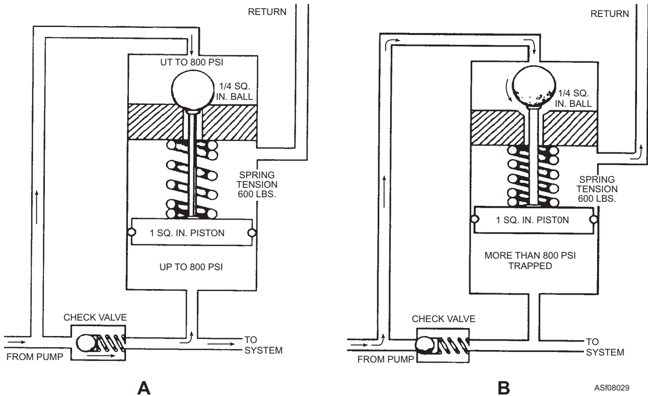
Figure 8-29.—Pressure regulator in the cut-in state (view A); and the cut-out state (view B).
