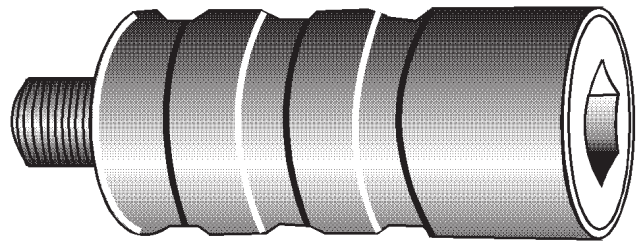
Figure 3-51.—Valve seat grinding stone sleeve.
