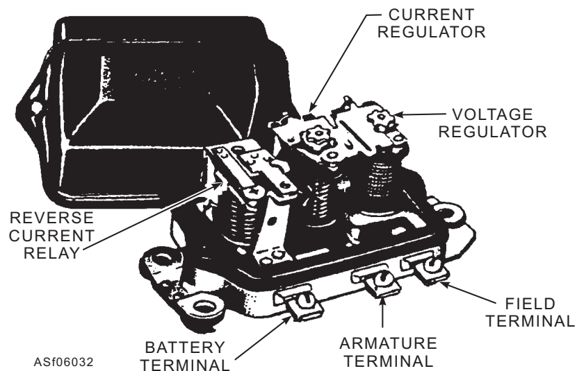
Figure 6-32.—Three-unit, vibrating contact, dc regulator.
