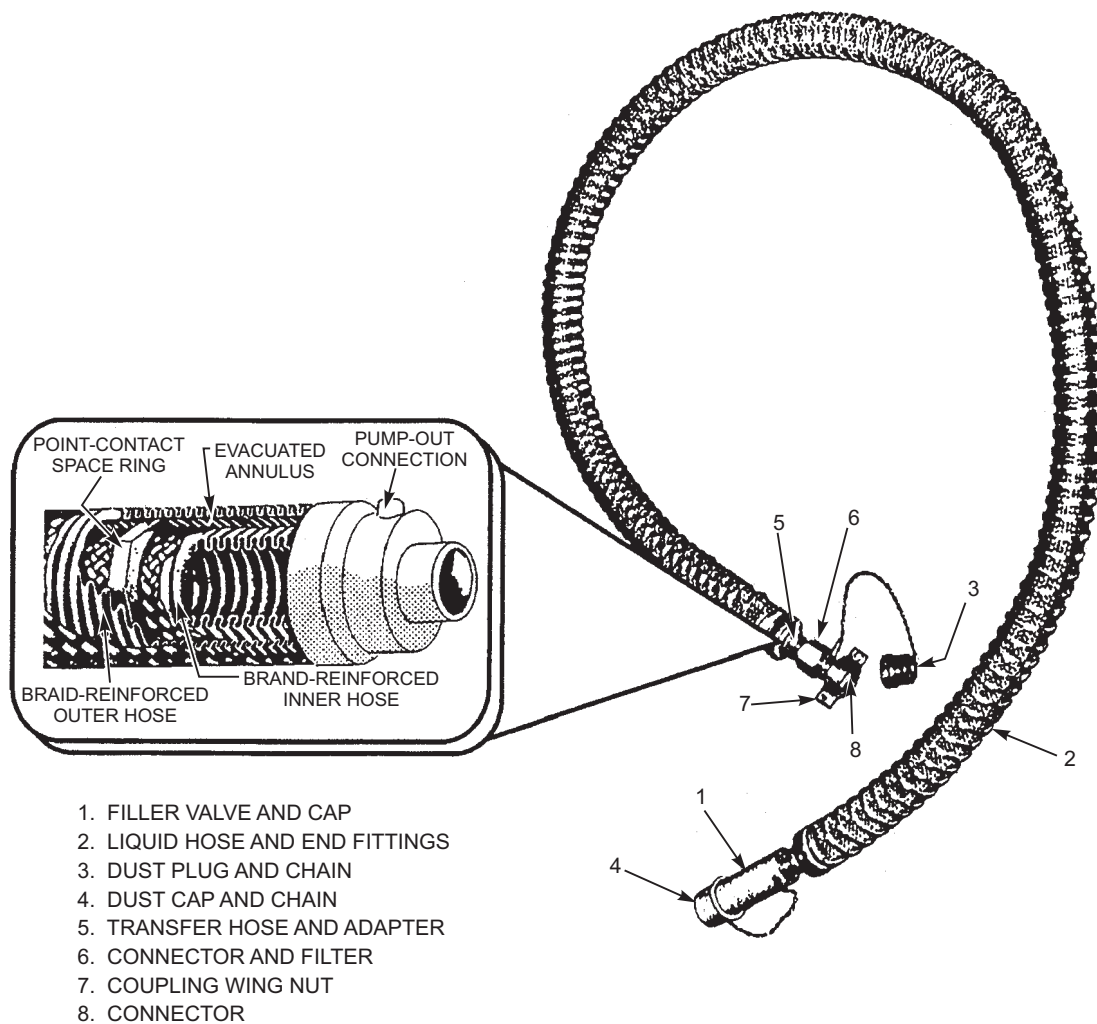
Figure 10-3.—Corrugated flexible metal hose.
