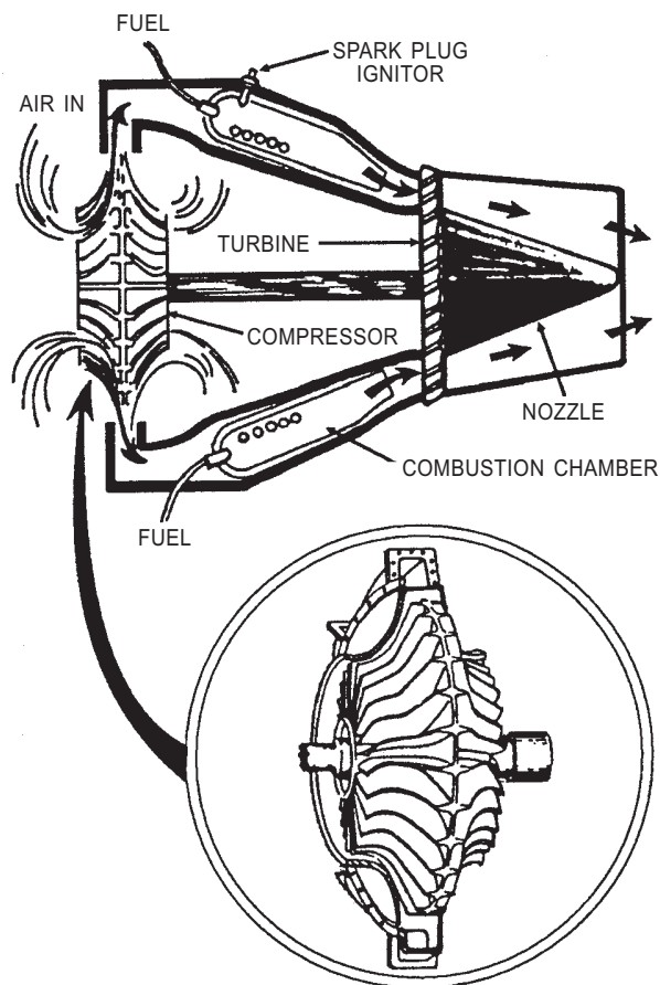
COMPRESSOR - CENTRIFUGAL - FLOW (DOUBLE - ENTRY TYPE)
