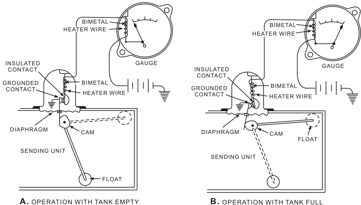
Figure 6-76.—Thermostatic fuel gauge circuit.
