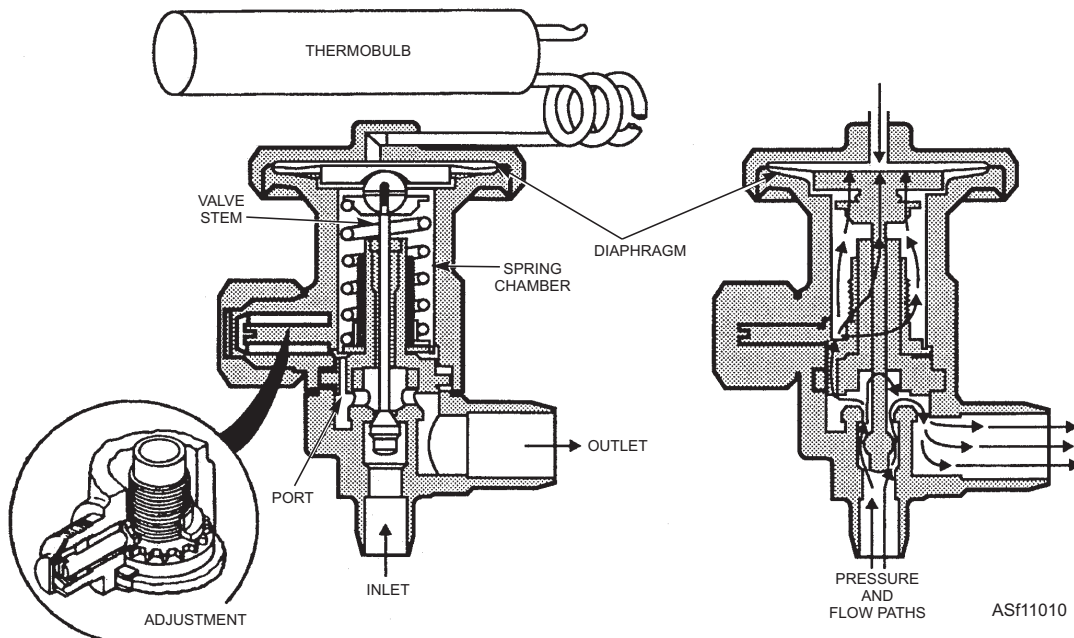
Figure 11-10.—Thermostatic expansion valve.
