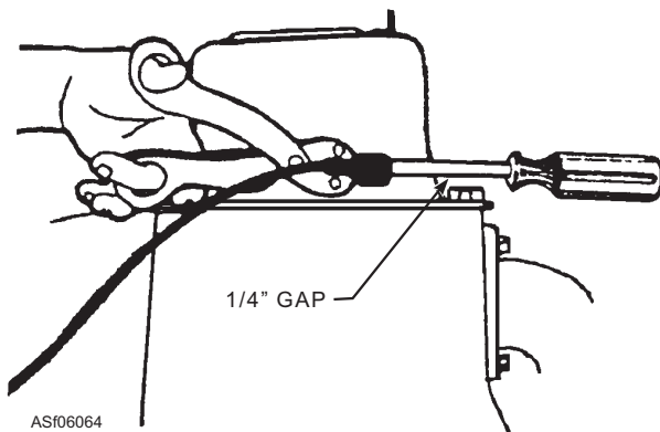
Figure 6-64.—Checking for spark at the plug.
