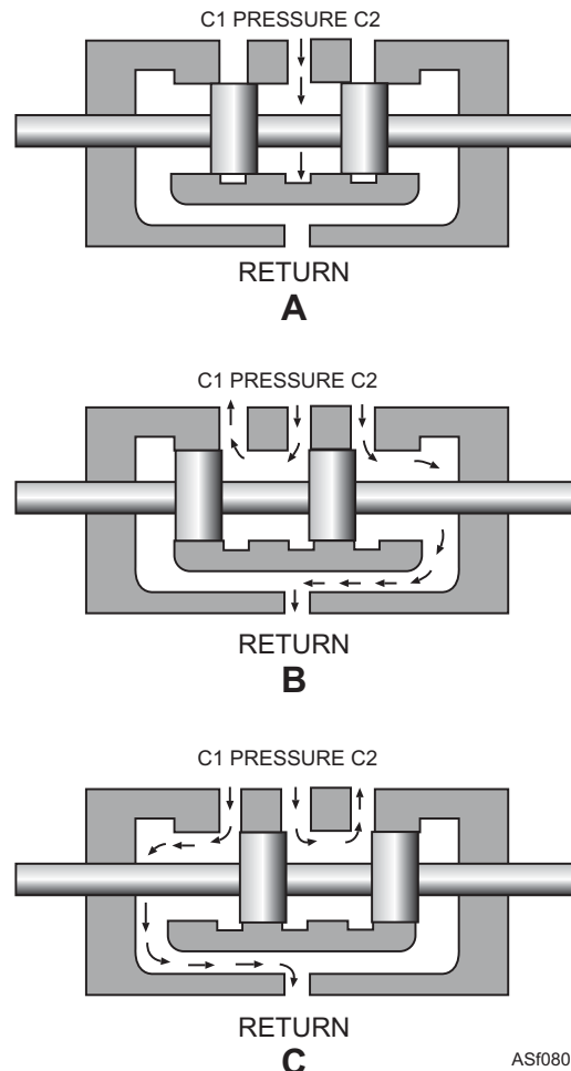
Figure 8-33.—Closed-center directional control valve.
