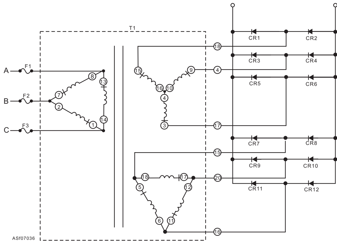
Figure 7-36.—A dc power supply circuit.
