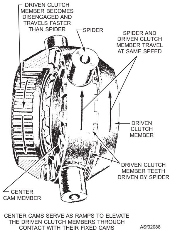
Figure 2-88.—Action of a center cam during a turn.
