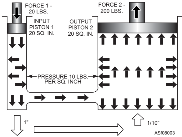
Figure 8-3.—Multiplication of forces.
