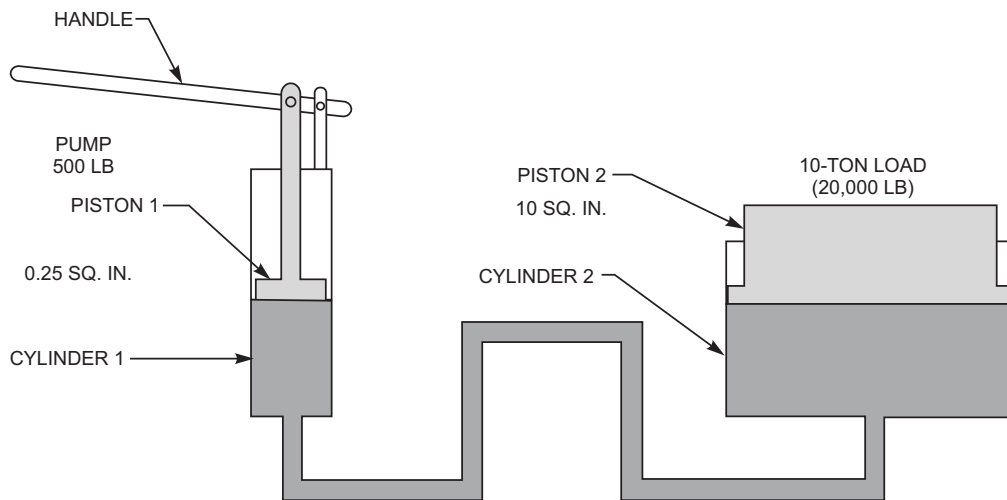
Figure 8-4.—A 10-ton hydraulic jack.
