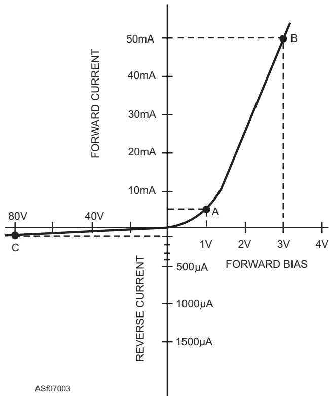
Figure 7-3.—PN junction diode characteristic curve.
