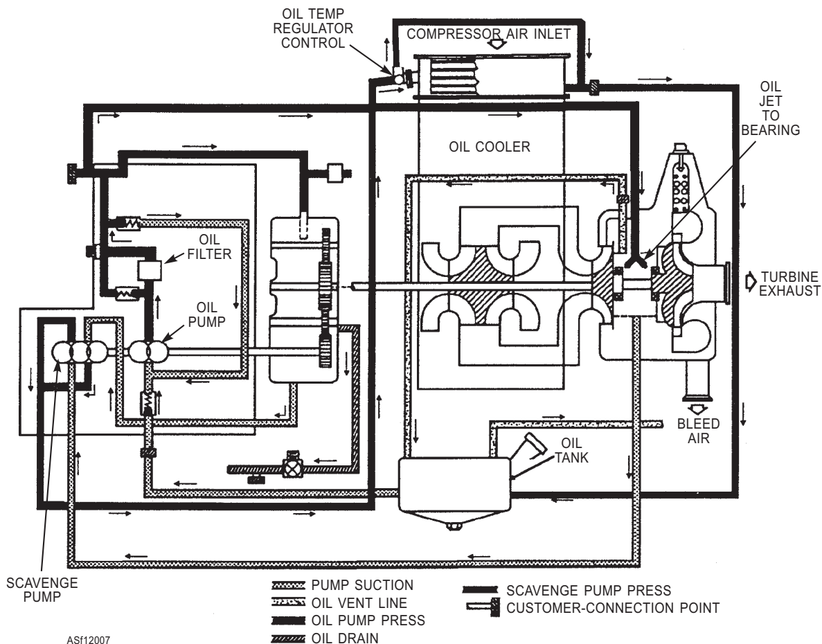
Figure 12-7.—Lubrication system.
