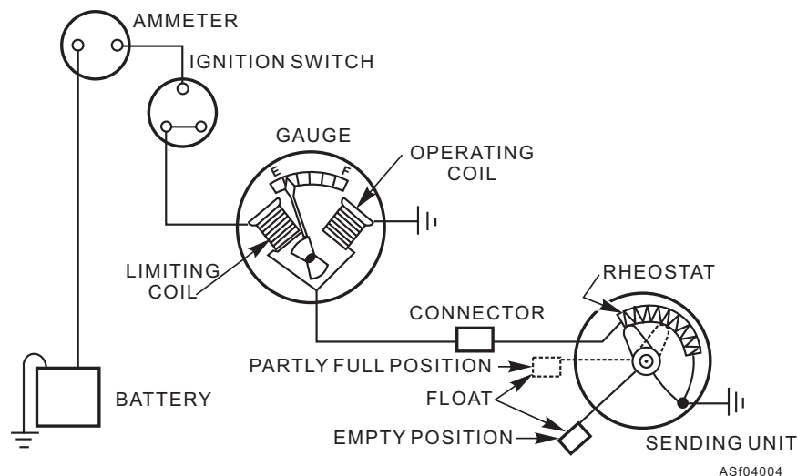
Figure 4-4.—Coil-type gauge circuit.
