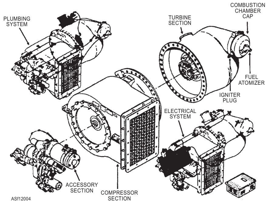
Figure 12-4.—Major sections of a gas turbine compressor (GTC-85).
