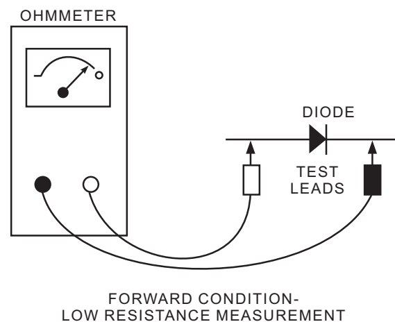
Figure 7-5.—Checking a diode with an ohmmeter.
