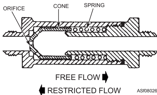
Figure 8-26.—One-way restrictor (check valve).
