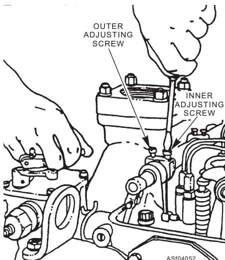
Figure 4-52.—Positioning rear injector rack control lever.
