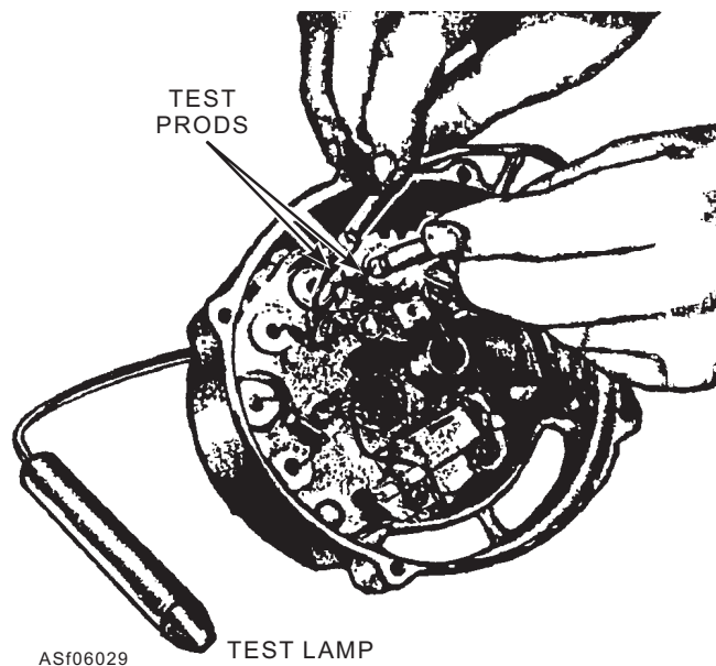
Figure 6-29.—Testing diodes with a test lamp.
