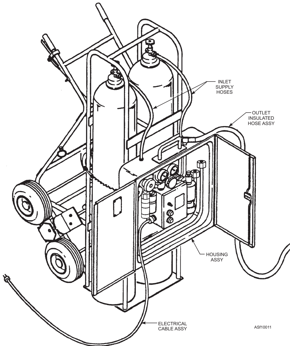
Figure 10-11.—Aircraft liquid oxygen system gas purging set.
