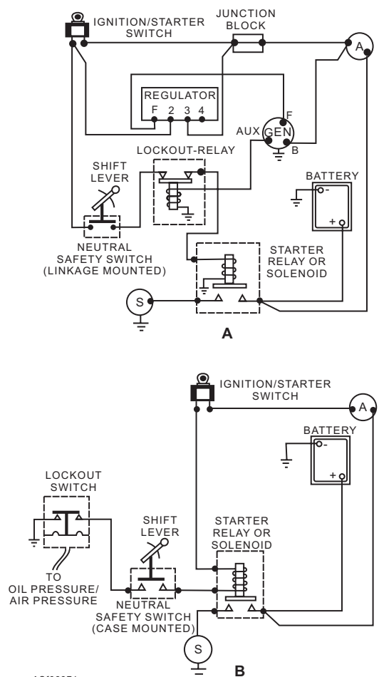
Figure 6-71.—Starter safety control combinations.
