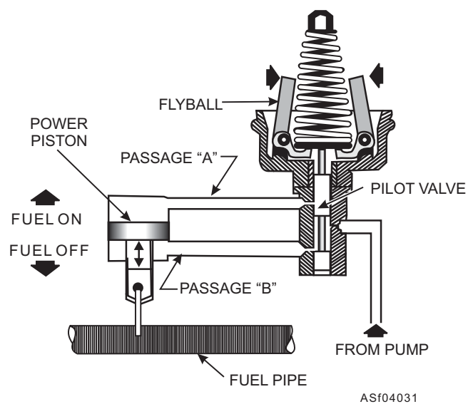
Figure 4-31.—Simple hydraulic governor.
