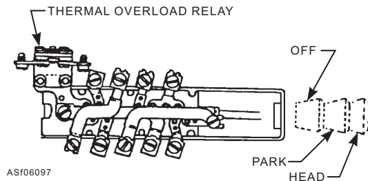
Figure 6-97.—Main light switch.
