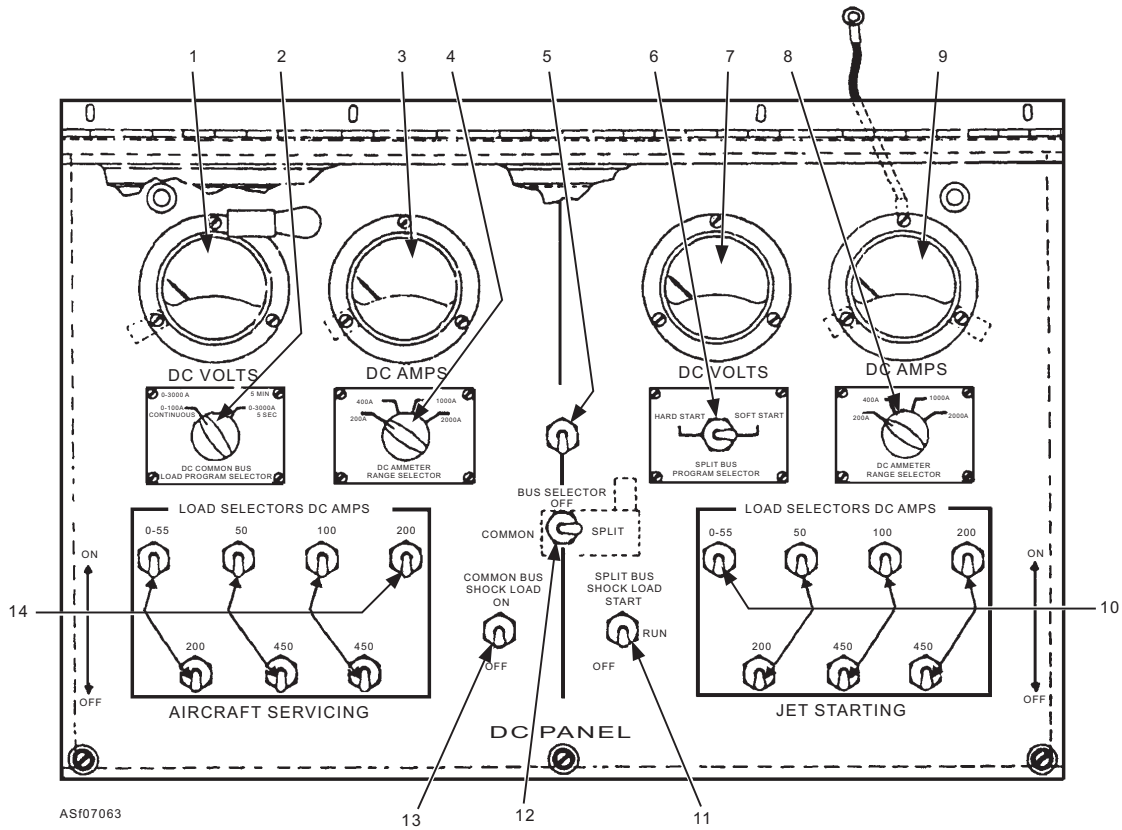
Figure 7-63.—DC control panel.
