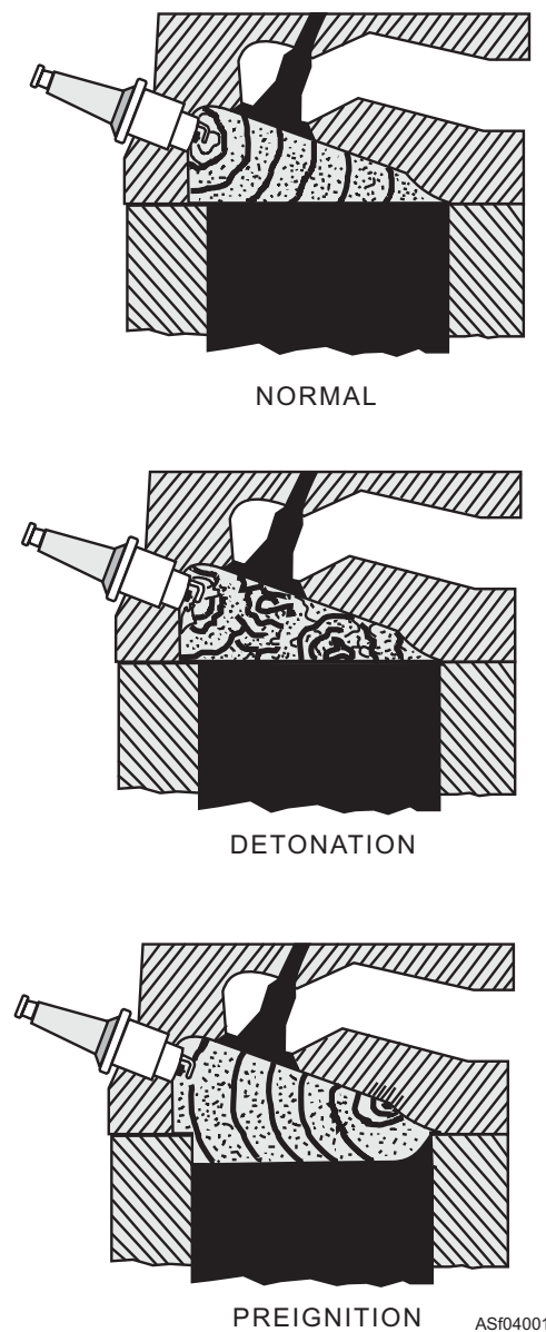
Figure 4-1.—Combustion process.
