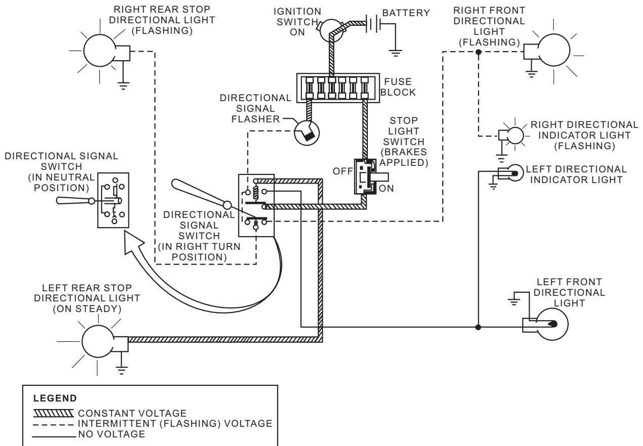
Figure 6-90.—A representative stop-directional light system.
