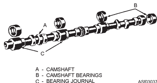
Figure 3-37.—Camshaft and bushings.
