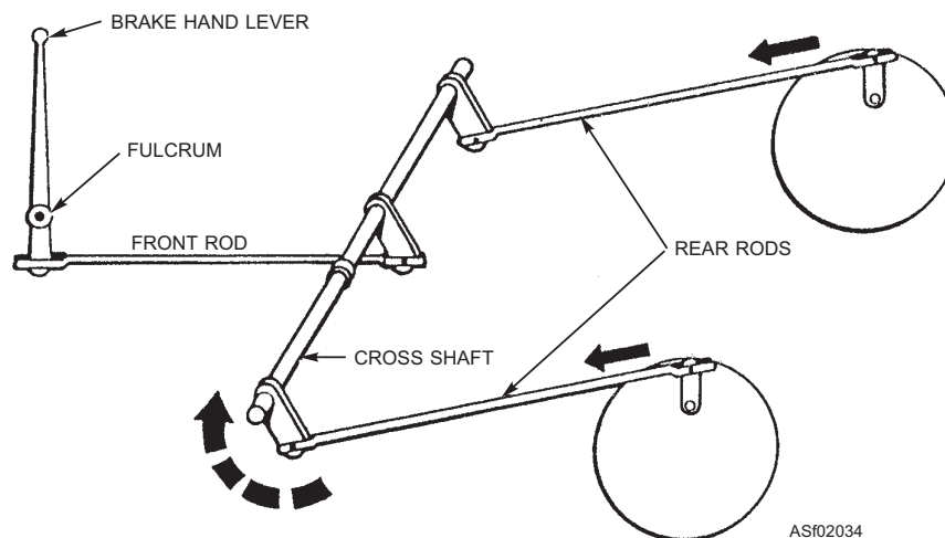
Figure 2-34.—Mechanical brake system—rods and shaft.
