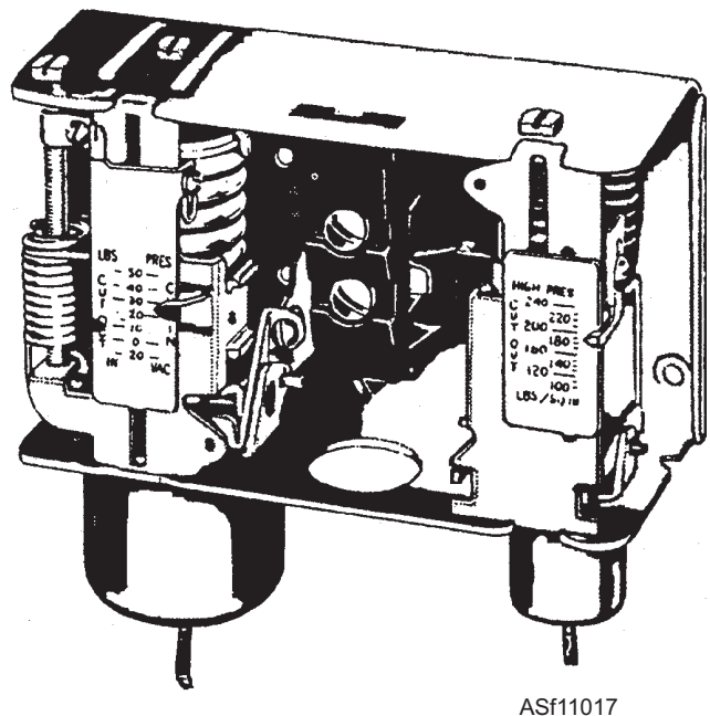
Figure 11-17.—High- and low-pressure safety control cutouts.
