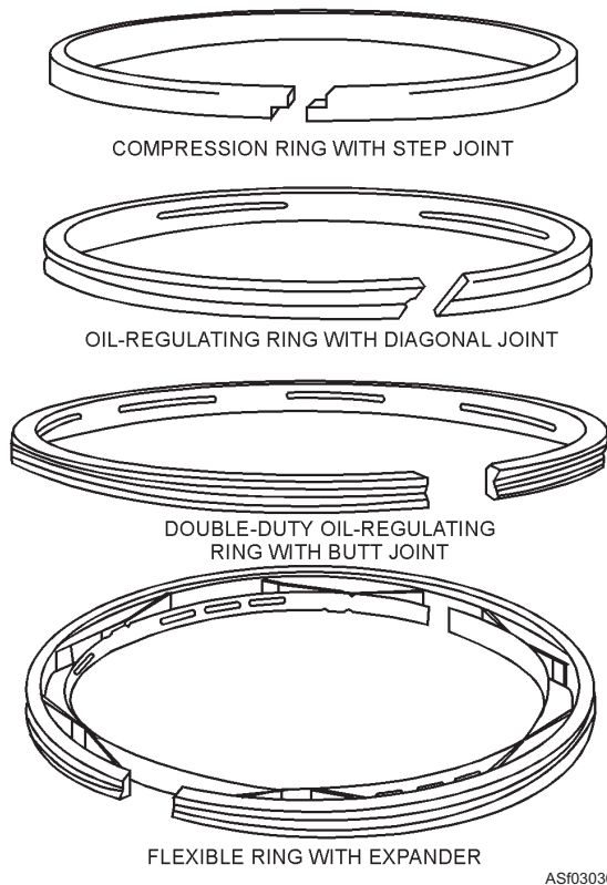
Figure 3-30.—Piston rings.
