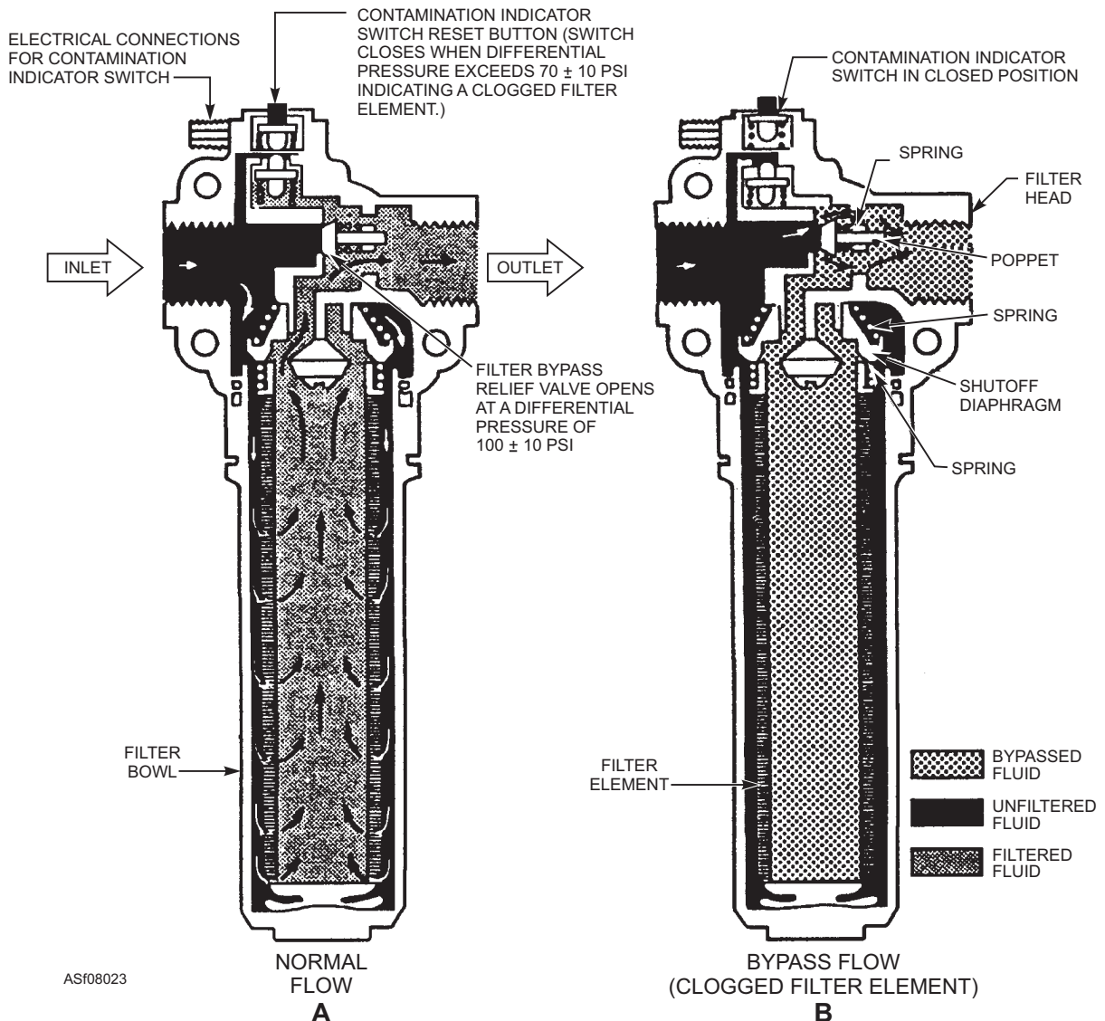
Figure 8-23.—Full flow bypass, electrical indicating hydraulic filter.
