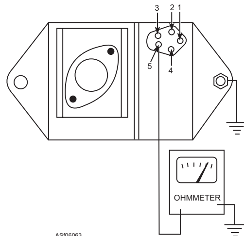
Figure 6-63.—Control unit No. 5 test.
