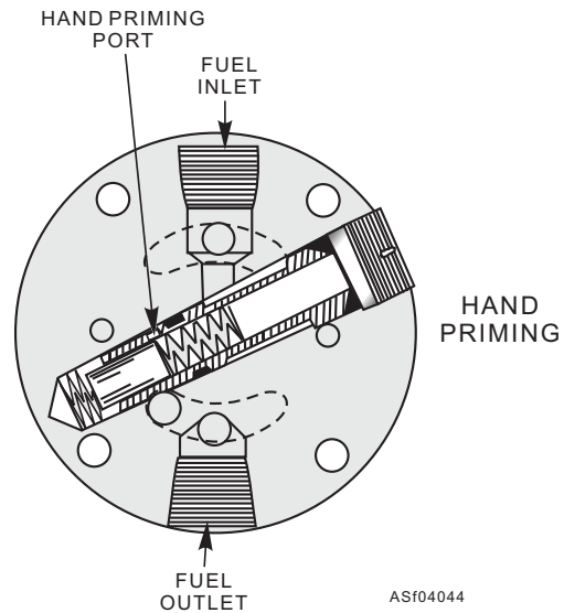
Figure 4-44.—Regulating piston during hand priming.
