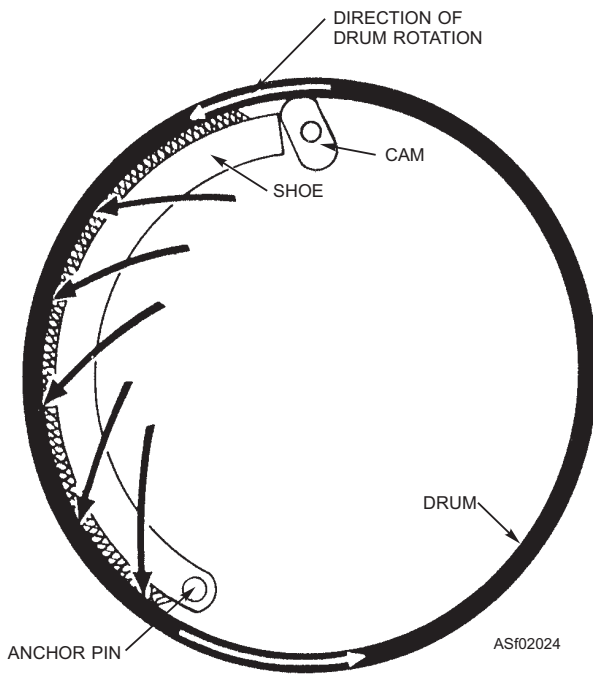
Figure 2-24.—Brake shoe self-energizing action.
