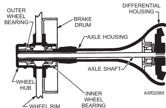
Figure 2-89.—Cross section of rear hub in full floating axle.
