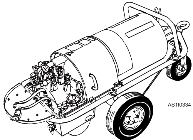
Figure 1-36.—TMU-70 liquid oxygen servicing unit.
