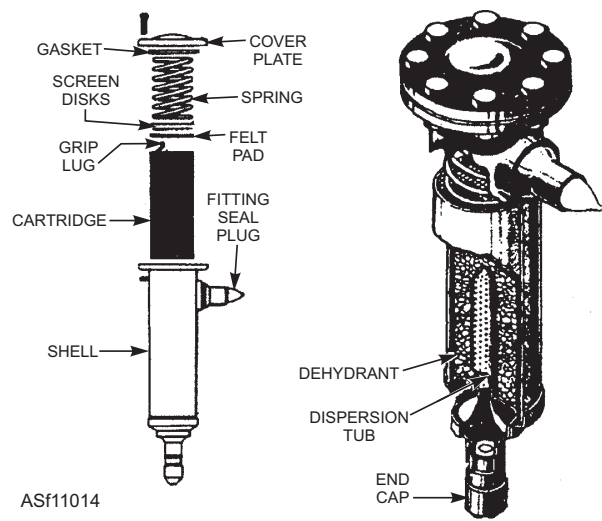
Figure 11-14.—Drier-strainer (dehydrator).
