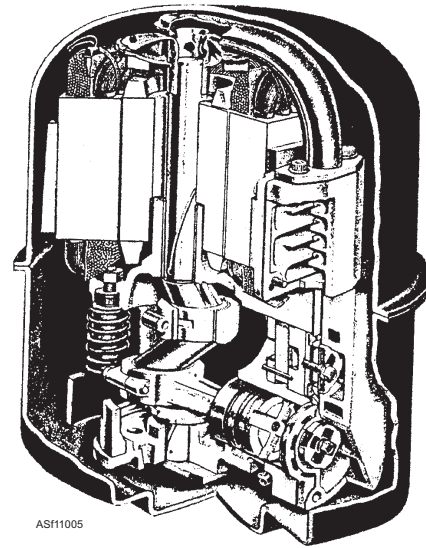
Figure 11-5.—Reciprocating hermetic compressor.
