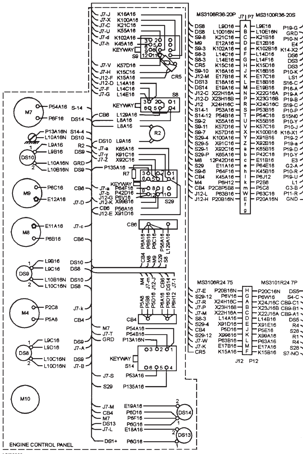
Figure 6-3.—Wiring diagram.
