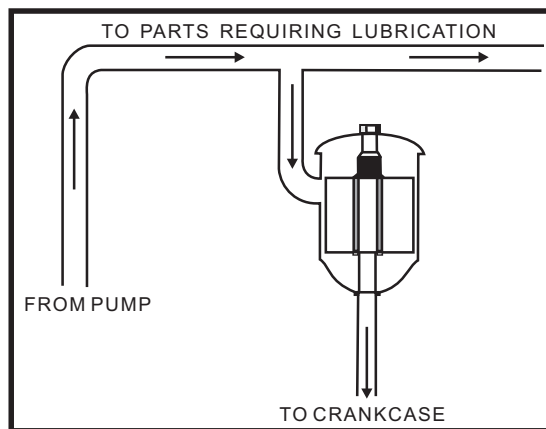
Figure 5-16.—Partial flow filter.
