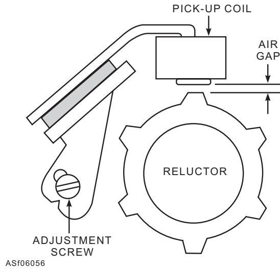
Figure 6-56.—Air gap adjustment.
