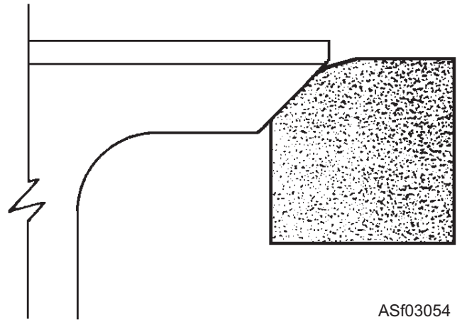
Figure 3-54.—Correct valve seat after narrowing seat.
