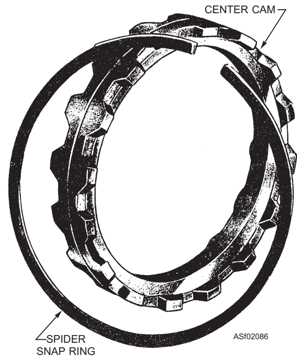
Figure 2-86.—Construction of center cam.
