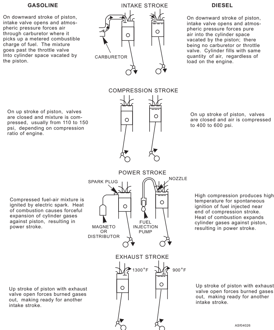
Figure 4-26.—Comparison of sequence of events in diesel and gasoline 4-cycle engines.
