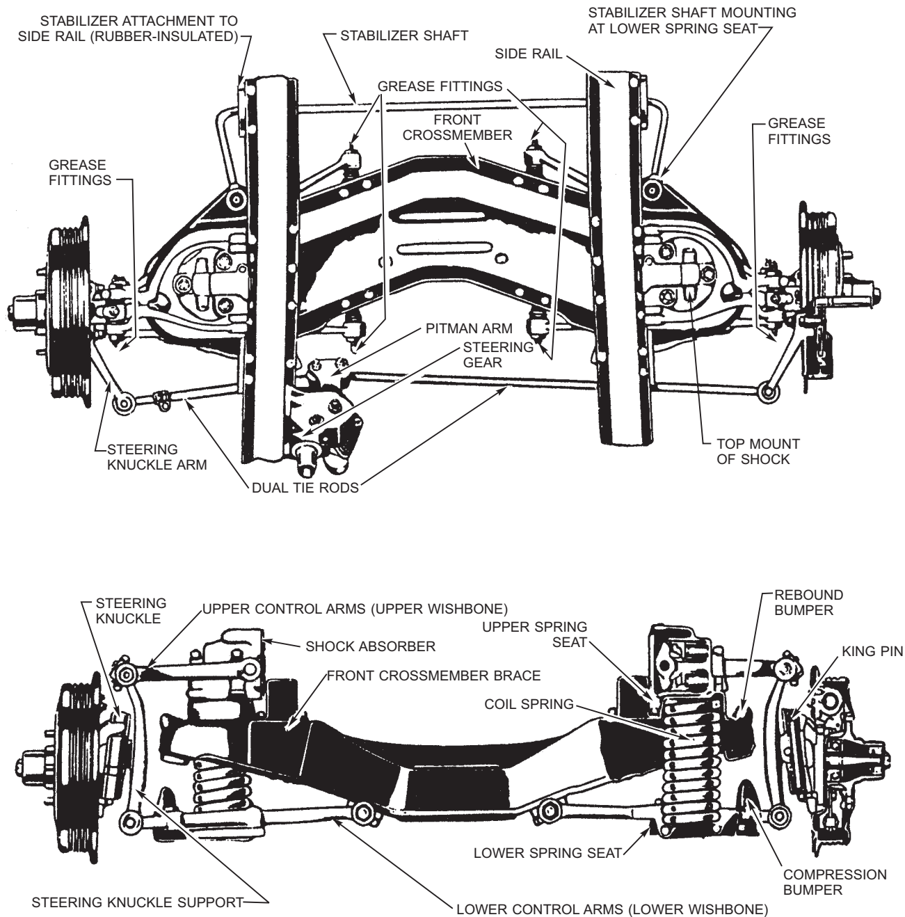
Figure 2-4.—Coil spring suspension.
