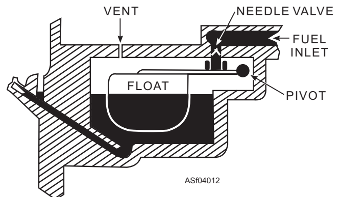
Figure 4-12.—A typical float circuit.
