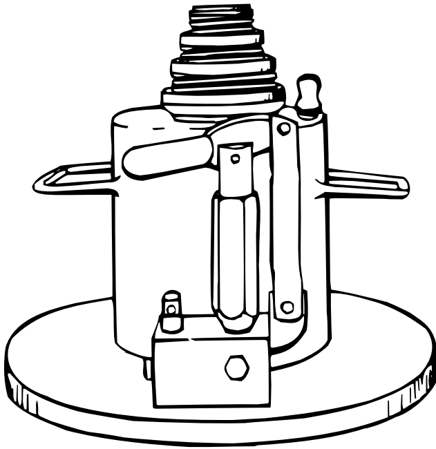
Figure 1-23.—A3-1HC axle jack.
