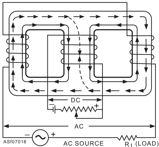
Figure 7-18.—Magnetic amplifier with three-legged core.
