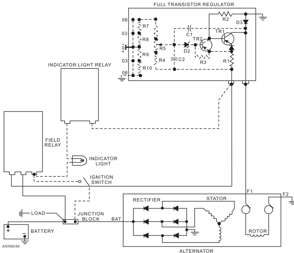
Figure 6-39.—Ac circuit using a fully transistorized regulator.
