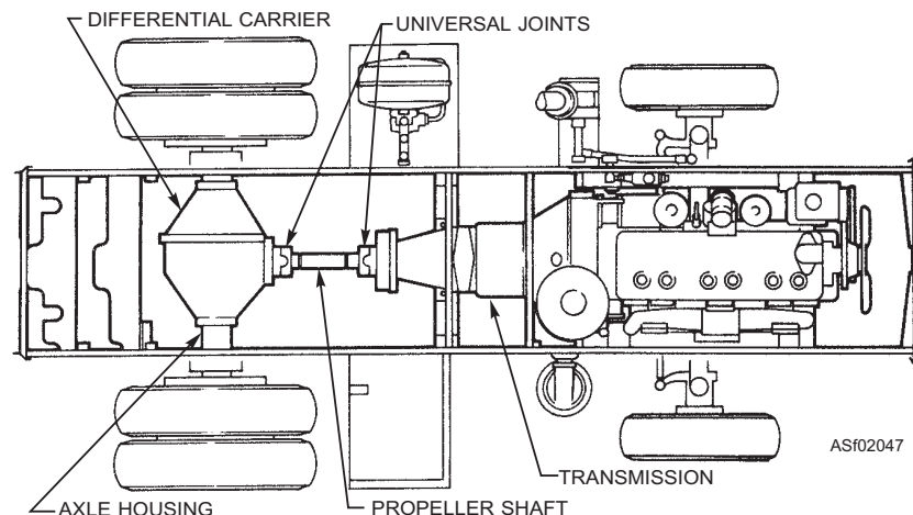
Figure 2-47.—Power train.
