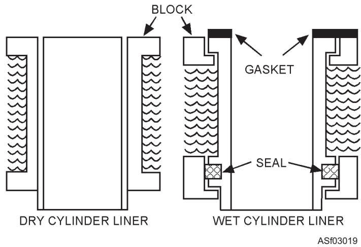
Figure 3-19.—Cylinder liner application.
