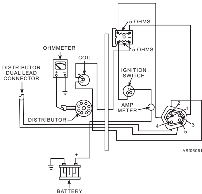
Figure 6-61.—Distributor dual lead test.
