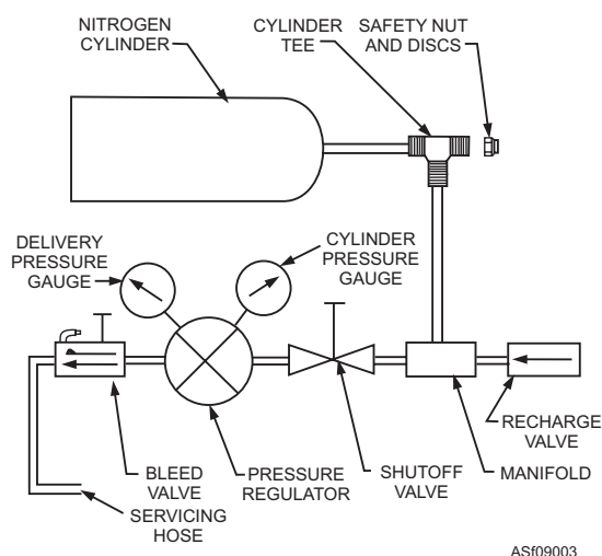
Figure 9-3.—Portable high-pressure nitrogen cylinder schematic.
