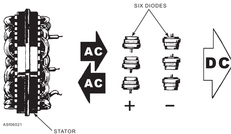
Figure 6-21.—Function of the alternator diode.
