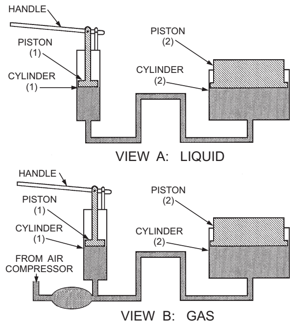
Figure 9-1.—Transmission of force by liquids and gases.
