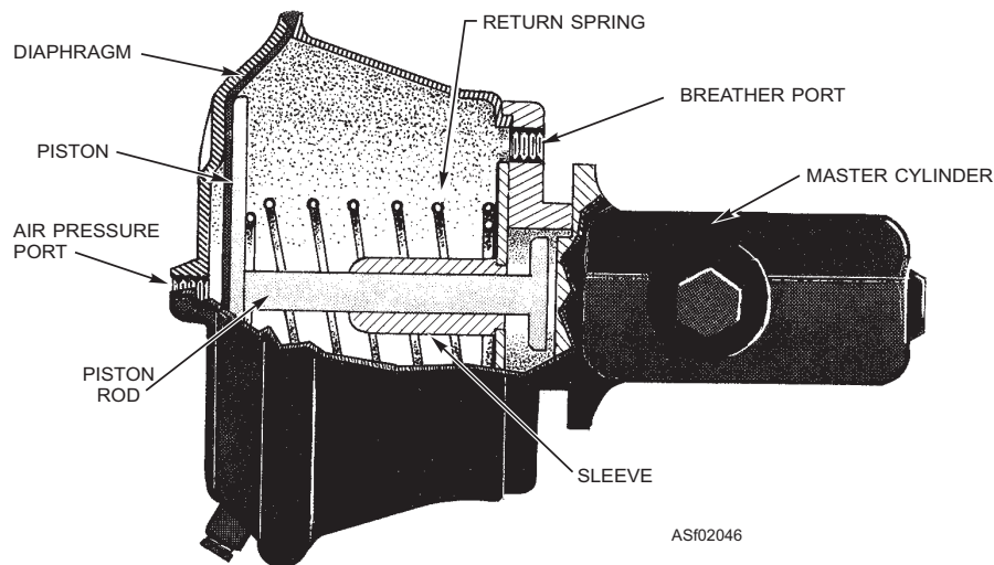
Figure 2-46.—Master cylinder assembly—air-over-hydraulic brake system.
