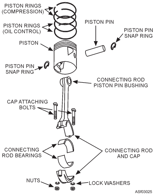
Figure 3-25.—Piston and connecting rod (exploded view).
