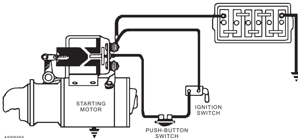
Figure 6-65.—Electric starting system.
