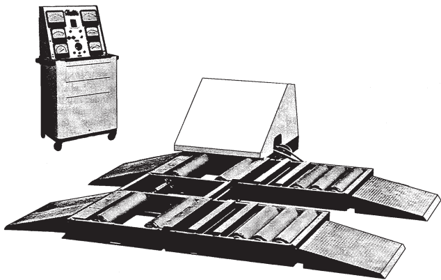
Figure 3-10.—Chassis dynamometer.
