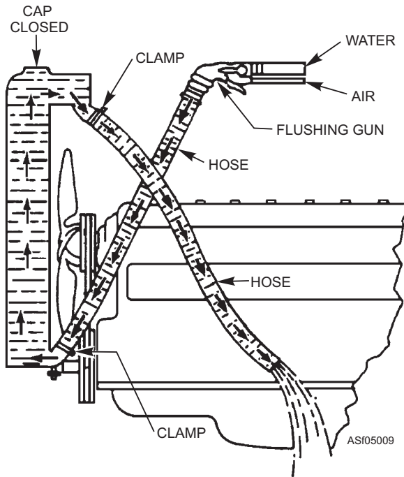
Figure 5-9.—Reverse flushing of radiator.
