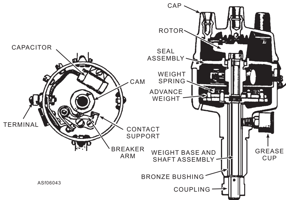
Figure 6-43.—Side and top view of a distributor.
