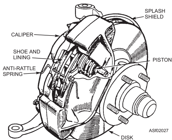
Figure 2-27.—Disc brake assembly.
