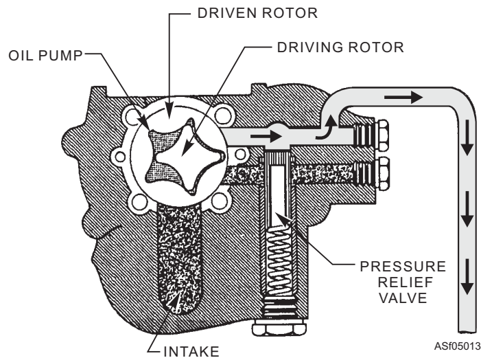
Figure 5-13.—Rotary oil pump.
