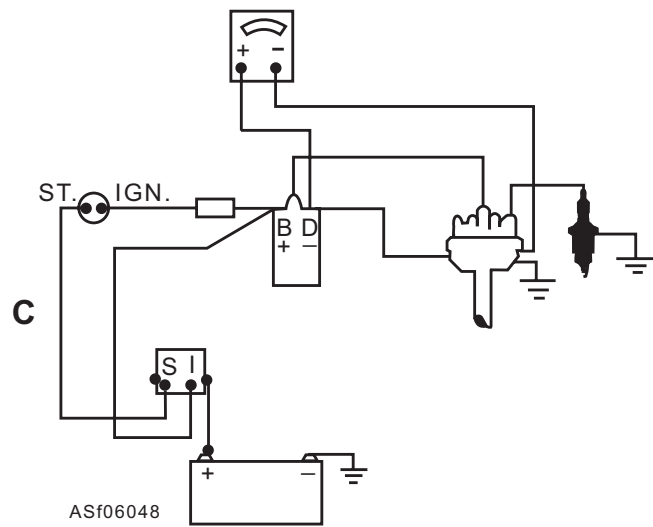
Figure 6-48.—Voltmeter connections for resistance tests of the primary circuit.
