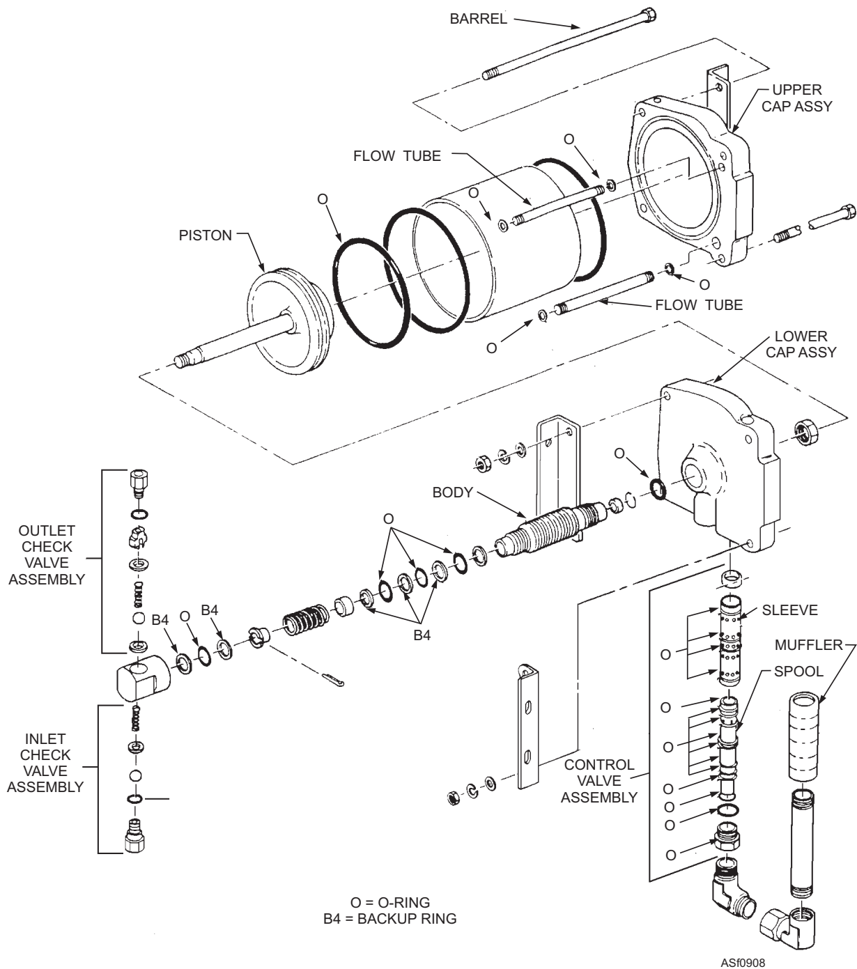
Figure 9-8.—Motor and pump assembly.
