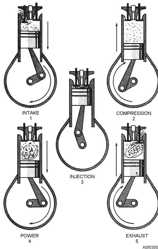
Figure 3-8.—Four-stroke cycle diesel engine.
