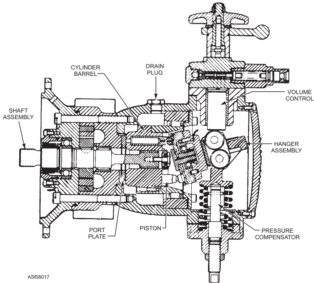
Figure 8-17.—Variable displacement axial piston pump.
