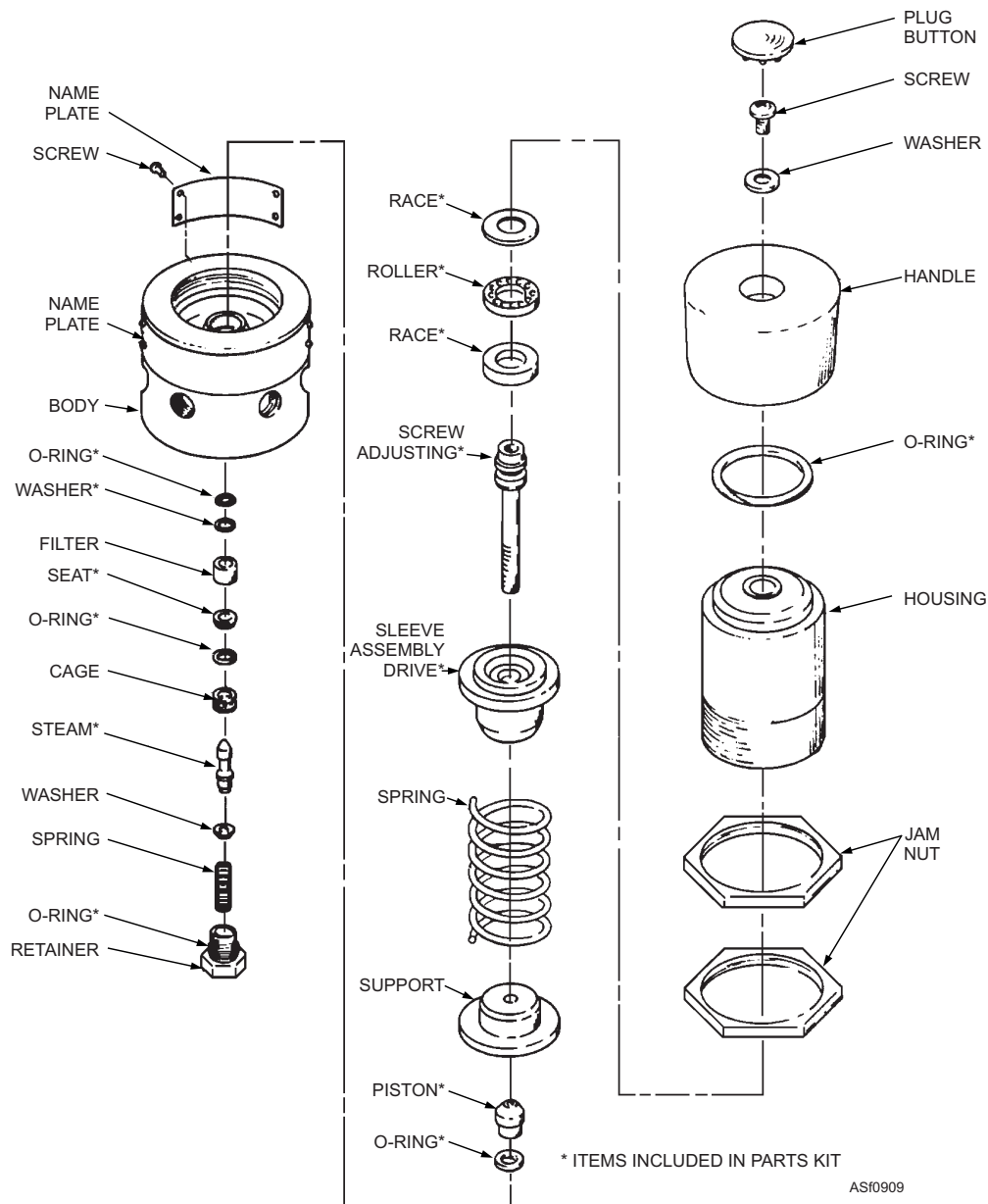
Figure 9-9.—Pressure regulator assembly.
