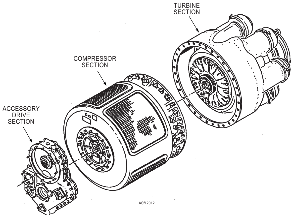
Figure 12-12.—GTCP-100 gas turbine engine sections.
