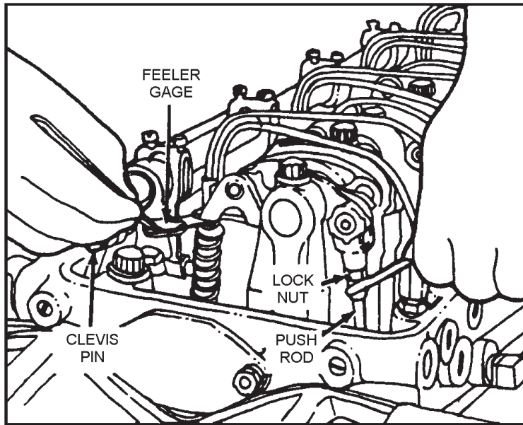
Figure 3-41.—Adjusting valve clearance.
