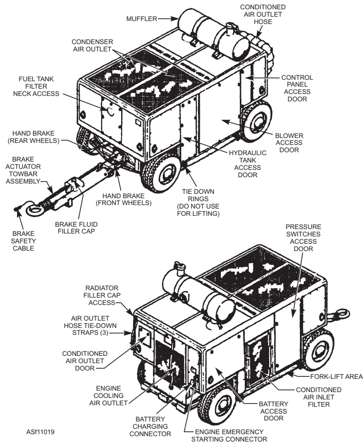
Figure 11-19.—A/M32C-17 trailer-mounted air-conditioning unit, diesel-powered.
