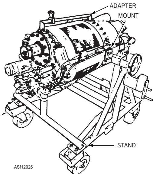
Figure 12-26.—Engine mounted on 281270-0-3 portable maintenance stand.
