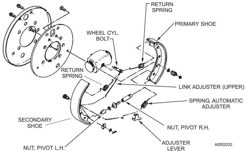
Figure 2-32.—Brake assembly, self-adjusting.
