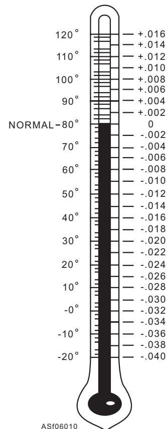
Figure 6-10.—Specific gravity temperature correction chart.
