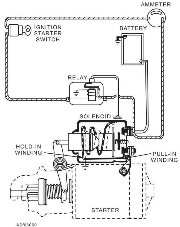
Figure 6-69.—Control system for a starter with overrunning clutch drive.
