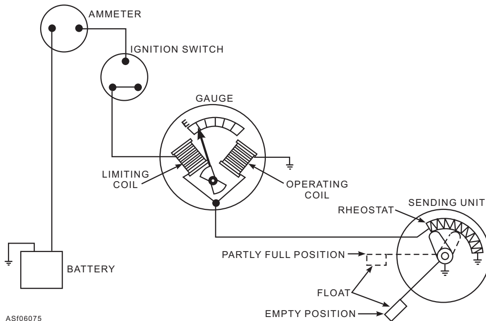
Figure 6-75.—Coil operated fuel gauge circuit.
