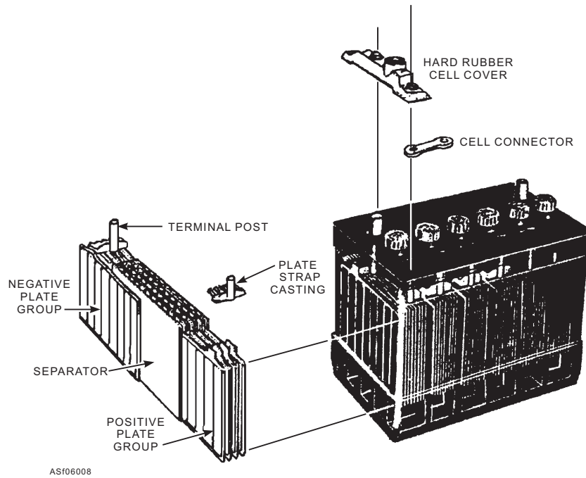
Figure 6-8.—Battery construction.
