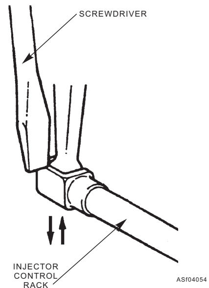
Figure 4-54.—Checking injector rack “spring” action.
