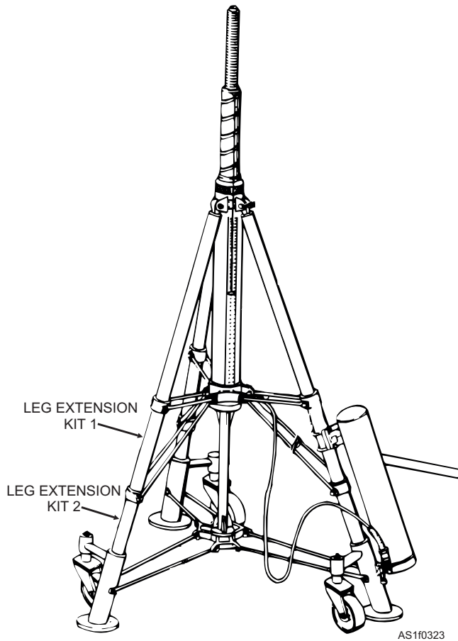
Figure 1-25.—Variable height tripod jack, two-leg extension.
