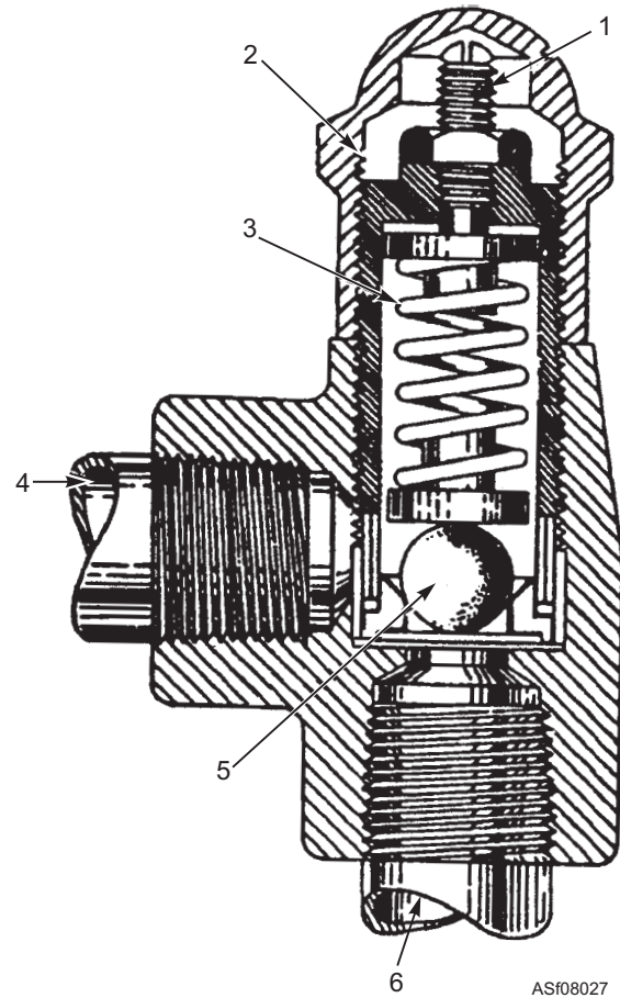
Figure 8-27.—Relief valve.
