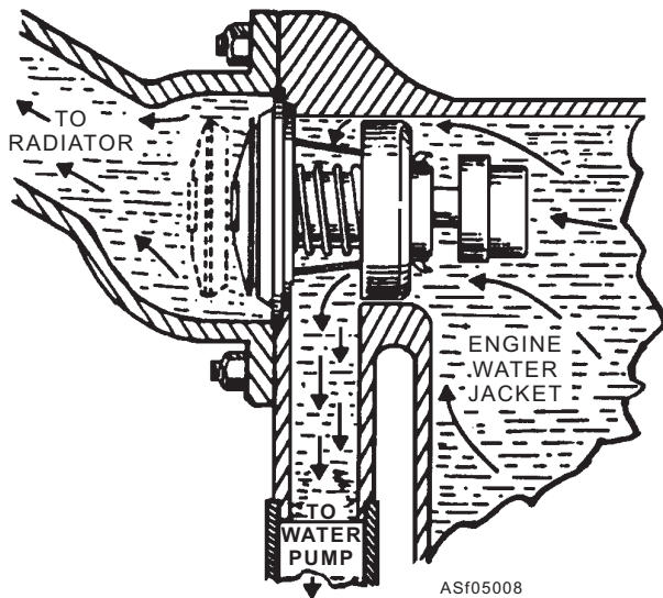
Figure 5-8.—Pellet thermostat.
