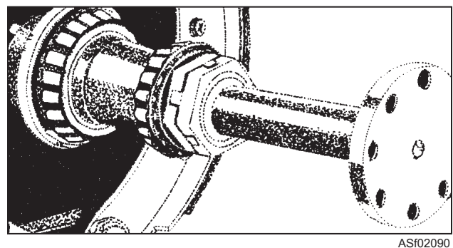
Figure 2-90.—Bearing mounting and adjustment nuts of full floating construction.
