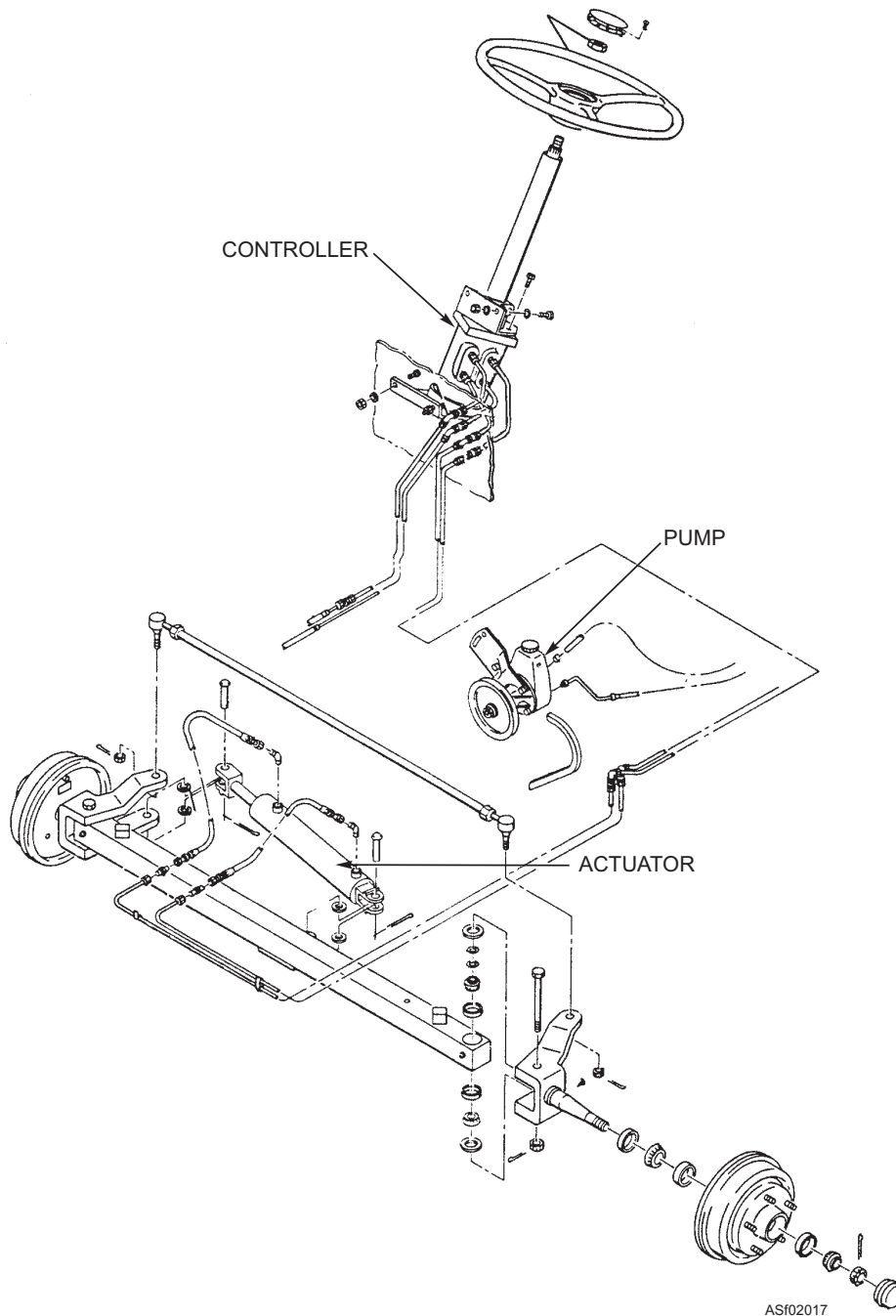
Figure 2-17.—Power steering system.
