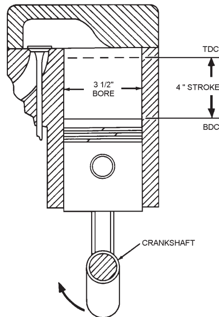
Figure 3-12.—Bore and stroke of an engine cylinder.
