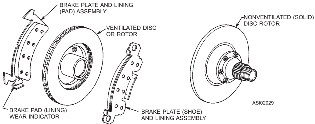
Figure 2-29.—Disc brake assembly.
