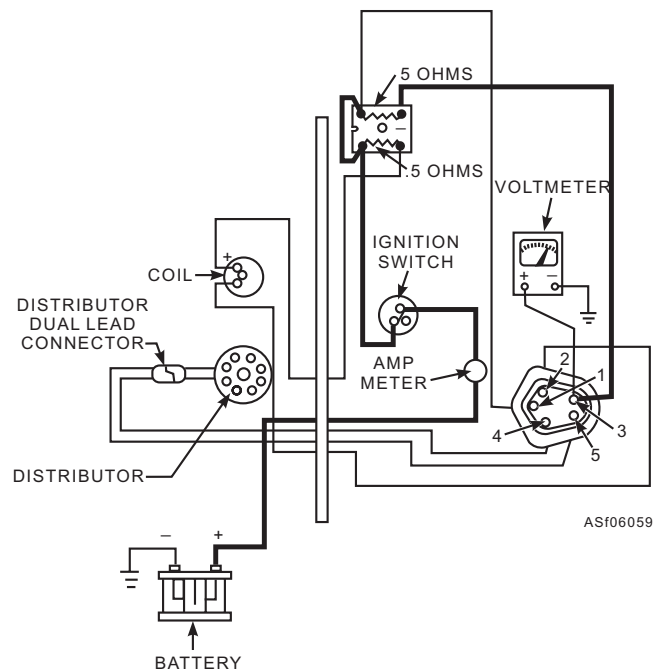
Figure 6-59.—Harness connector No. 3 test.
