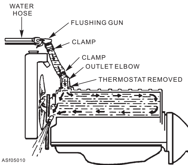
Figure 5-10.—Reverse flushing of water jackets.
