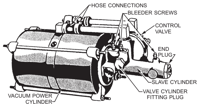
Figure 2-42.—Hydrovac vacuum power brake cylinder.
