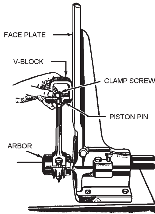
Figure 3-32.—Checking connecting rod alignment.
