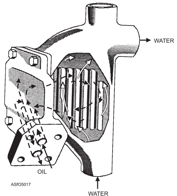
Figure 5-17.—Oil temperature regulator (cooler).
