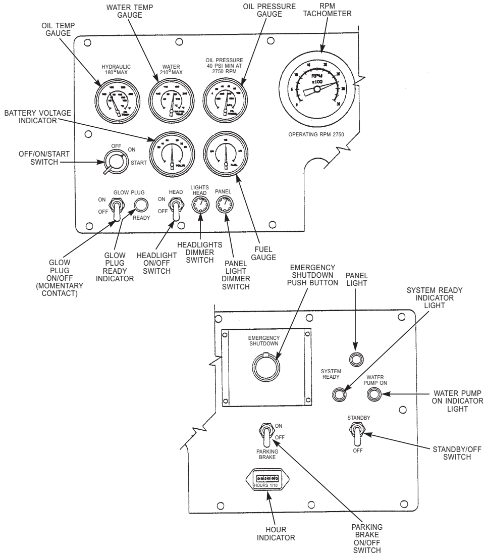
Figure 13-5.—Controls and indicators on the A/S32P-25 fire-fighting vehicle.
