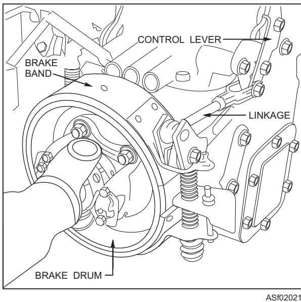
Figure 2-21.—External contracting transmission parking brake.
