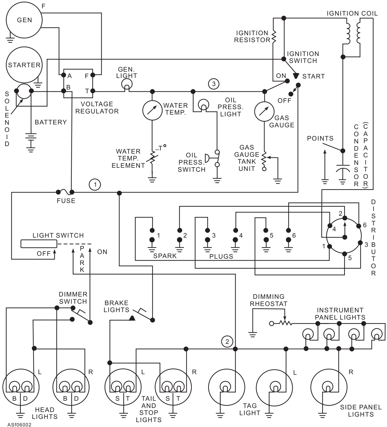
Figure 6-2.—Schematic diagram.
