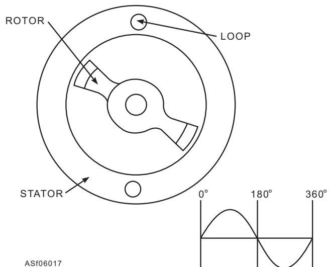
Figure 6-17.—A simple alternator.
