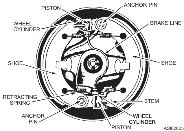
Figure 2-25.—Front wheel brake assembly.
