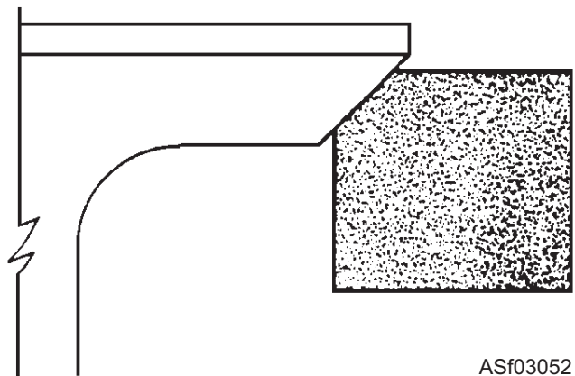
Figure 3-52.—Normal valve seat.
