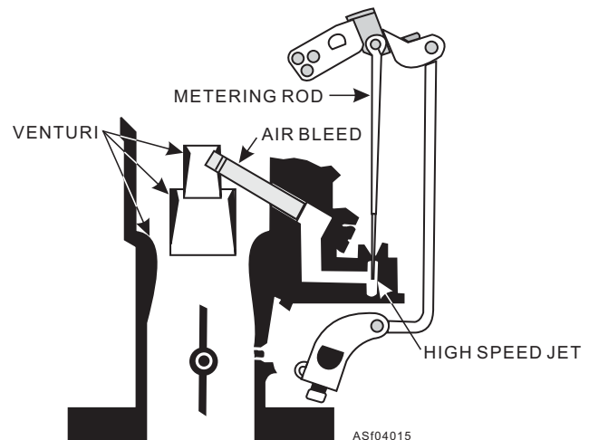
Figure 4-15.—Metering rod full load circuit.
