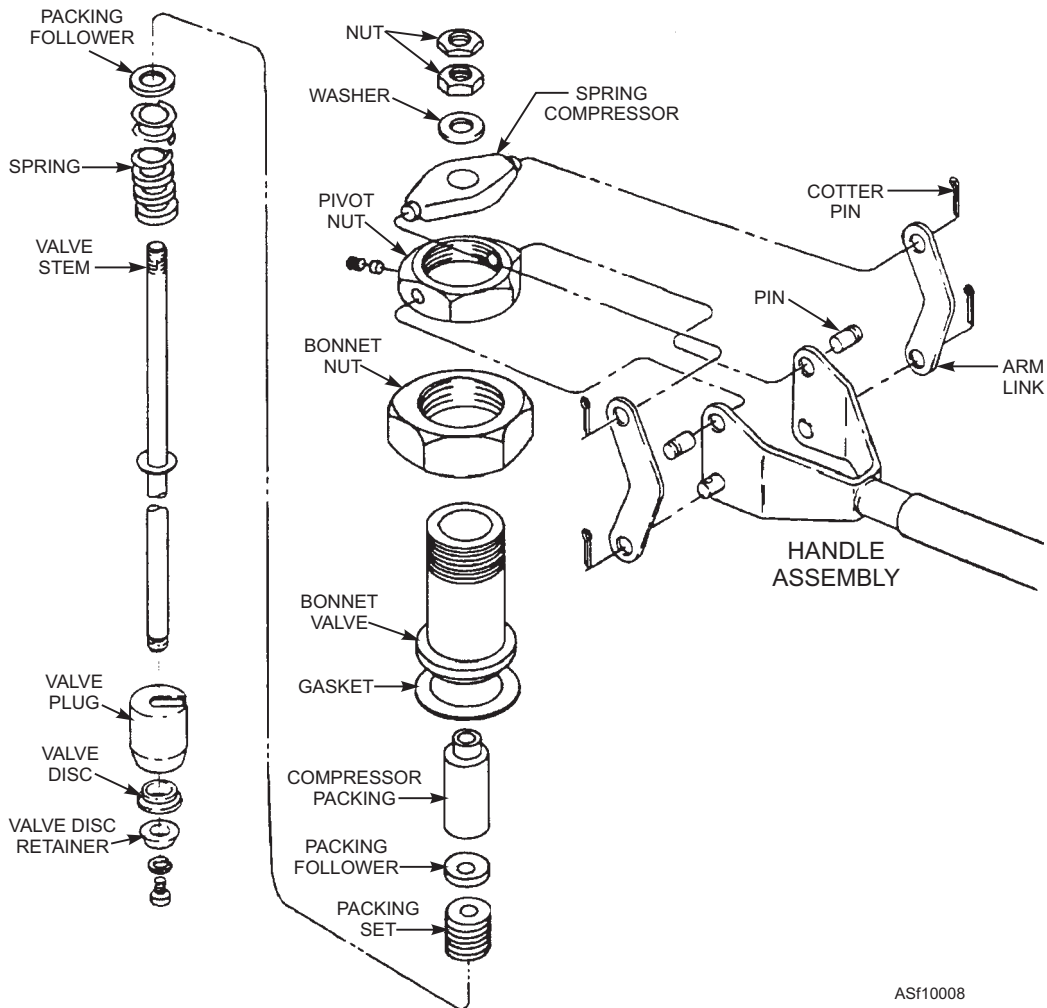
Figure 10-8.—Toggle valve assembly.
