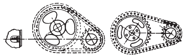
Figure 3-57.—Methods of valve timing with chain drive.
