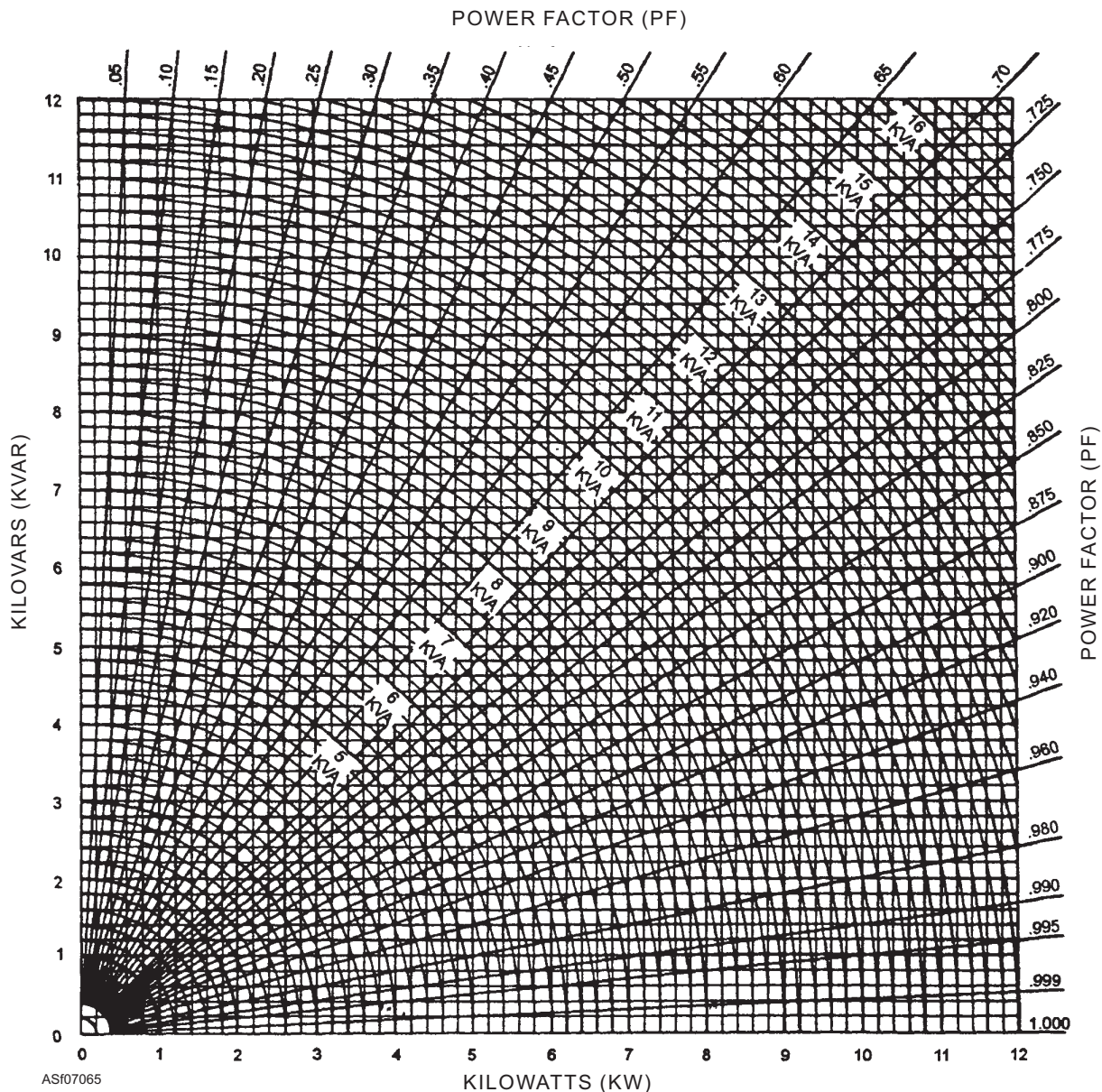
Figure 7-65.—Kilowatts (KW) chart.
