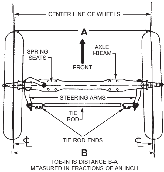
Figure 2-15.—Toe-in.
