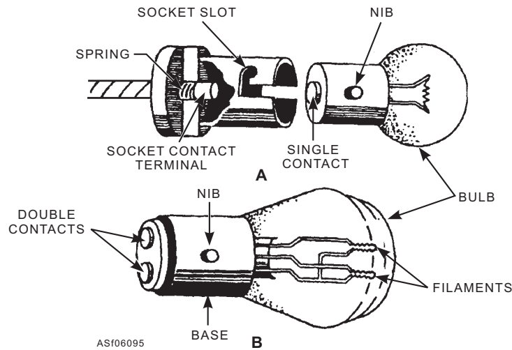
Figure 6-95.—Commonly used light bulbs.
