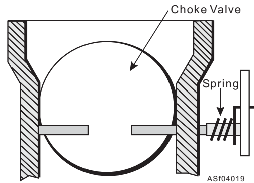
Figure 4-19.—Off-center choke valve.
