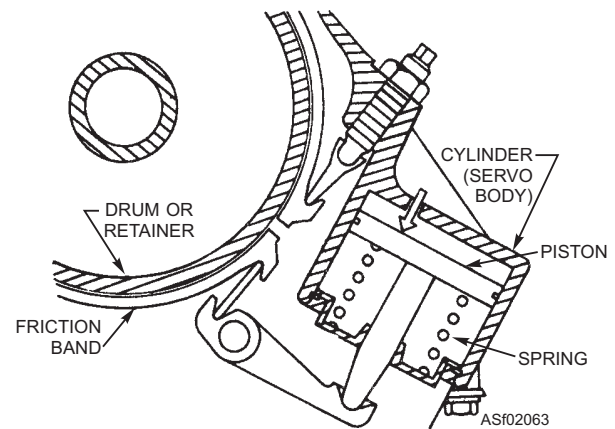
Figure 2-63.—Servo unit.
