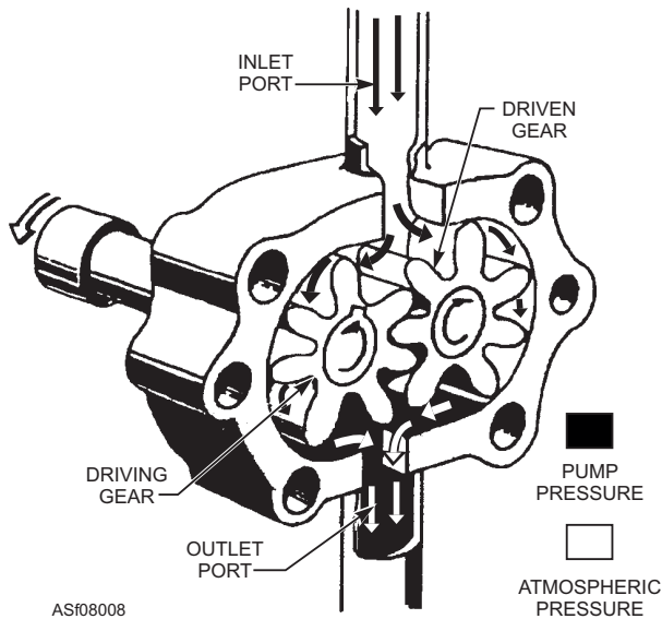
Figure 8-8.—Spur tooth pump.
