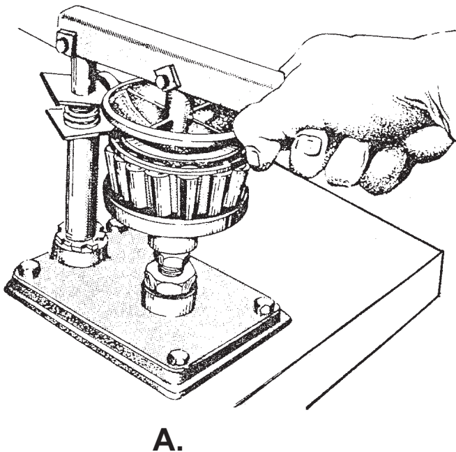
Figure 2-3.—Packing wheel bearings.
