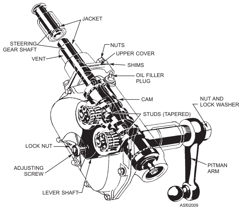
Figure 2-9.—Steering gear unit of the cam and lever type.
