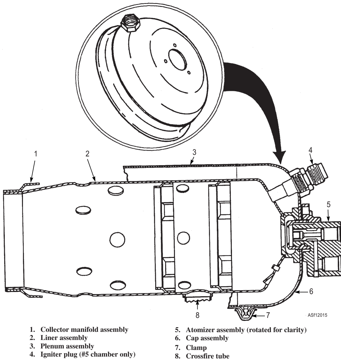
Figure 12-15.—Combustion chamber construction.
