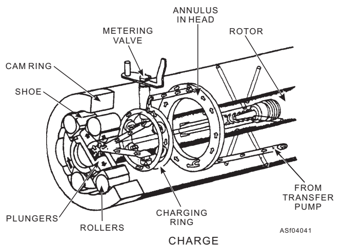
Figure 4-41.—Rotor in charging position with the rollers between the cam lobes (DC pump).
