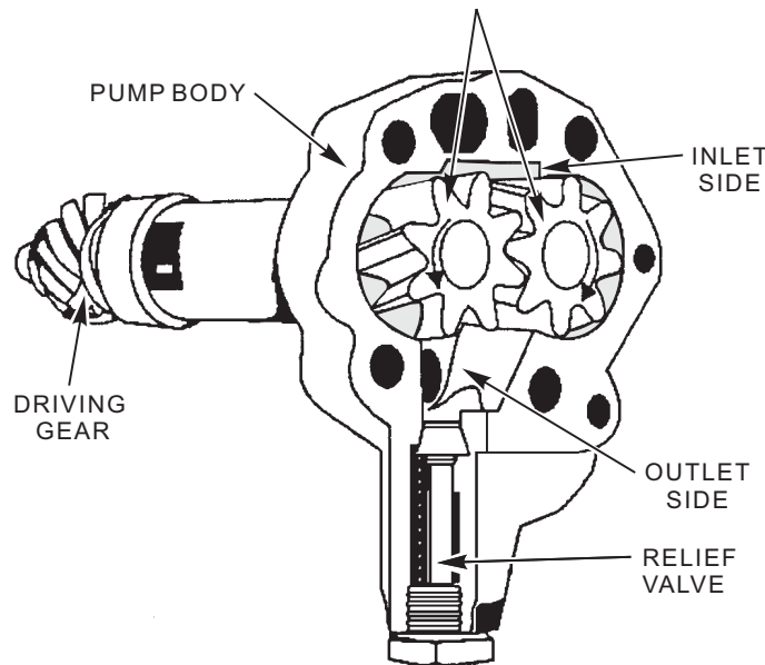
Figure 5-12.—Gear oil pump.
