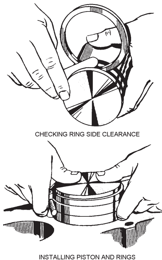
Figure 3-31.—Fitting piston ring and installing piston.
