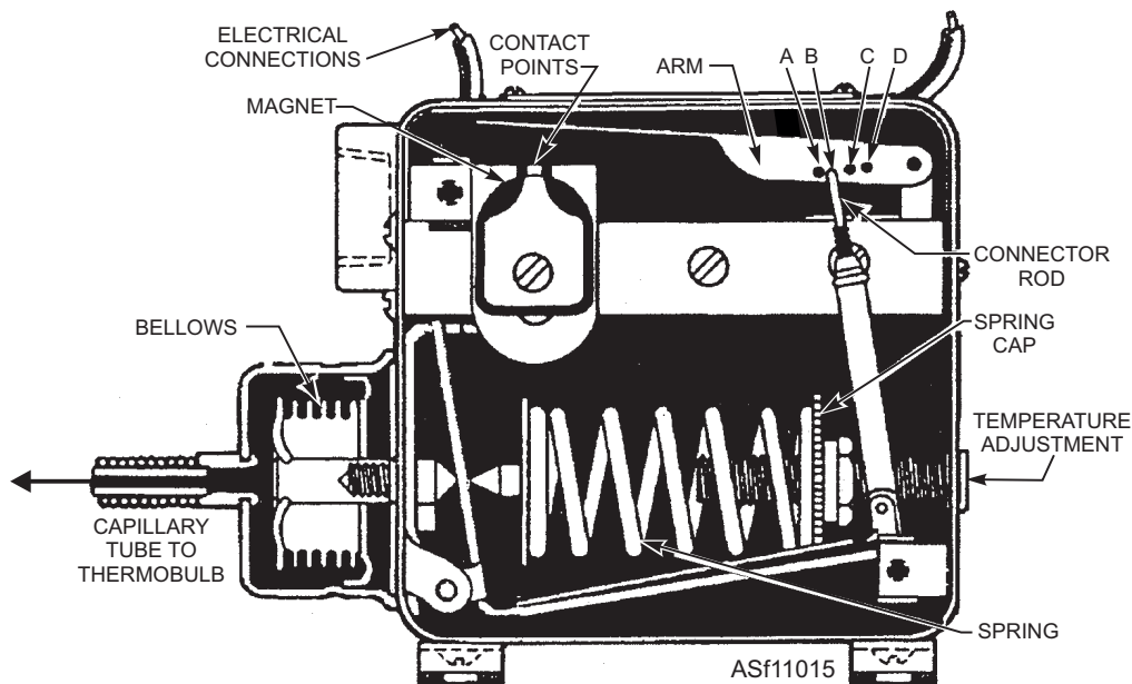
Figure 11-15.—Thermostat.
