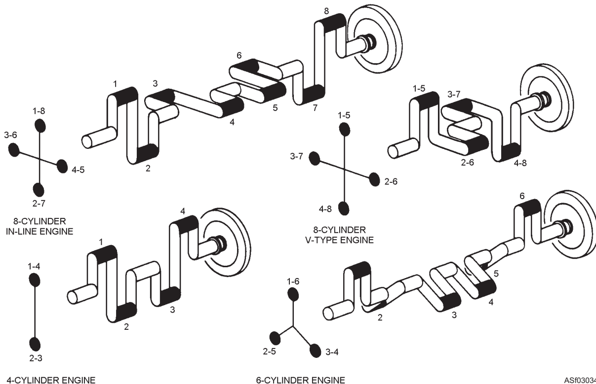
Figure 3-34.—Crankshaft and throw arrangements commonly used.
