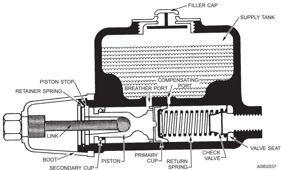
Figure 2-37.—Hydraulic brake master cylinder.
