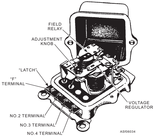
Figure 6-34.—Two-unit, vibrating-contact, ac regulator.
