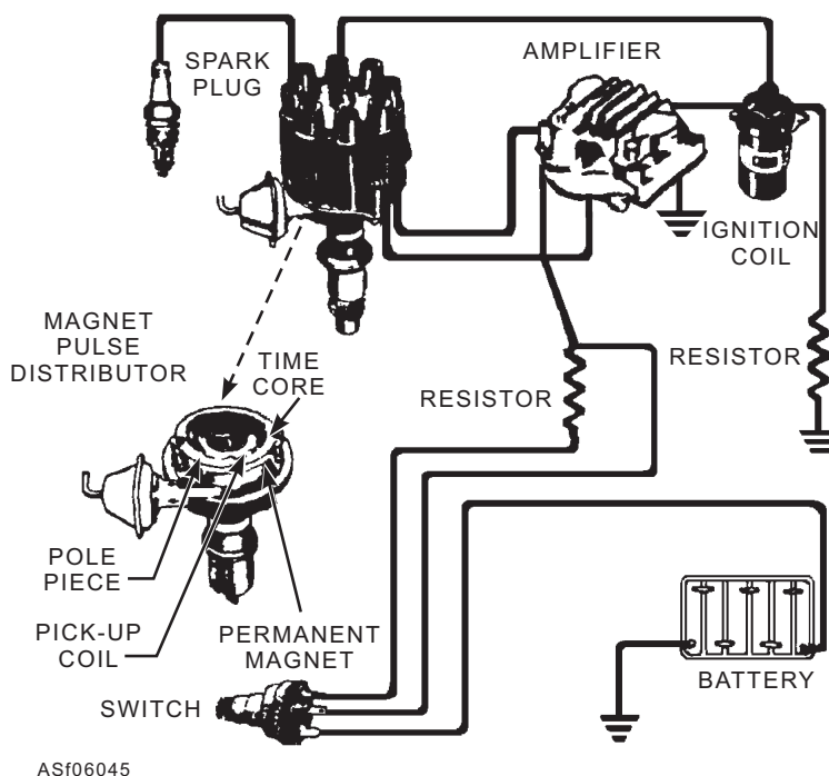
Figure 6-45.—Transistor controlled magnetic pulse battery ignition system.
