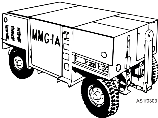
Figure 1-5.—MMG-1A mobile electric power plant.
