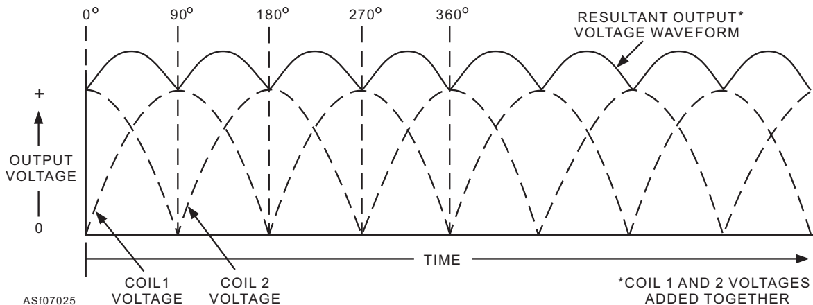
Figure 7-25.—Results of additional coil.
