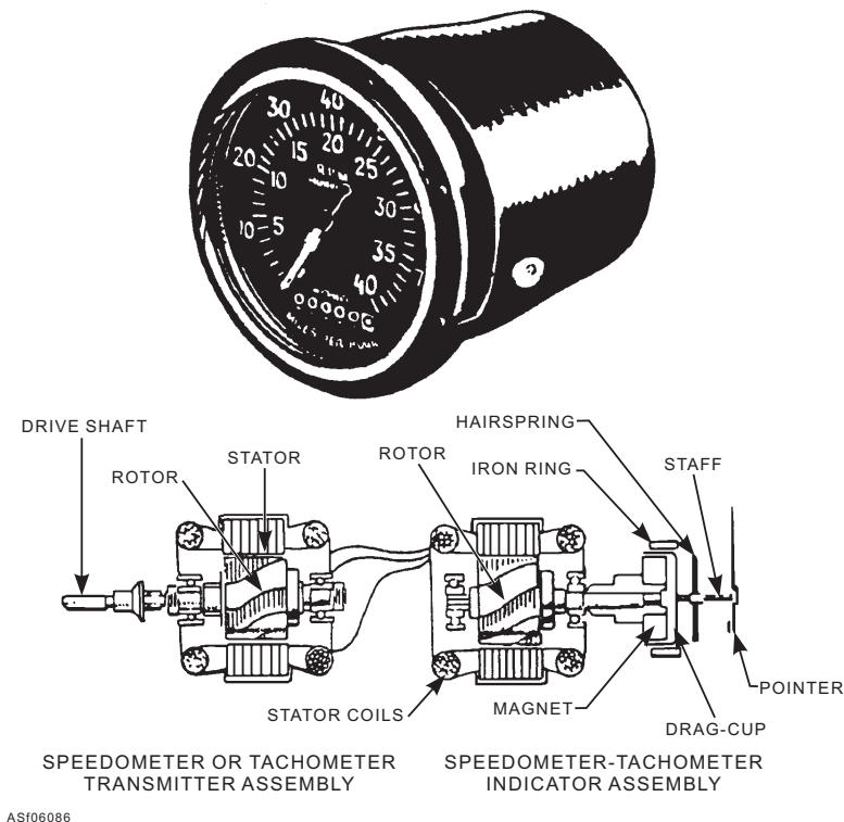
Figure 6-86.—Electrical speedometer-tachometer.
