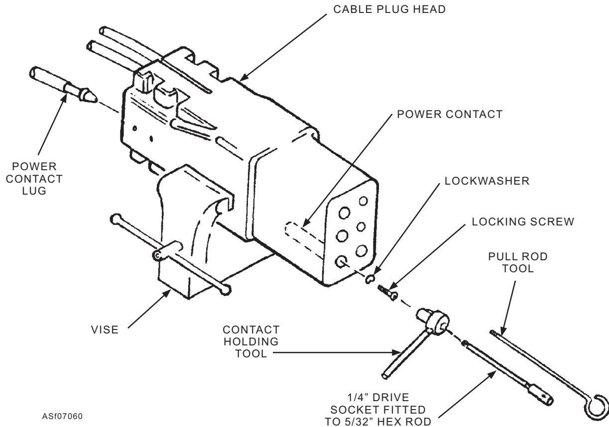
Figure 7-60.—Special tools.
