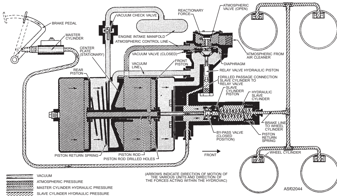
Figure 2-44.—Hydrovac operation—applied position.
