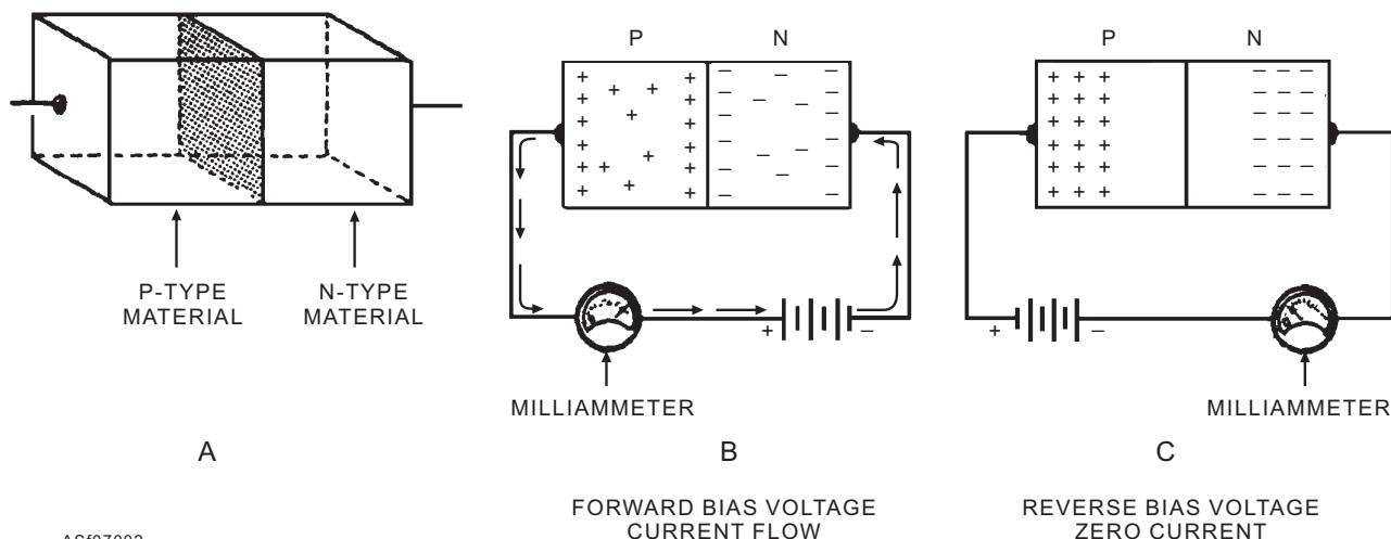
Figure 7-2.—Junction diode.
