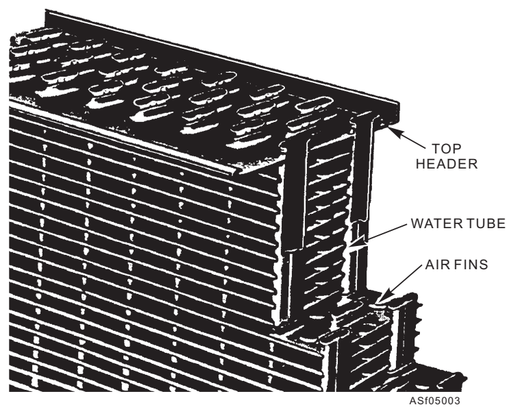
Figure 5-3.—Tubular radiator core construction.
