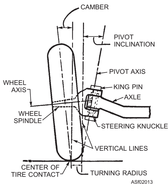
Figure 2-13.—Pivot inclination and camber.
