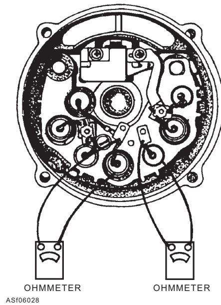
Figure 6-28.—Testing diodes with an ohmmeter.
