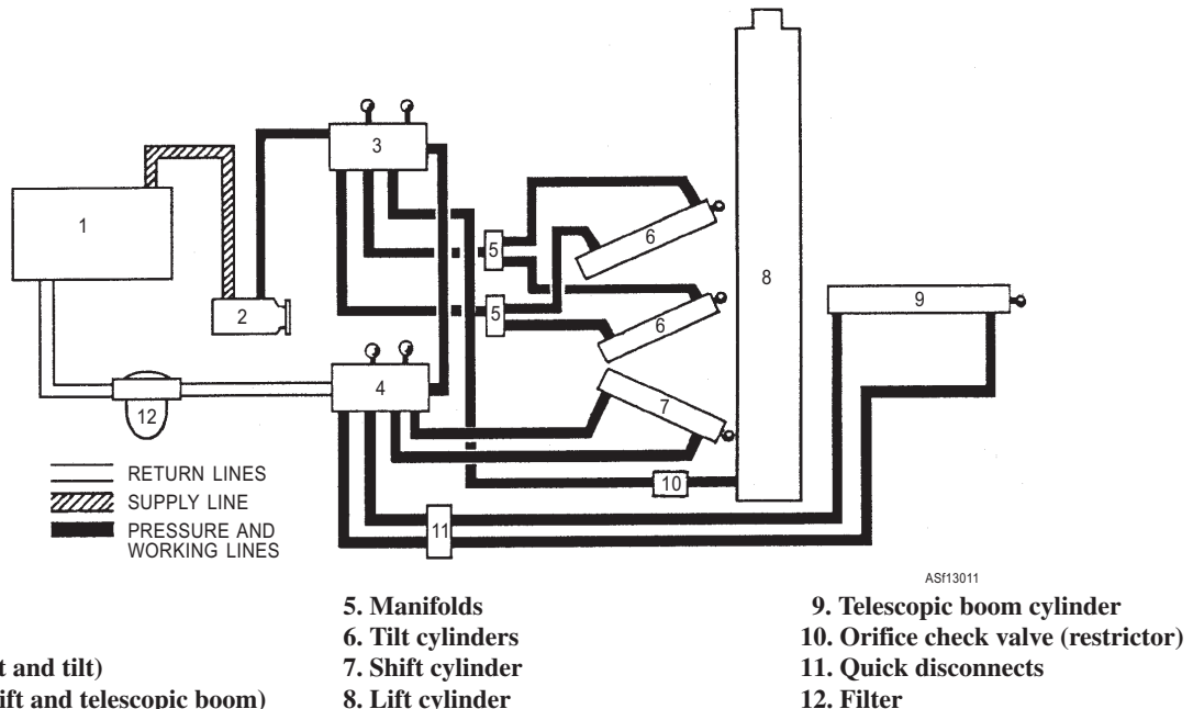
Figure 13-11.—Schematic of a typical forklift hydraulic system.
