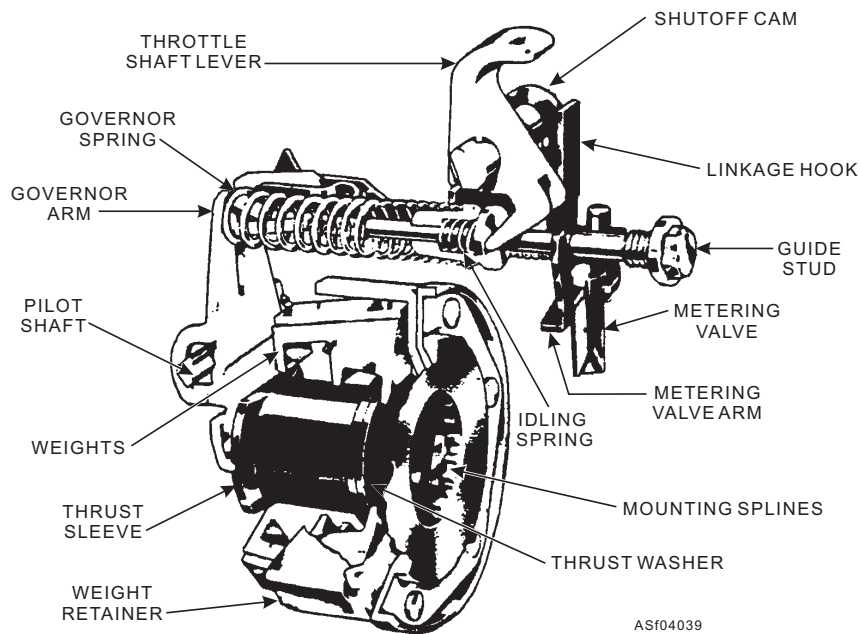
Figure 4-39.—Governor assembly (Model DC).
