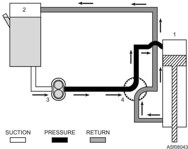
Figure 8-43.—Simple hydraulic system.
