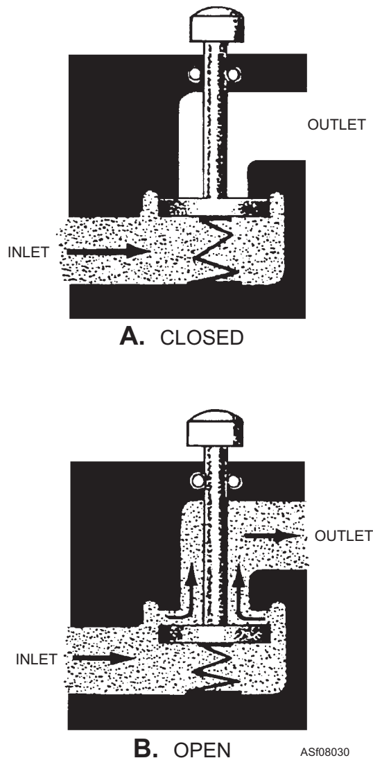
Figure 8-30.—Operation of a simple poppet valve.
