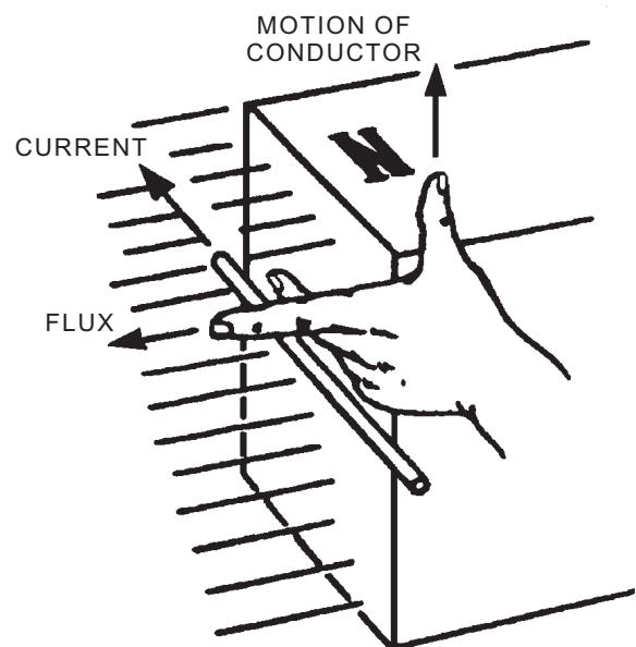
Figure 7-21.—Left-hand rule for generators.
