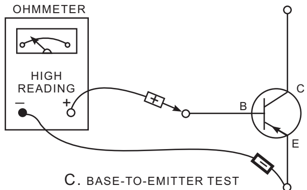
Figure 7-12.—Testing a transistor's leakage with an ohmmeter.
