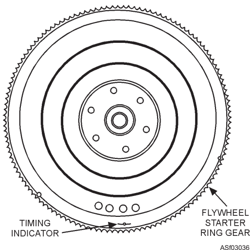
Figure 3-36.—Flywheel.
