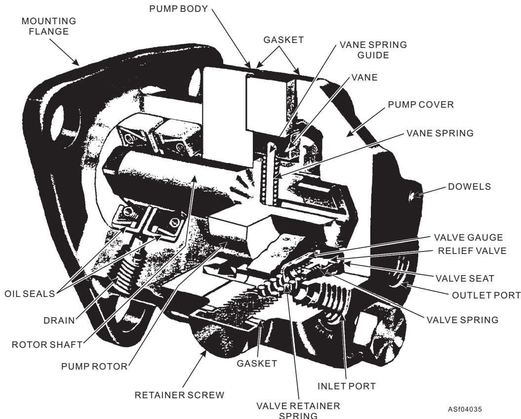
Figure 4-35.—Cutaway view of vane-type fuel pump.
