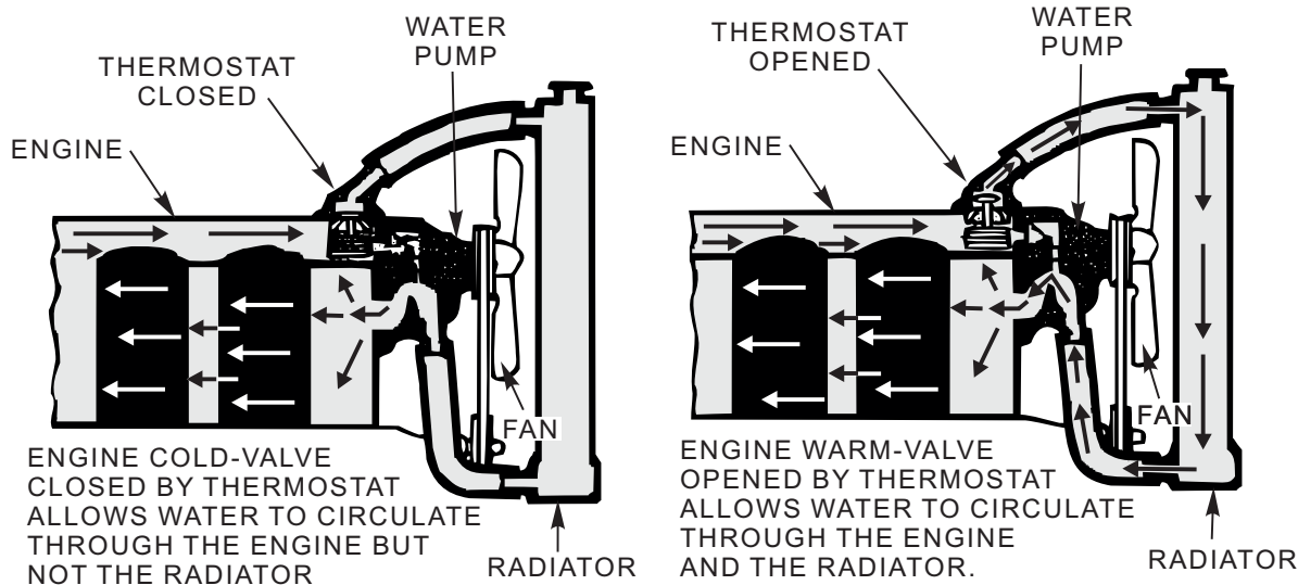
Figure 5-6.—A thermostat in operation.
