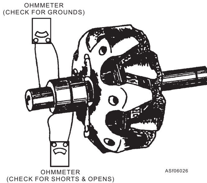
Figure 6-26.—Testing the rotor for grounds, shorts, and opens.
