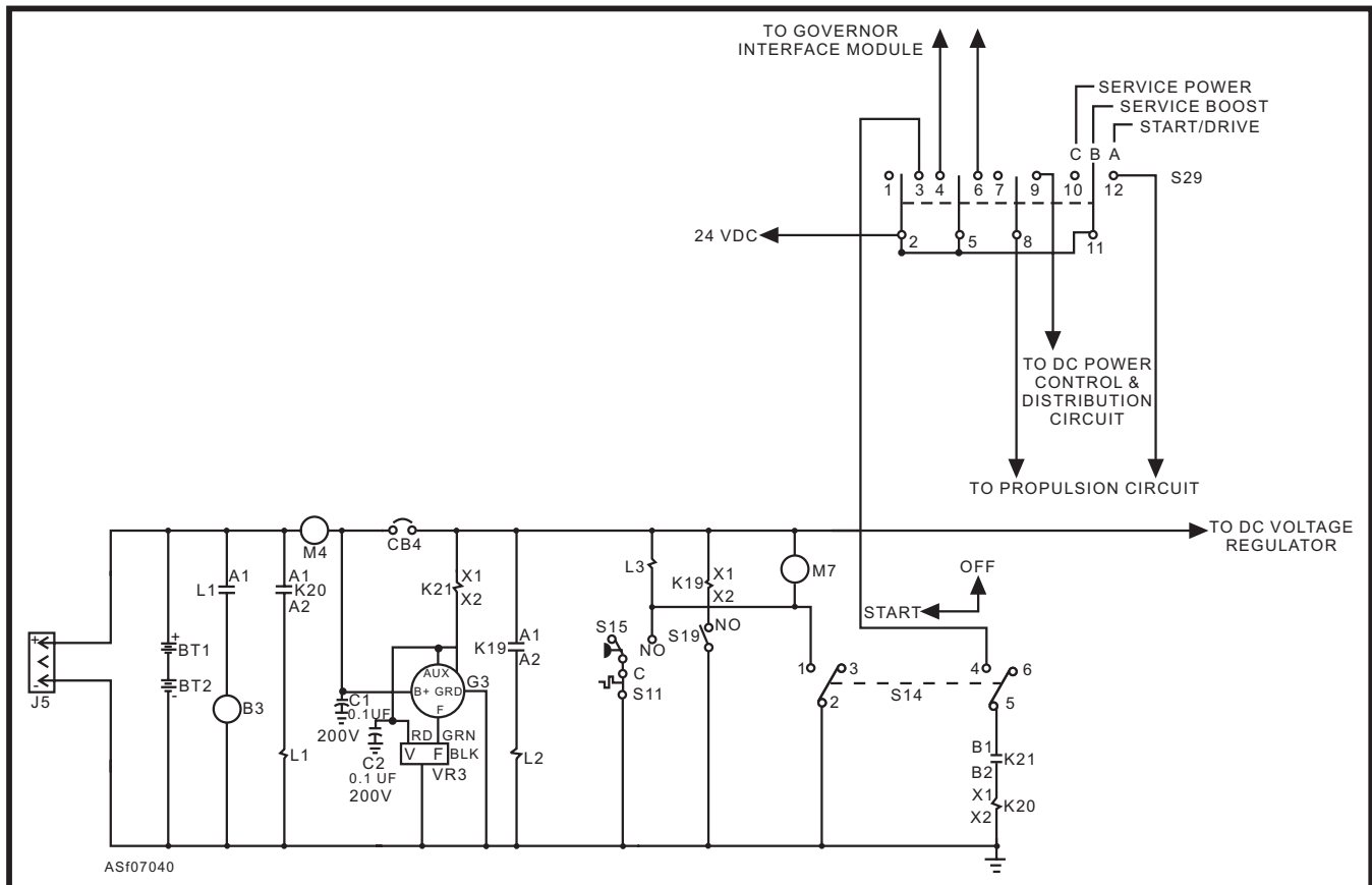
Figure 7-40.—Engine starting circuit.
