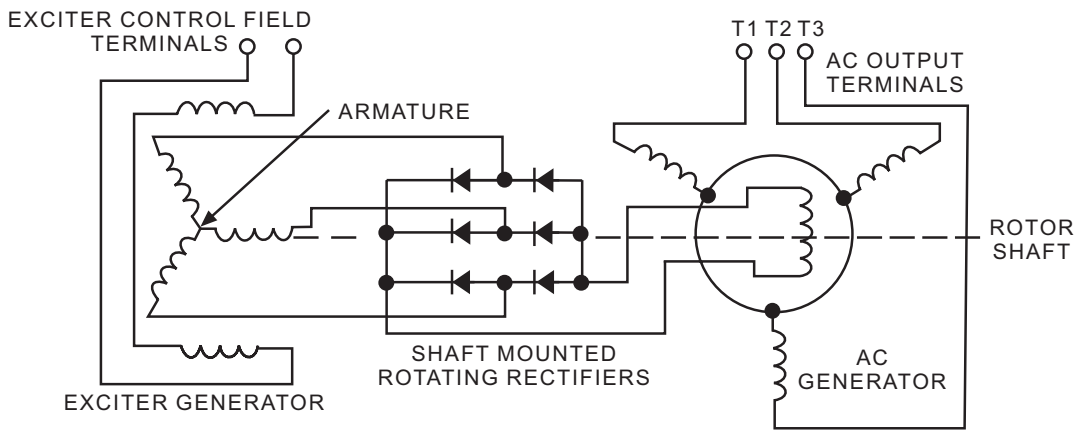
B BRUSHLESS GENERATOR (SCHEMATIC)
