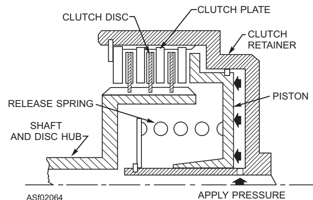
Figure 2-64.—Multiple disc clutch unit.
