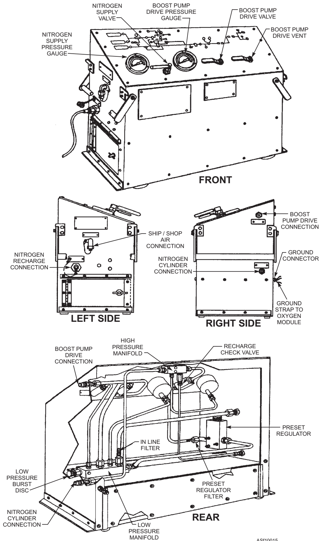
Figure 10-15.—Nitrogen module.
