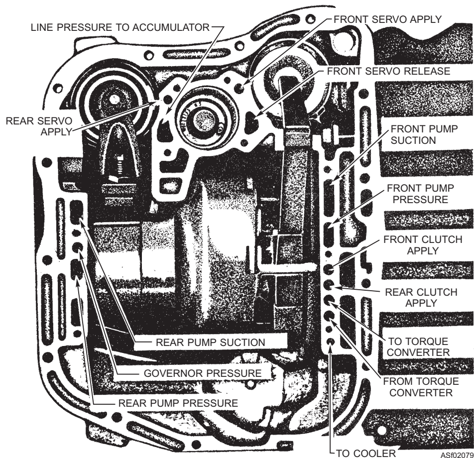
Figure 2-79.—Typical transmission oil passages.
