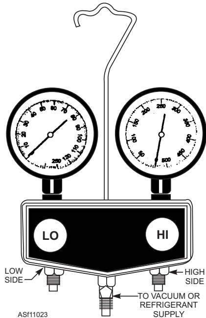
Figure 11-23.—Refrigerant manifold test set.
