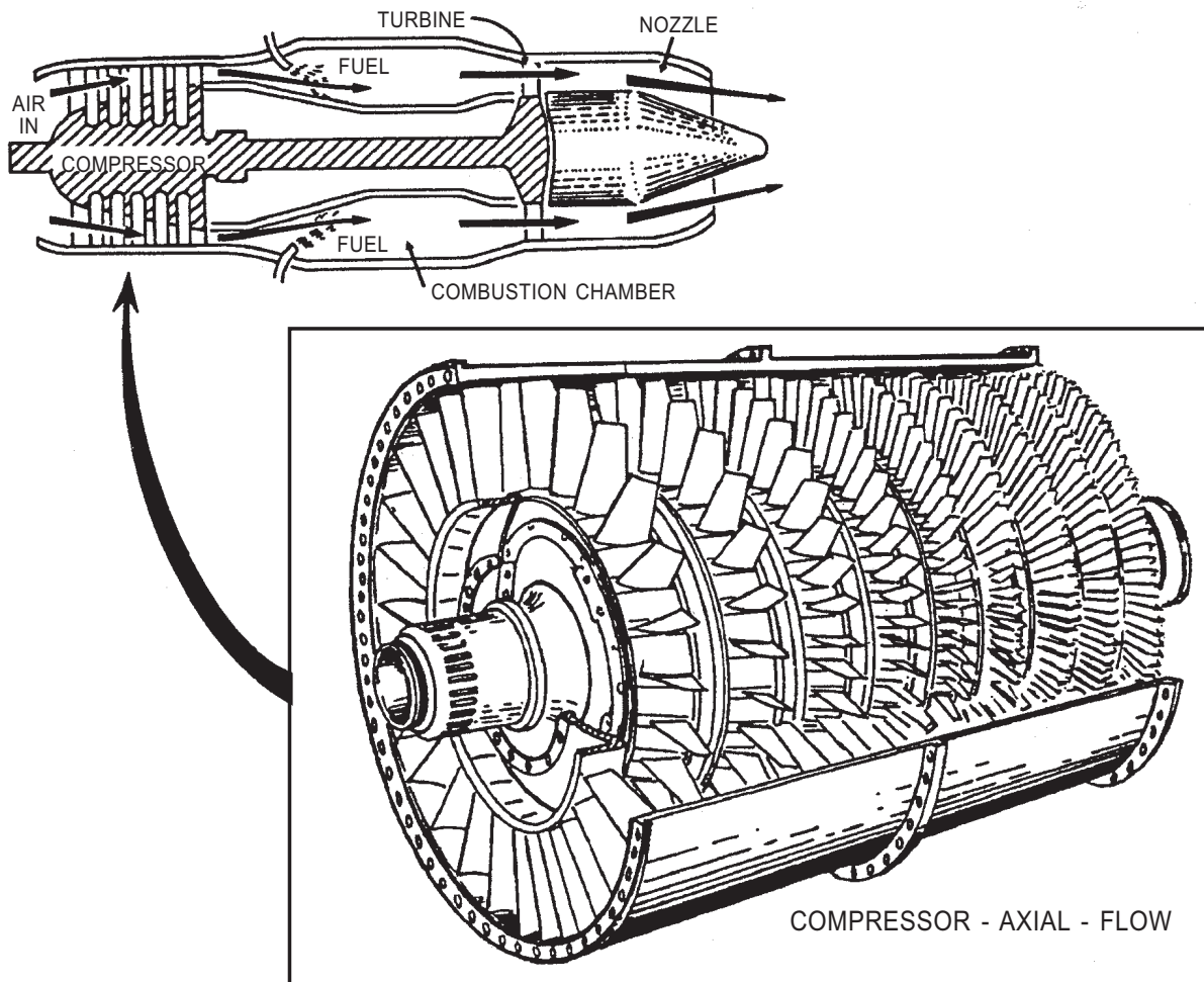
Figure 12-2.—Axial-flow type engine.
