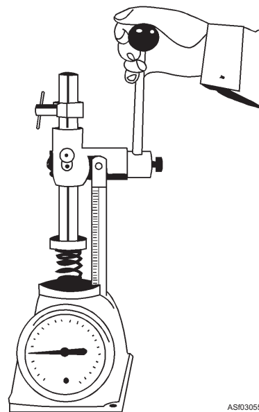
Figure 3-55.—Valve spring tester.
