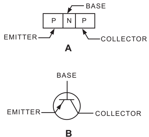
ASf07008 Figure 7-8.—PNP transistor—(A) PNP diagram; (B) schematic symbol.
