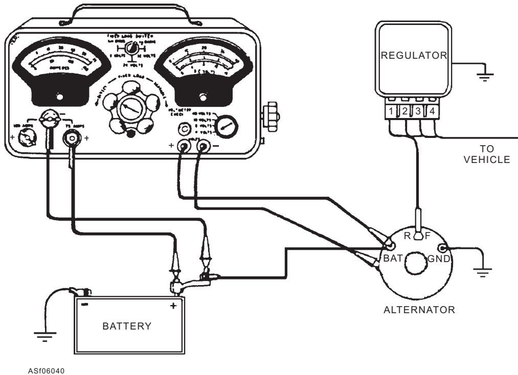
Figure 6-40.—Voltage regulator test.
