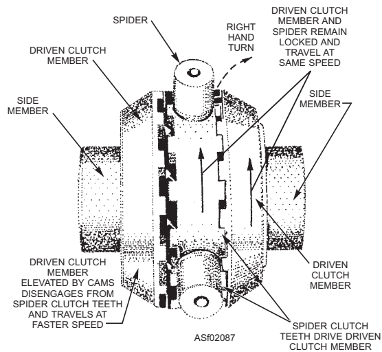
Figure 2-87.—Operation of a no-spin differential during a turn.
