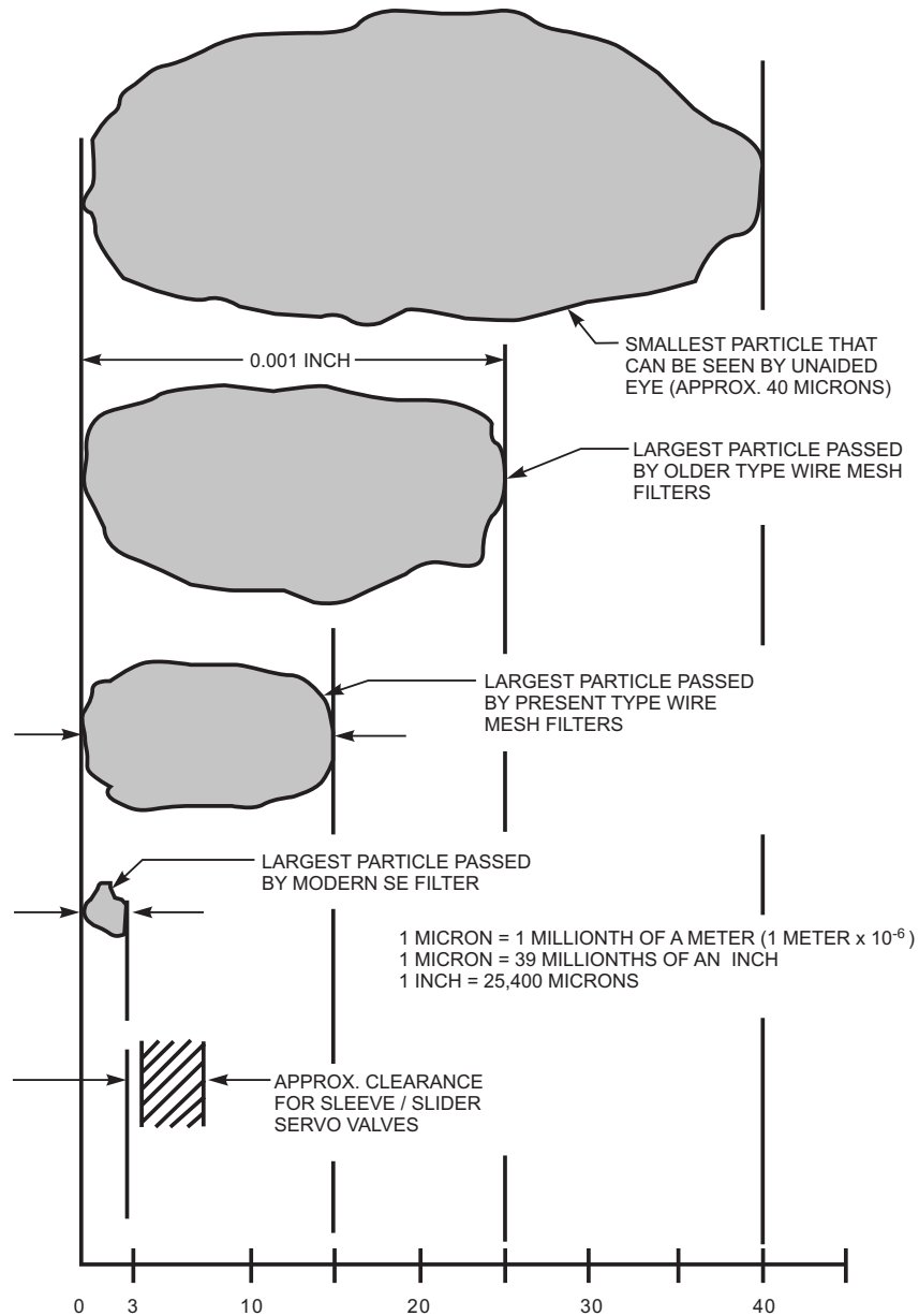
Figure 8-20.—Graphic comparison of particle sizes.
