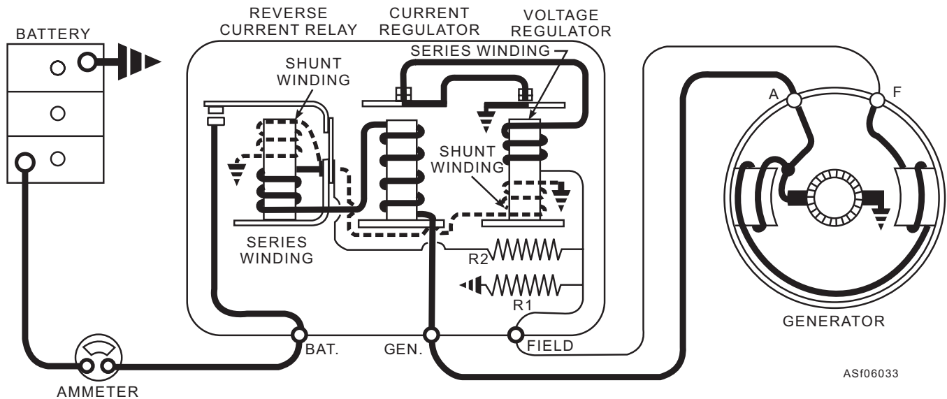
Figure 6-33.—Dc charging circuit with a vibrating-contact regulator.
