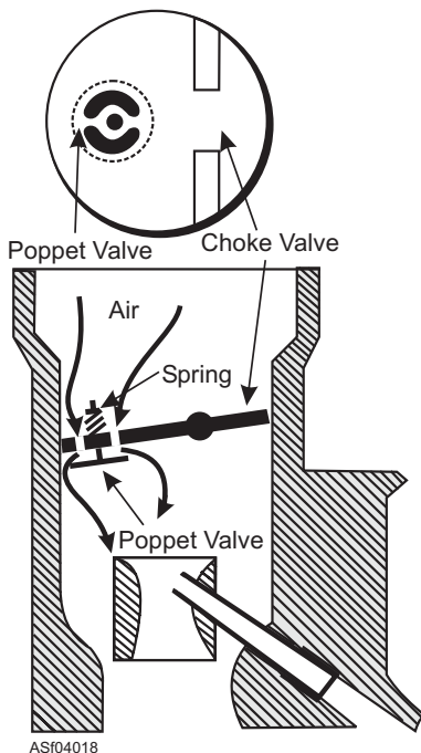
Figure 4-18.—Spring-loaded poppet valve in choke valve.
