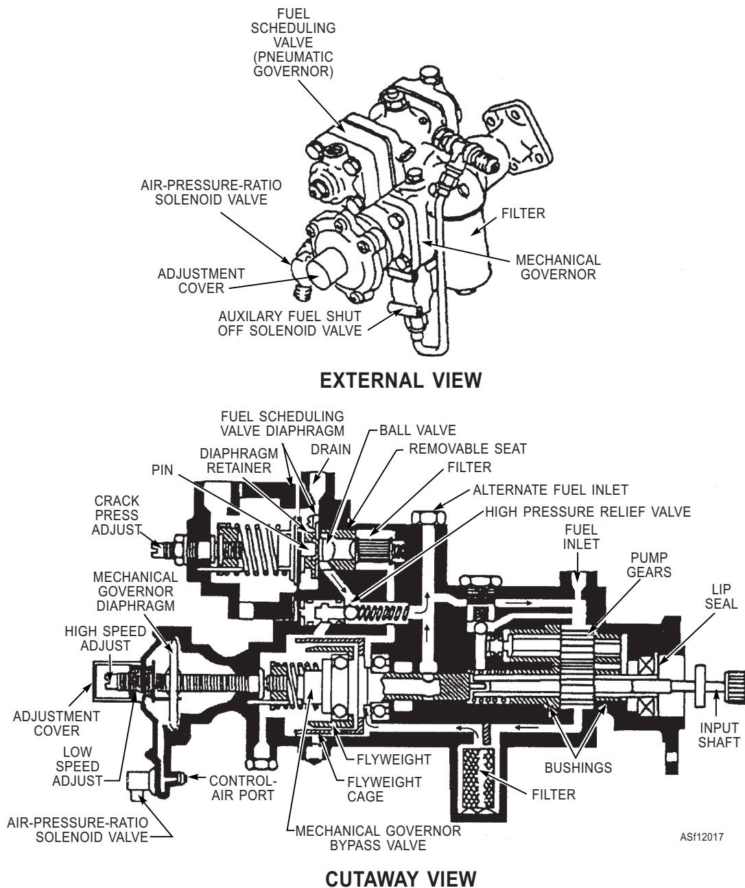
Figure 12-17.—Fuel control assembly.
