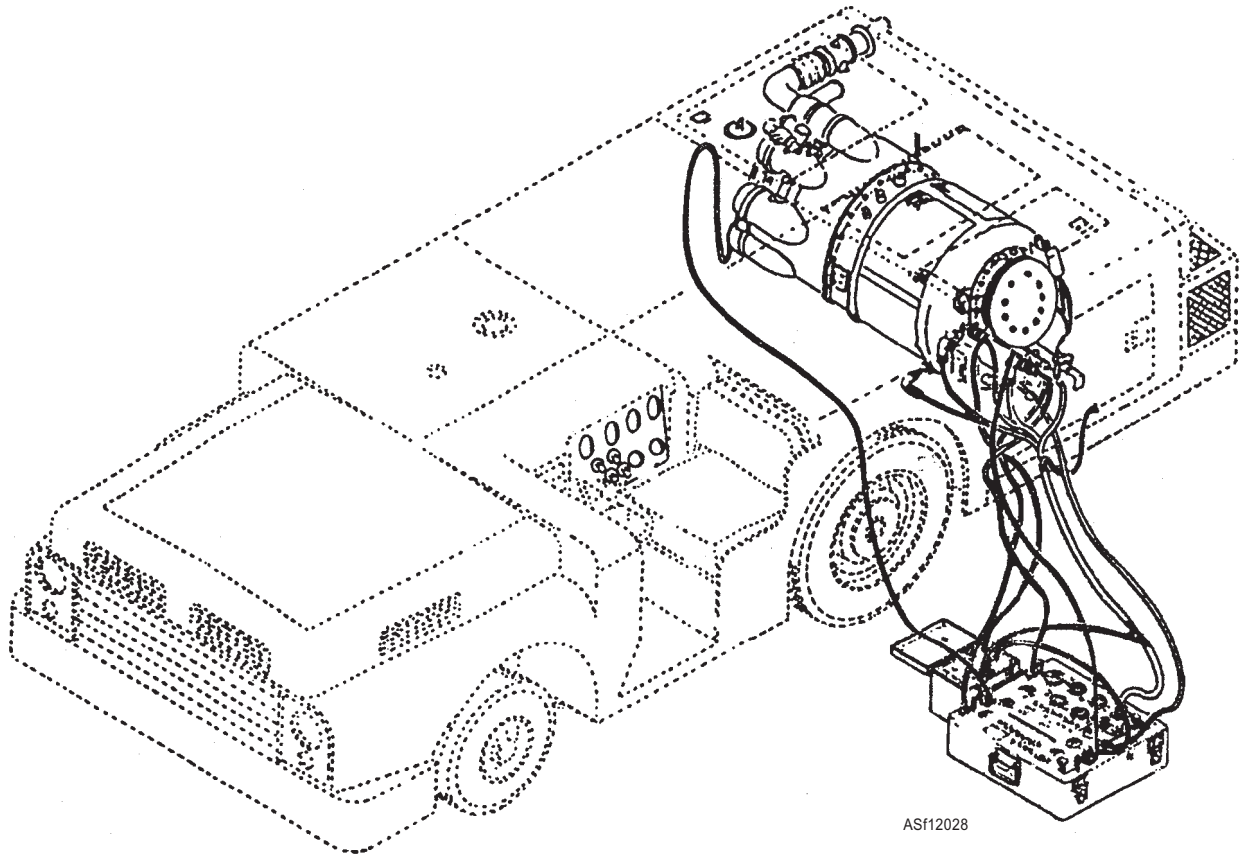
Figure 12-28.—Analyzer connected to engine while in its enclosure.
