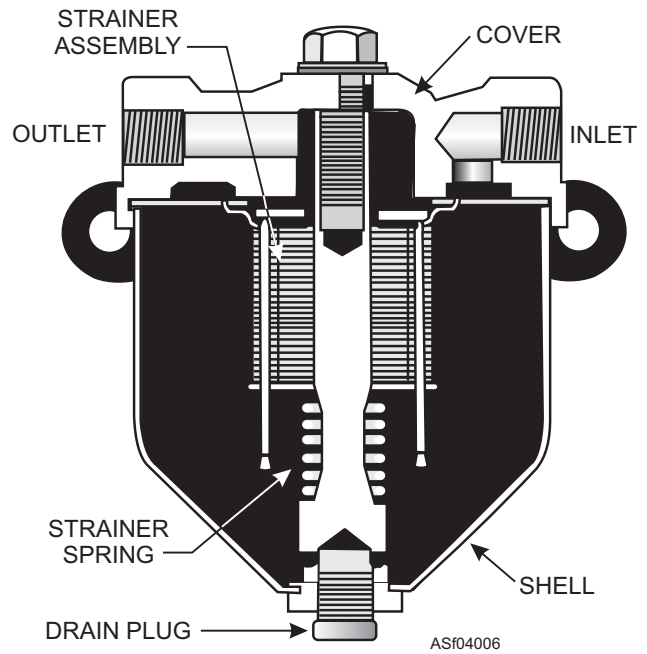
Figure 4-6.—Fuel filter.
