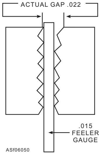
Figure 6-50.—False setting given by feeler gauge for used points.
