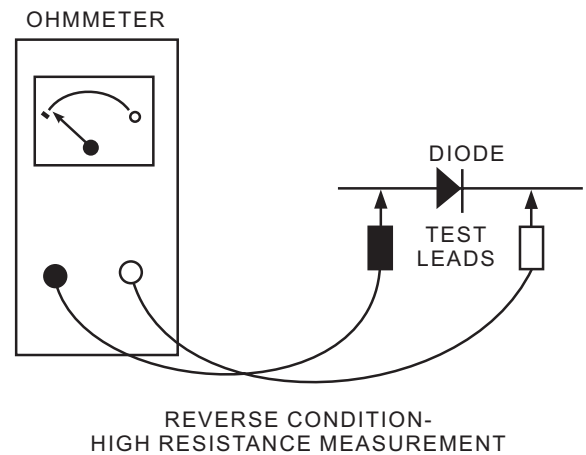
Figure 7-4.—PN diode identification.
