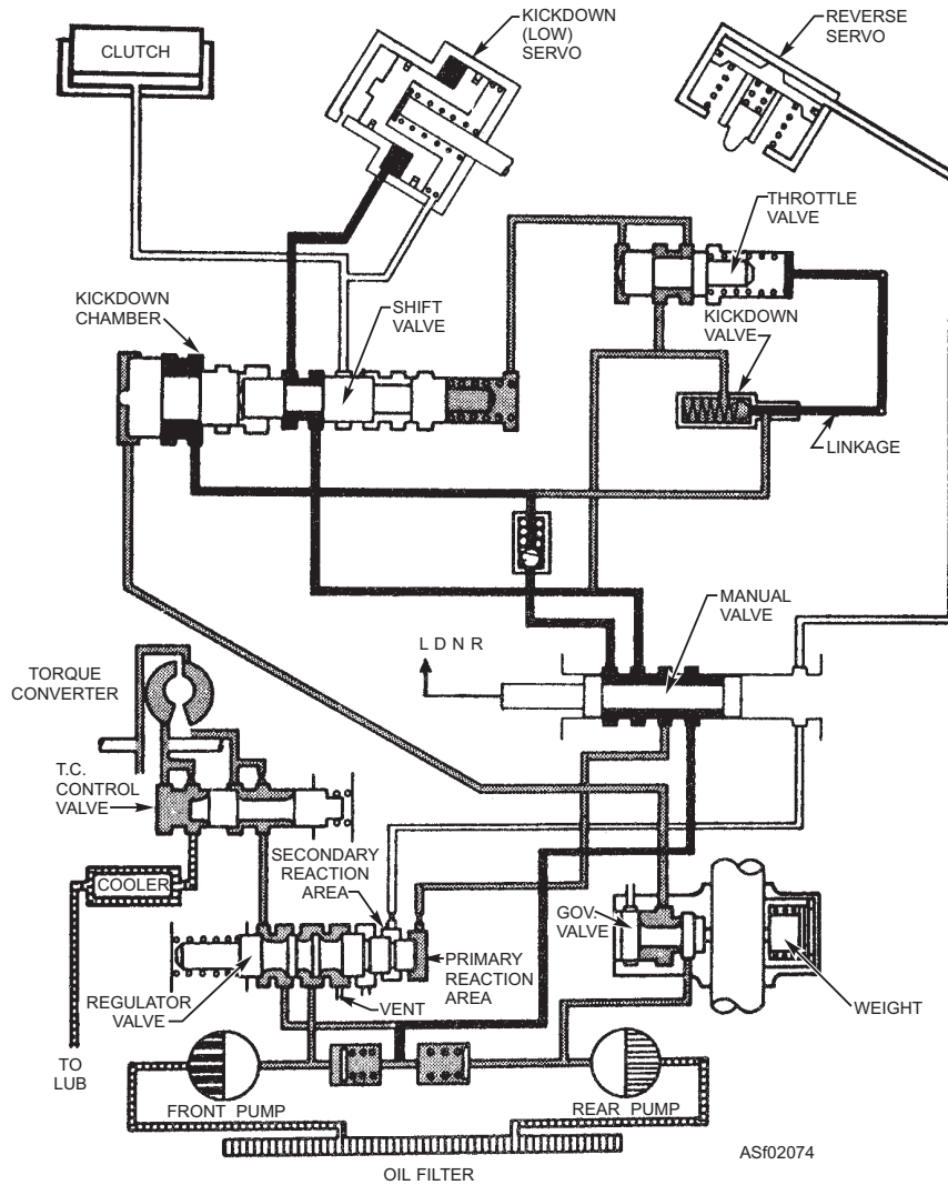
Figure 2-74.—Low (L) operating range.
