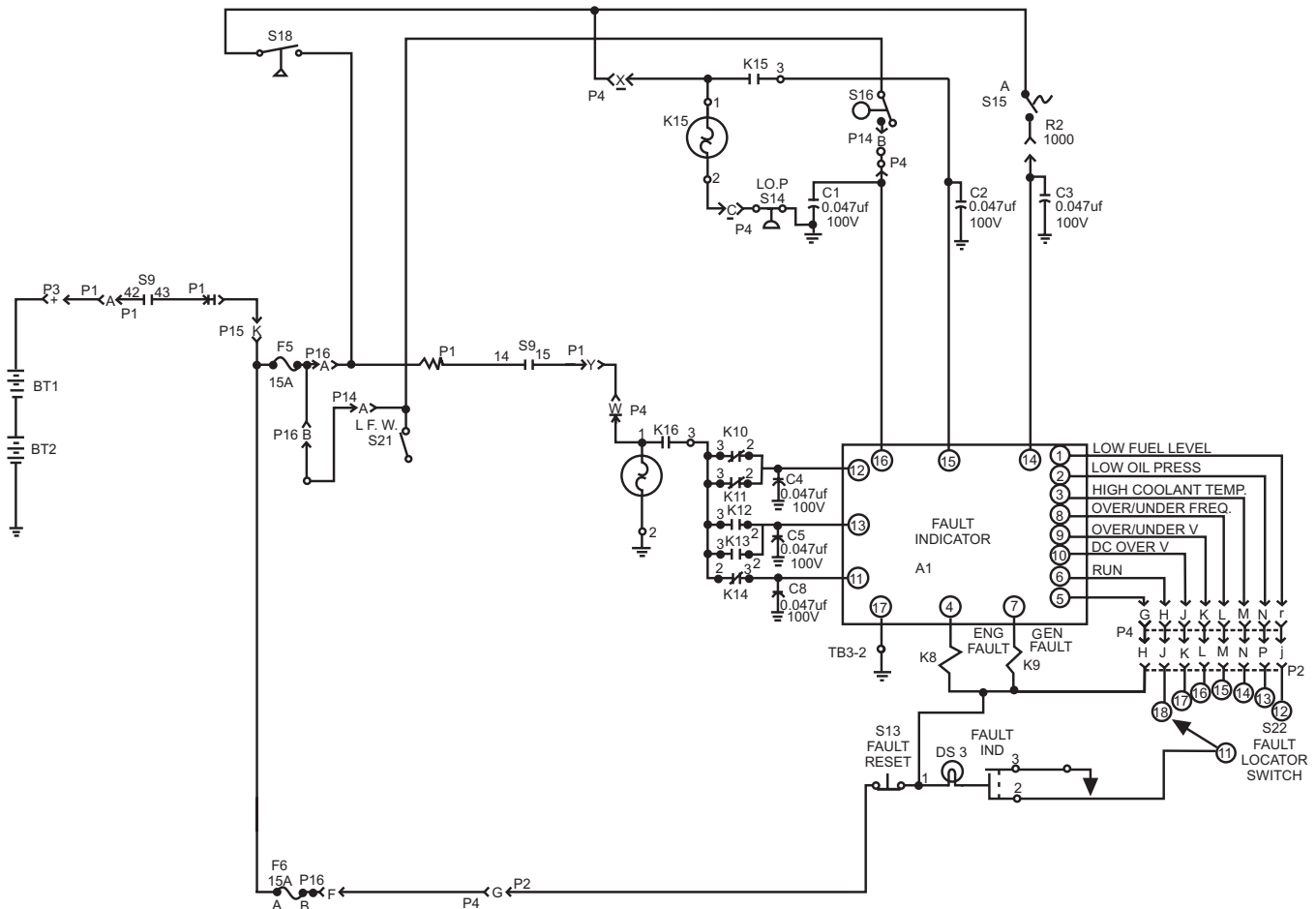
Figure 7-52.—Simplified schematic for fault locator switch.
