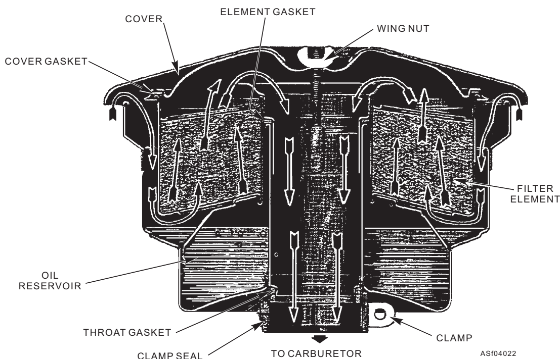
Figure 4-22.—Wet-type air cleaner.
