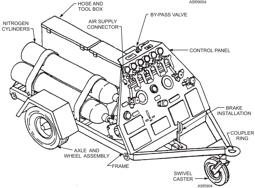
Figure 9-4.—A/M26U-4 (NAN-4) nitrogen servicing unit.
