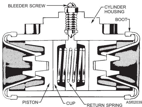
Figure 2-39.—Hydraulic brake wheel cylinder.
