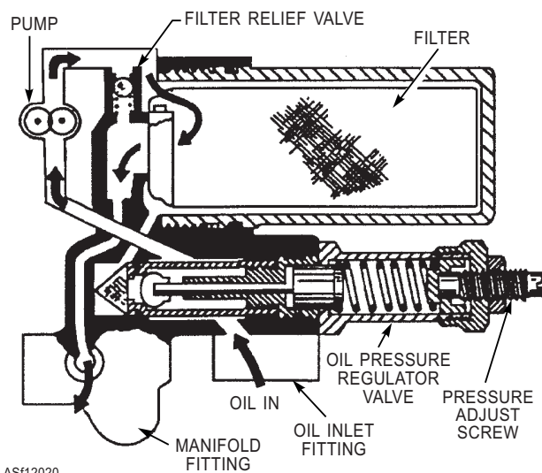
OIL PUMP SCHEMATIC
