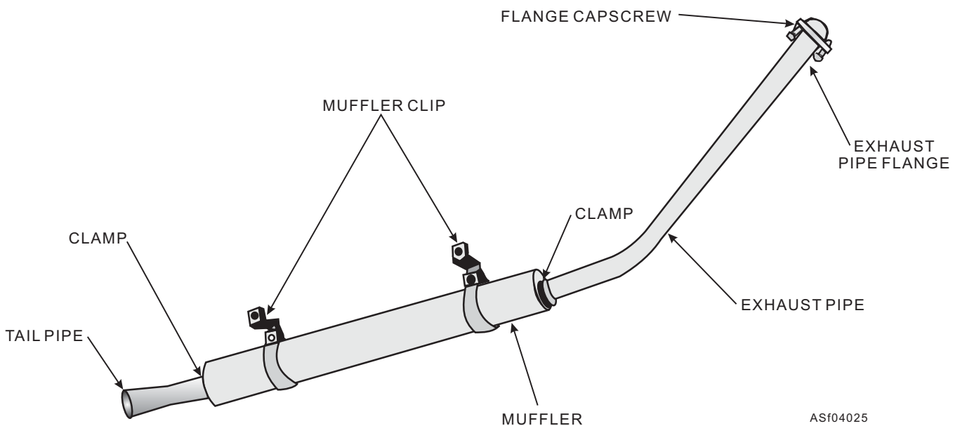
Figure 4-25.—Exhaust pipe, muffler, and tail pipe.
