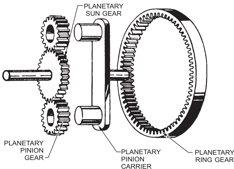
Figure 2-59.—Members of a simple planetary gear system.
