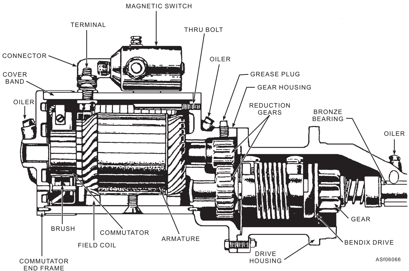
Figure 6-66.—Sectional view of a heavy-duty starter.
