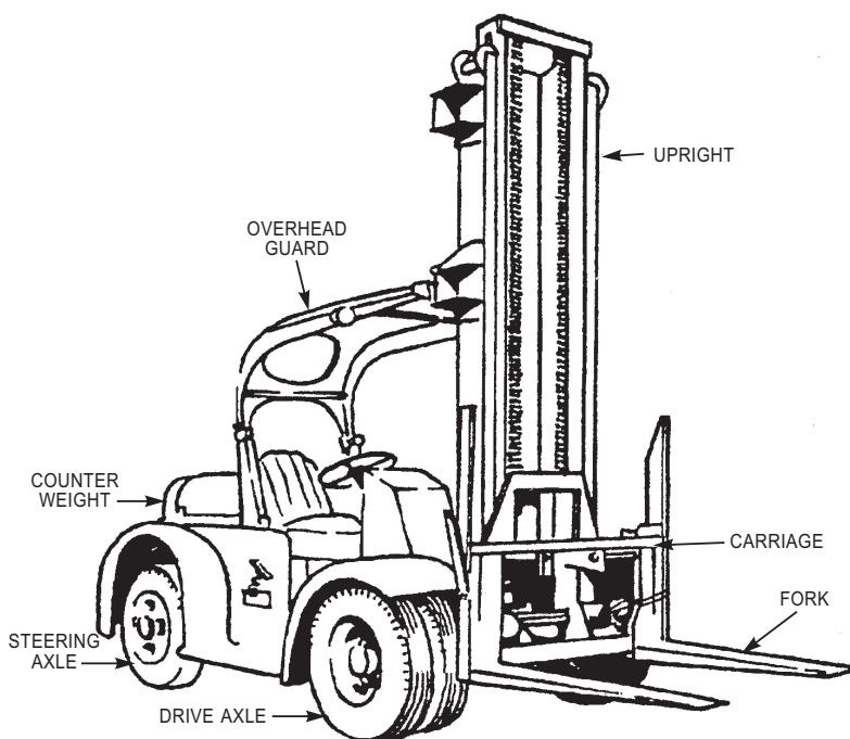
Figure 13-10.—A typical forklift.
