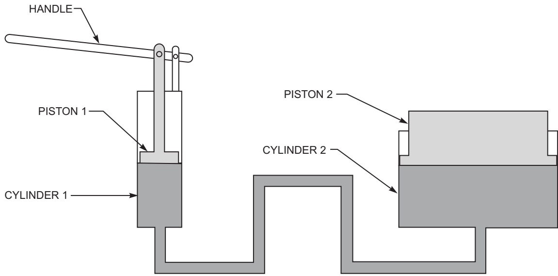
Figure 8-1.—Transmission of force by liquids.
