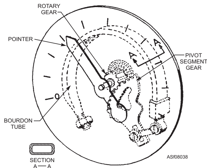
Figure 8-38.—Bourdon tube.
