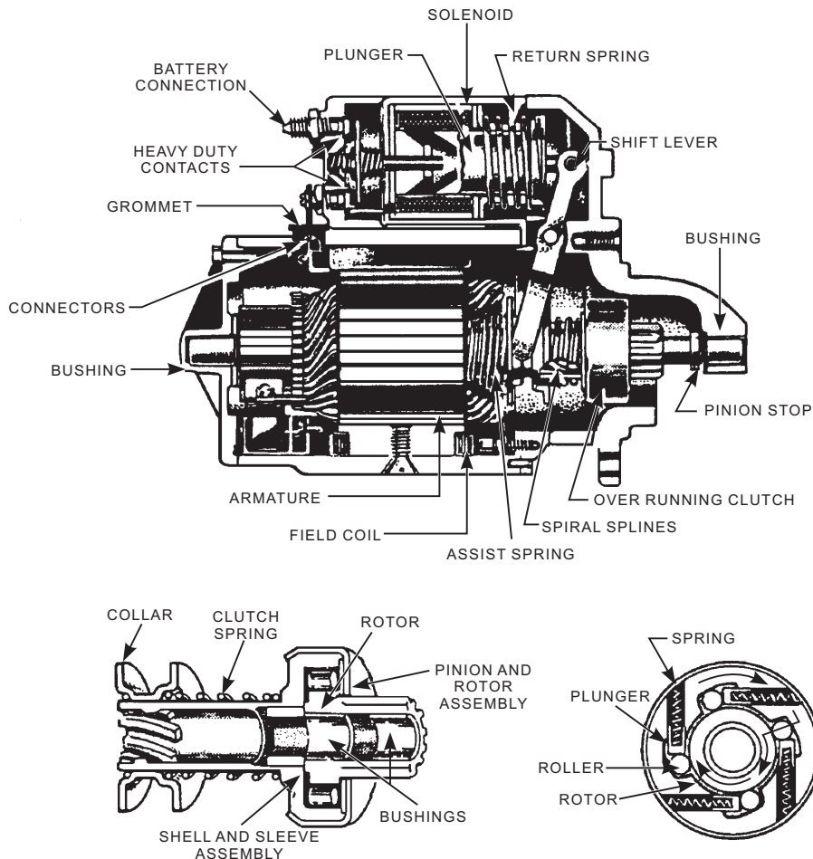
Figure 6-68.—Solenoid shift starter and overrunning clutch drive.
