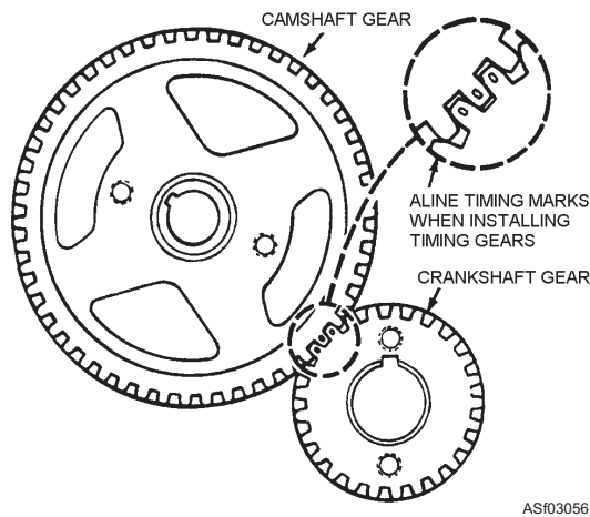
Figure 3-56.—Timing gears and their markings.
