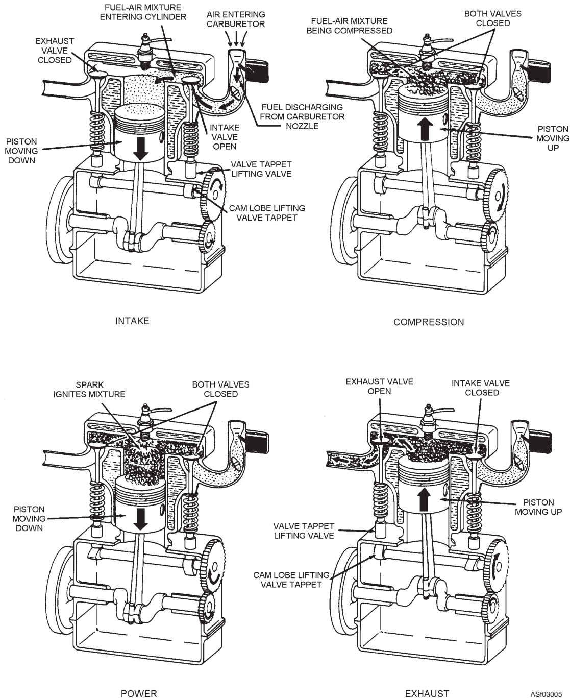
Figure 3-5.—Four-stroke cycle in a gasoline engine.
