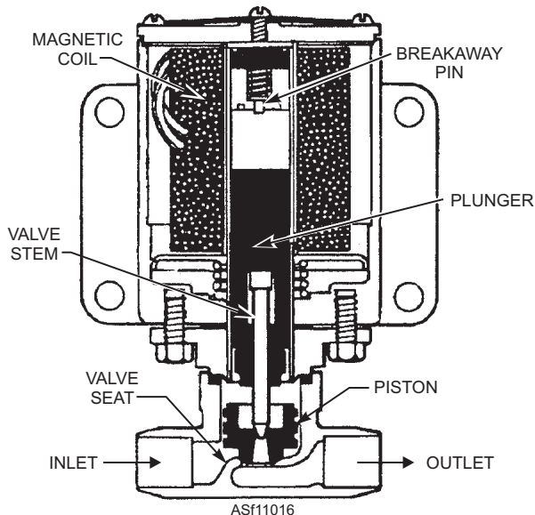
Figure 11-16.—Solenoid valve.
