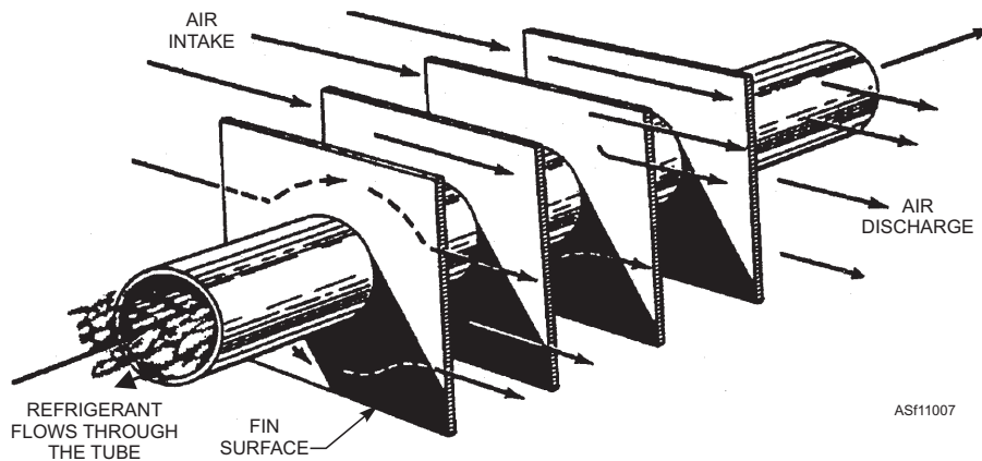
Figure 11-7.—Construction of an air-cooled condenser.
