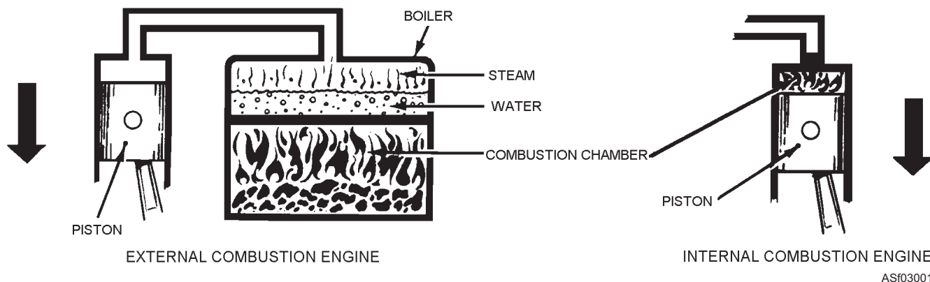
Figure 3-1.—Simple external and internal combustion engines.
