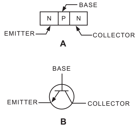
ASf07007 Figure 7-7.—NPN transistor—(A) NPN diagram; (B) schematic symbol.
