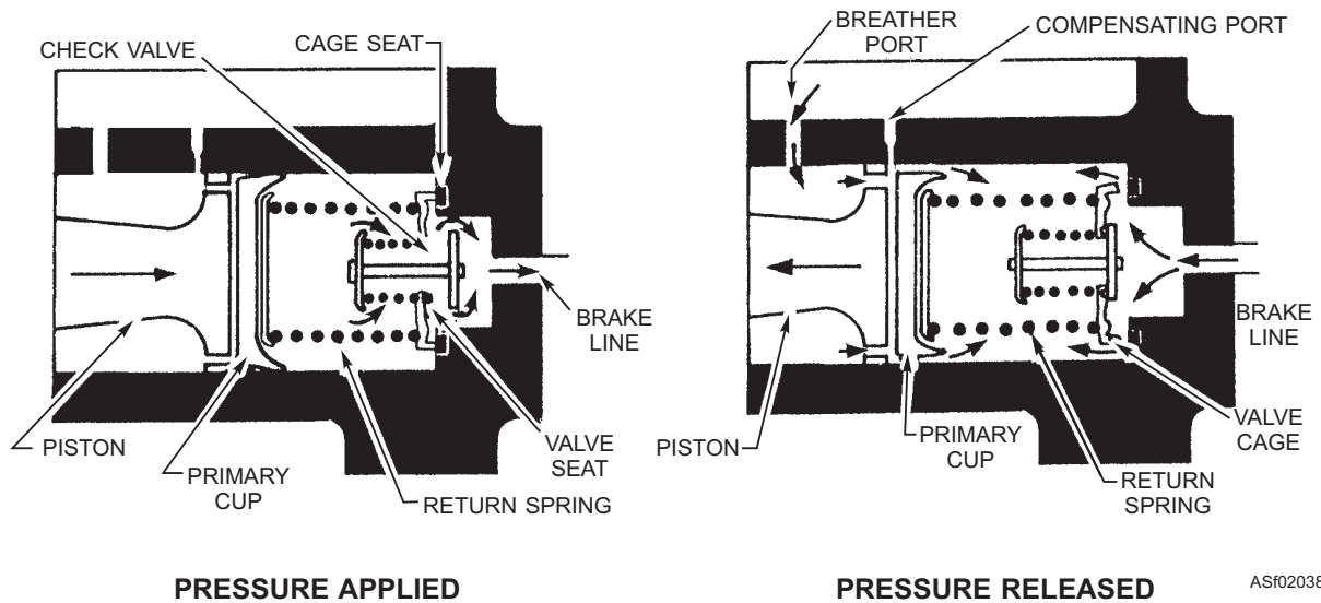
Figure 2-38.—Hydraulic brake master cylinder—operation of two-way valve.
