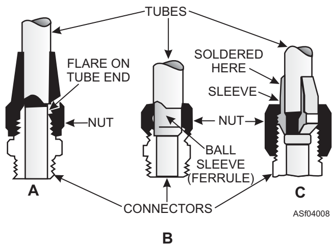
Figure 4-8.—Types of fittings used on fuel lines. (A) Flared. (B) Compression. (C) Soldered.
