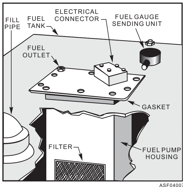
Figure 4-7.—Tank unit type of electric pump.
