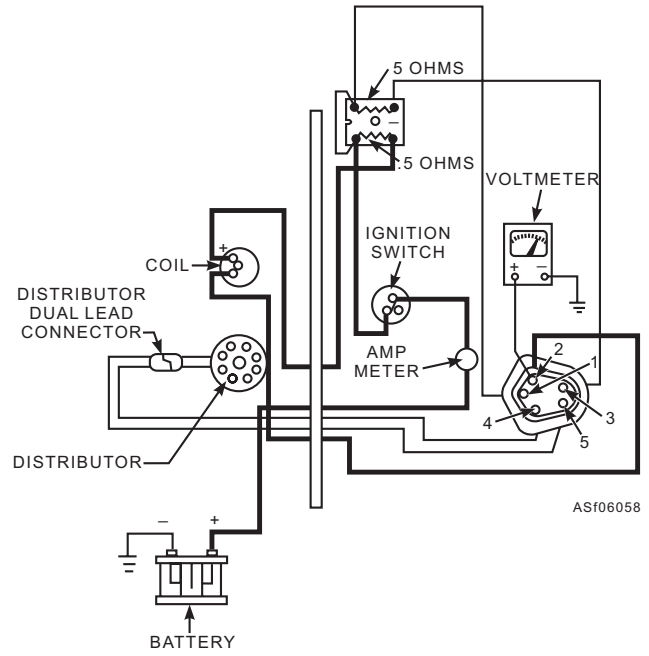
Figure 6-58.—Harness connector No. 2 test.
