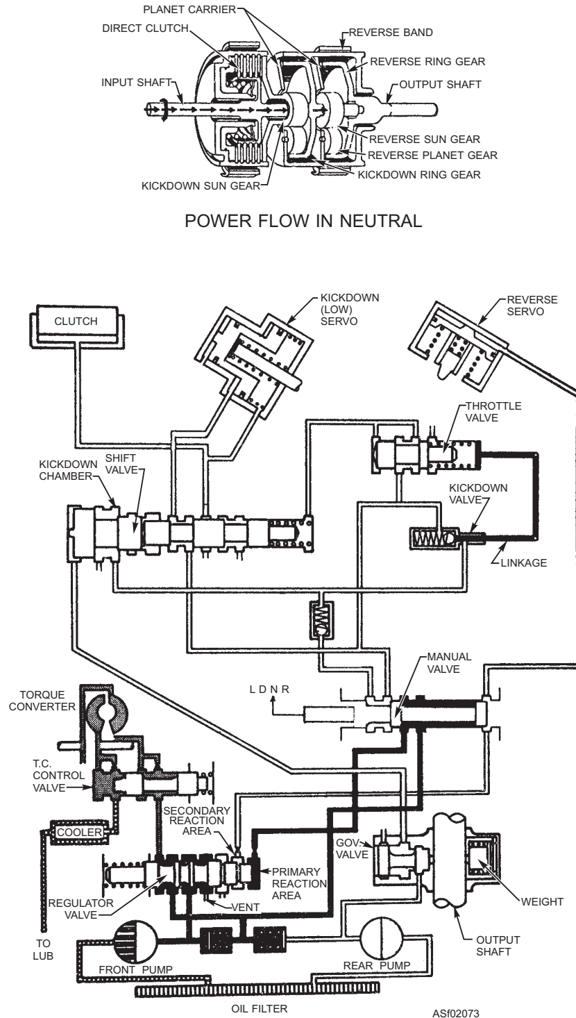
Figure 2-73.—Neutral (N) operating range.
