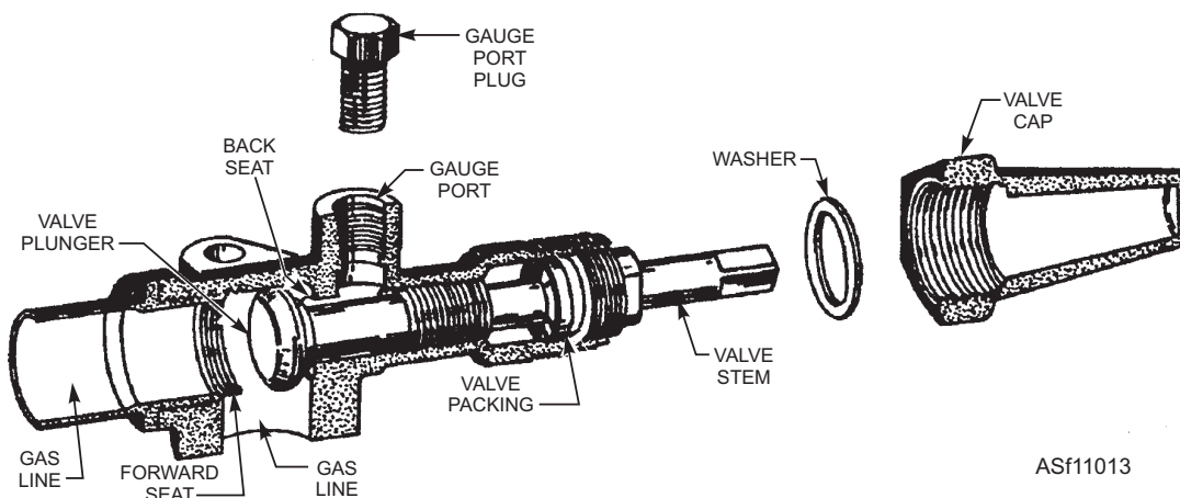
Figure 11-13.—Service valve.
