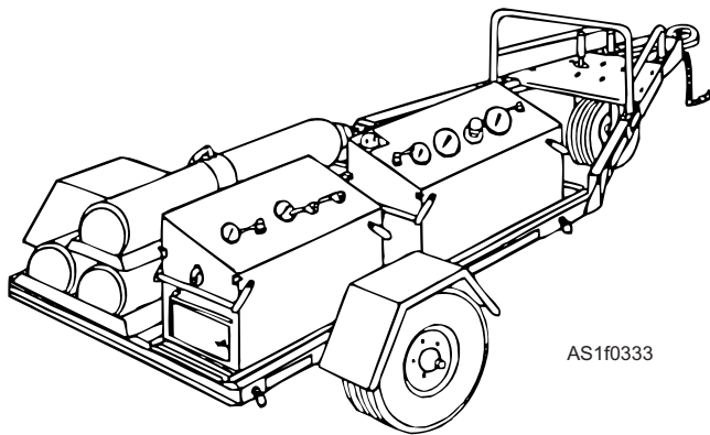
Figure 1-35.—A/U26U-1A oxygen servicing unit.
