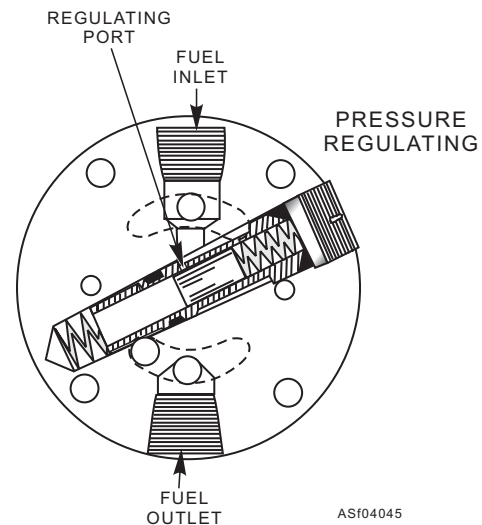
Figure 4-45.—Regulating piston in pressure regulating position.
