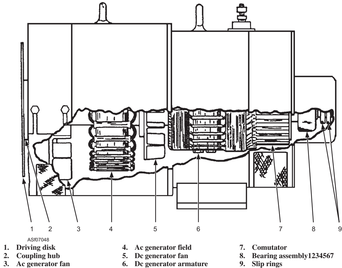
Figure 7-48.—Cutaway view of an NC-8A generator.
