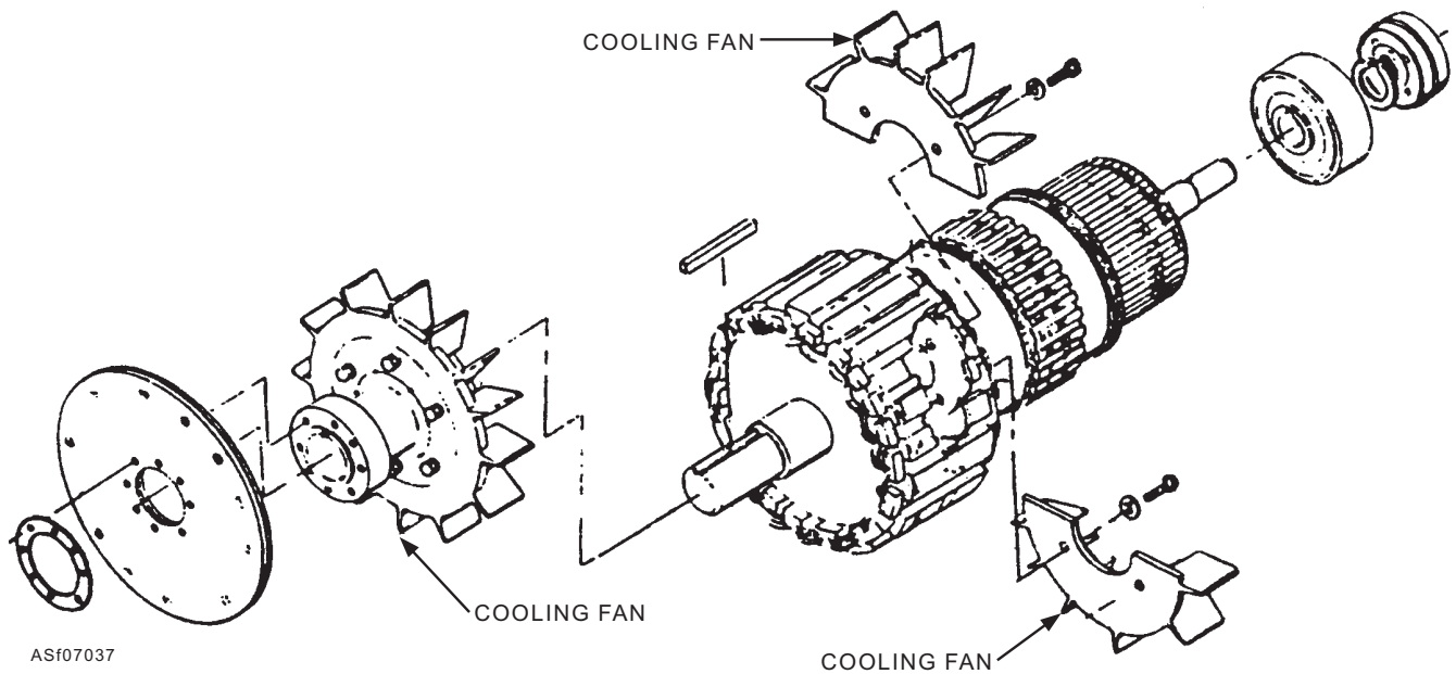
Figure 7-37.—Internal cooling fans of a typical generator.
