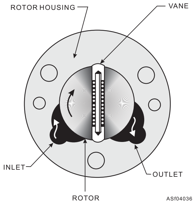
Figure 4-36.—Vaness and rotor in housing of a vane-type fuel pump.
