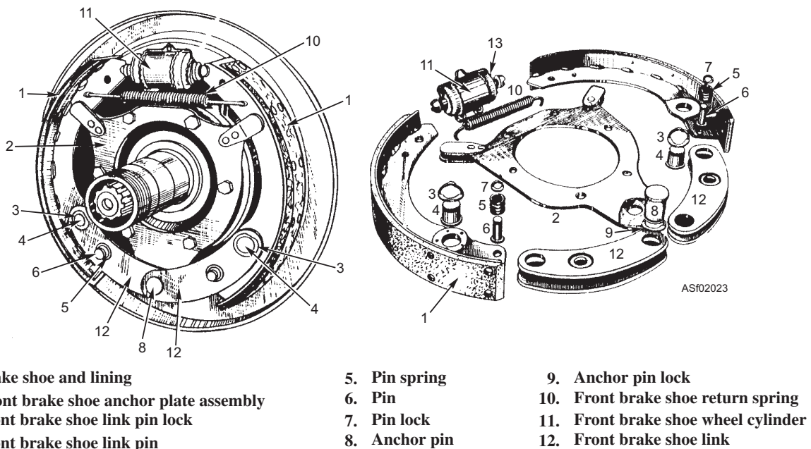
Figure 2-23.—Wheel brake assembled and exploded view.
