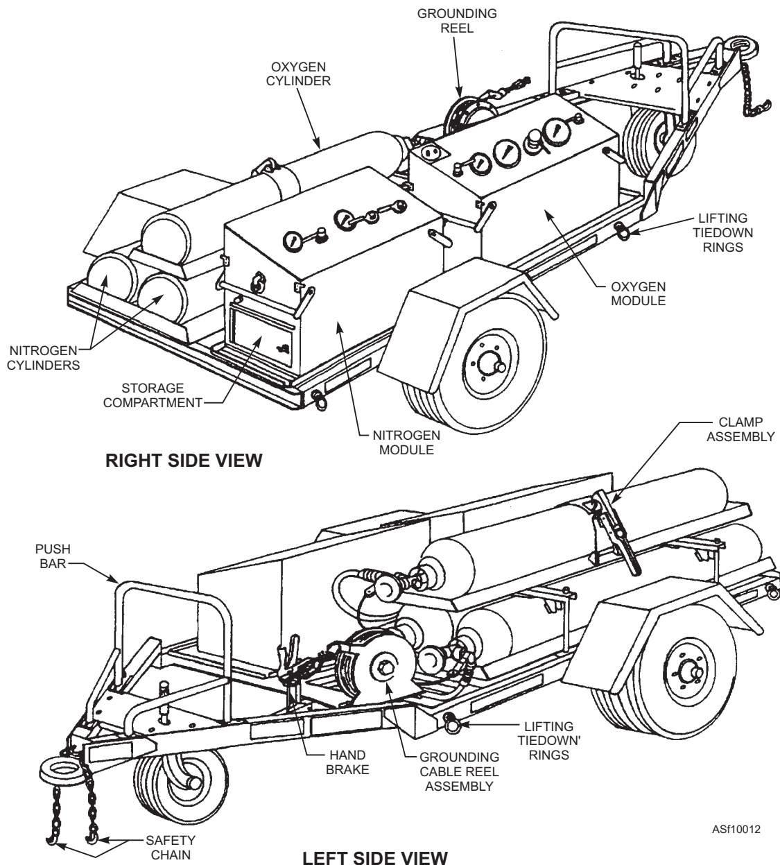
Figure 10-12.—A/U26U-1 oxygen servicing unit.
