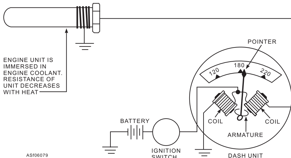
Figure 6-79.—Electrical temperature gauge.
