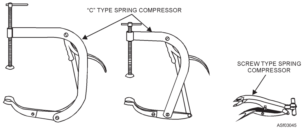
Figure 3-45.—Valve spring compressors for L-head and valve-in-head engines.
