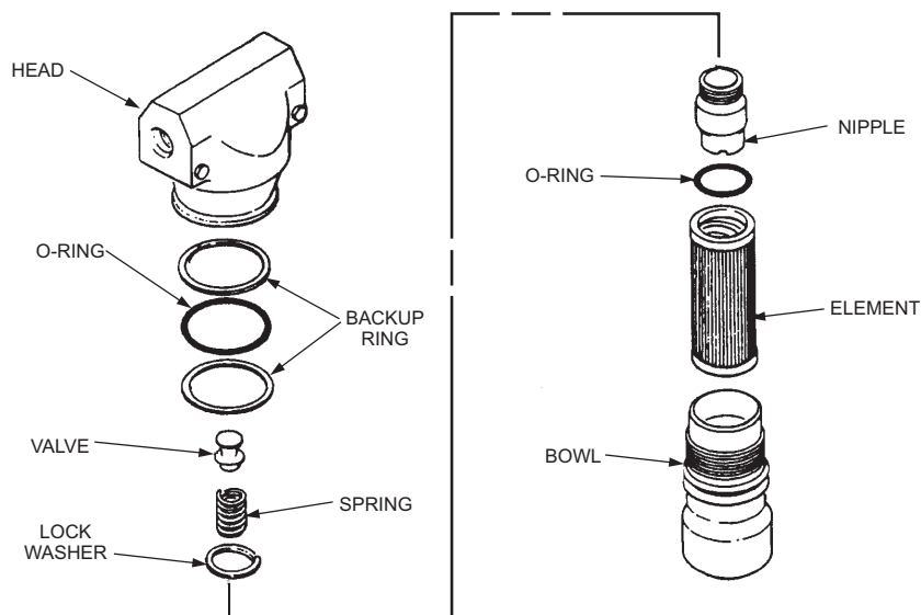
Figure 9-10.—Filter assembly.
