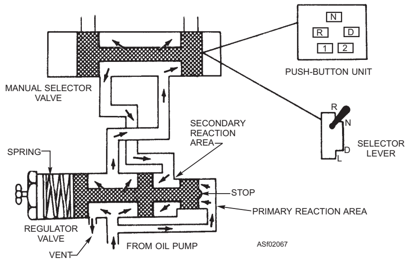
Figure 2-67.—Oil regulator.
