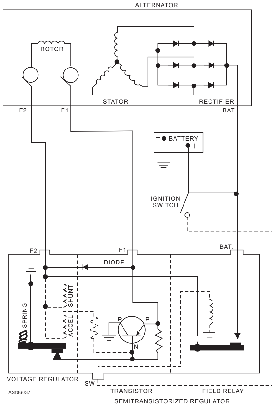
Figure 6-37.—Ac charging circuit using a semitransistorized regulator.
