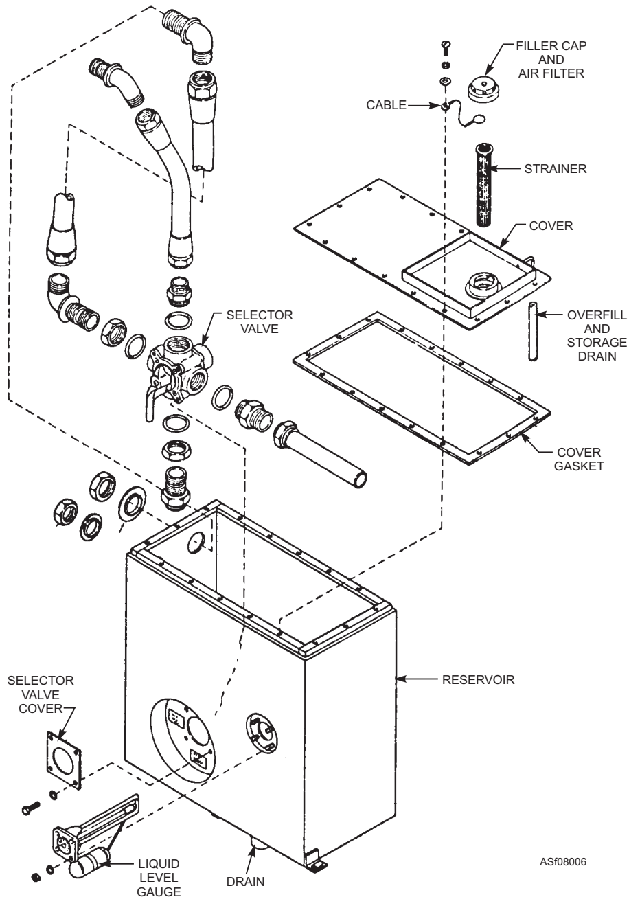
Figure 8-6.—Hydraulic Reservoir Assembly A/M27T-5.
