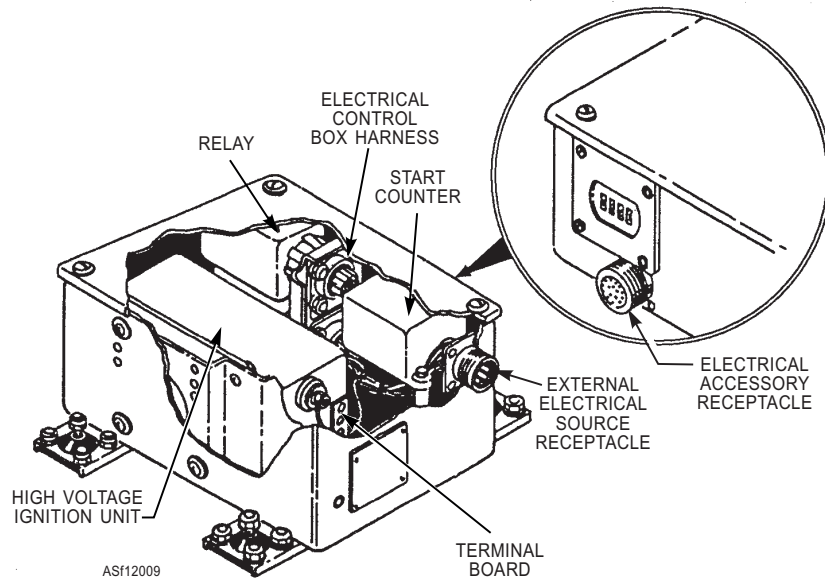
Figure 12-9.—Electrical control box.
