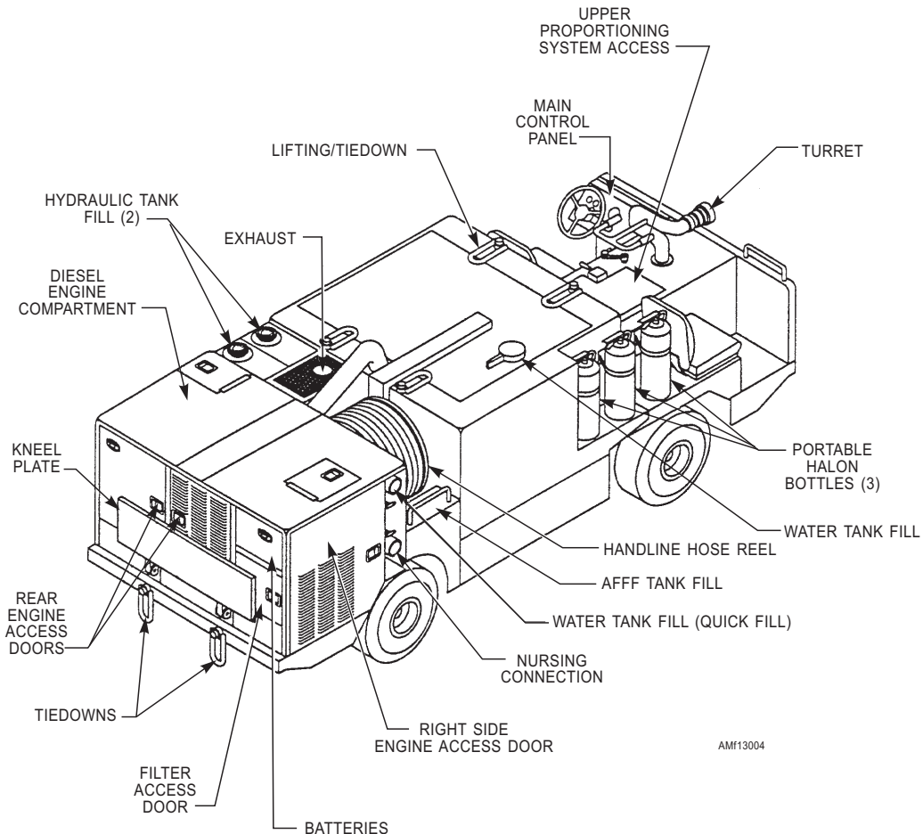
Figure 13-4.—A/S32P-25 fire-fighting truck.
