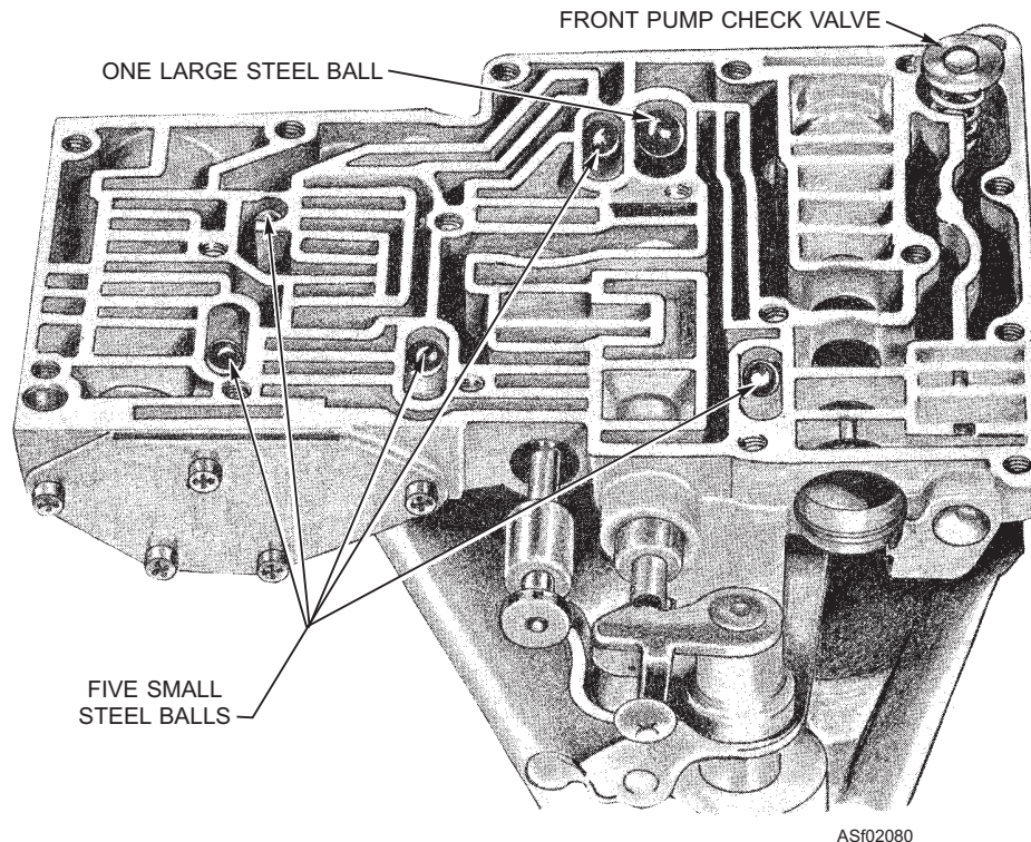
Figure 2-80.—Typical hydraulic control unit.
