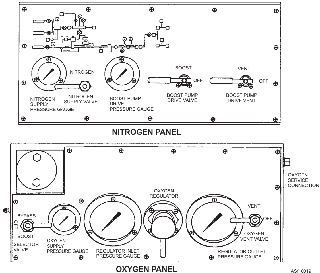
Figure 10-19.—Servicing controls and indicators.
