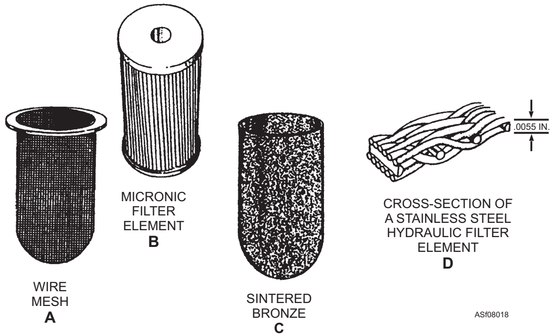
Figure 8-18.—Different types of hydraulic filter elements.
