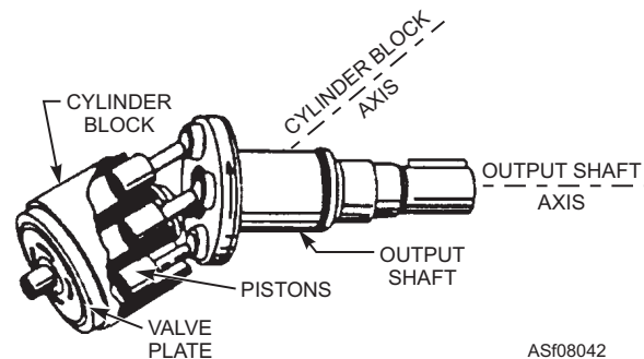
Figure 8-42.—Piston-type motor.
