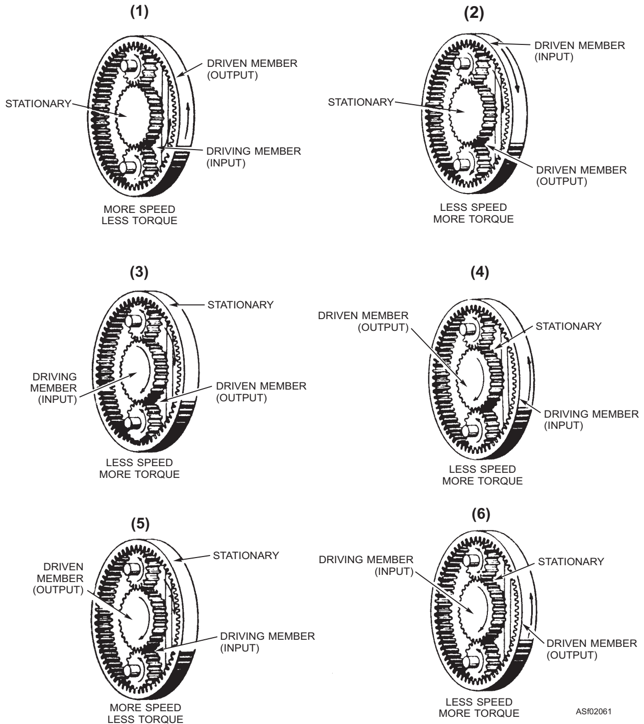
Figure 2-61.—Views of six speed/torque ratios for a simple planetary gear system.
