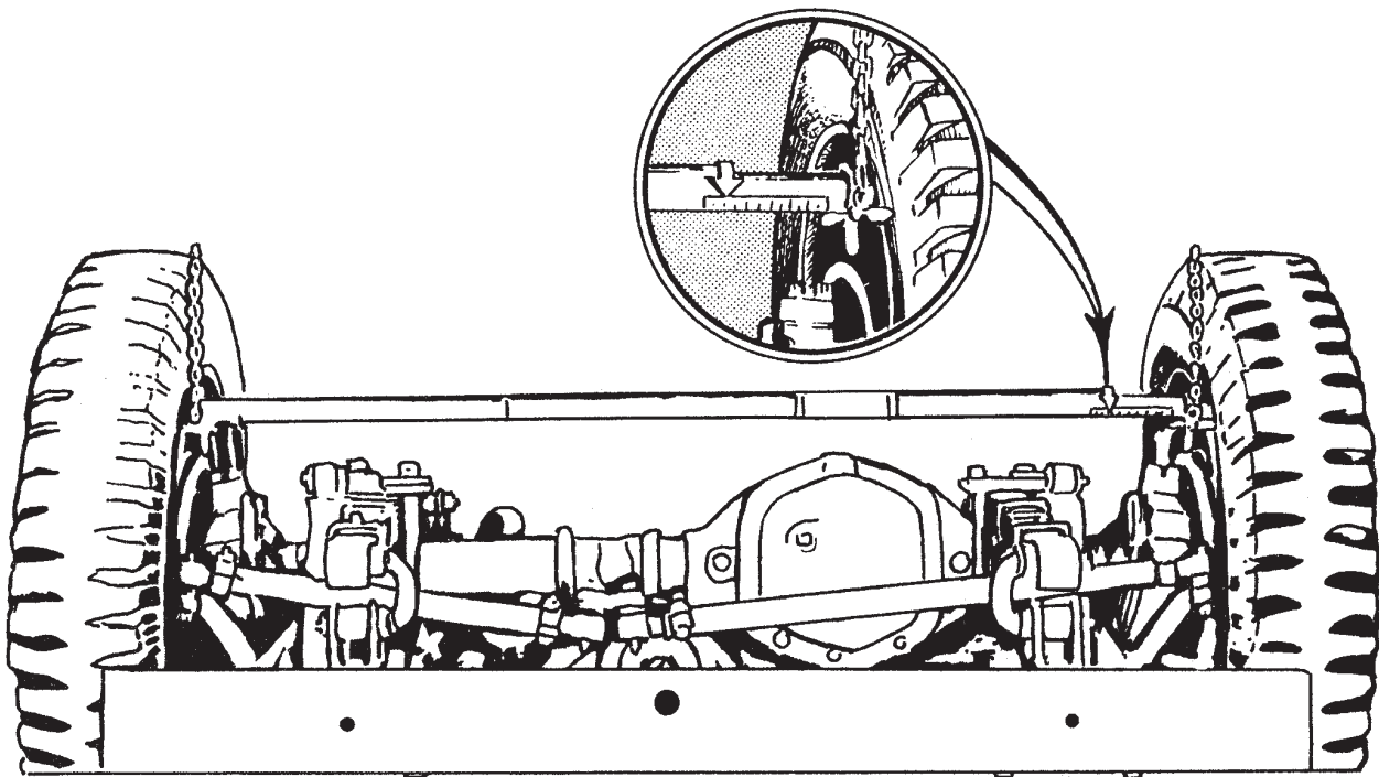
Figure 2-16.—Measuring pole.
