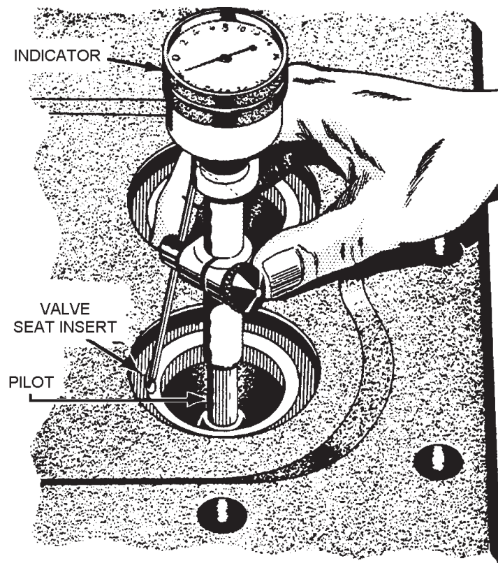
Figure 3-48.—Using a valve seat dial gauge.
