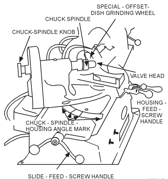
Figure 3-47.—Valve refacing machine.
