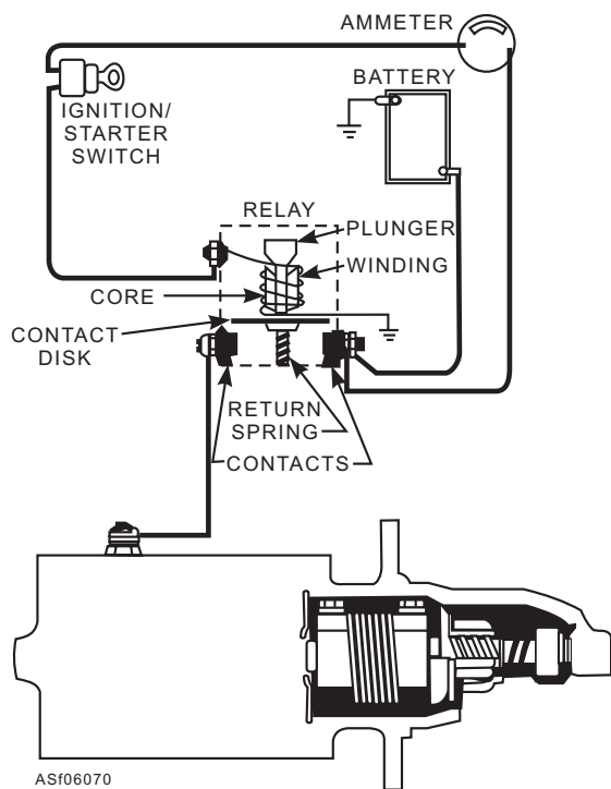
Figure 6-70.—Control system for a starter with a Bendix drive.
