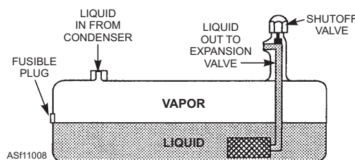
Figure 11-8.—Refrigerant receiver.
