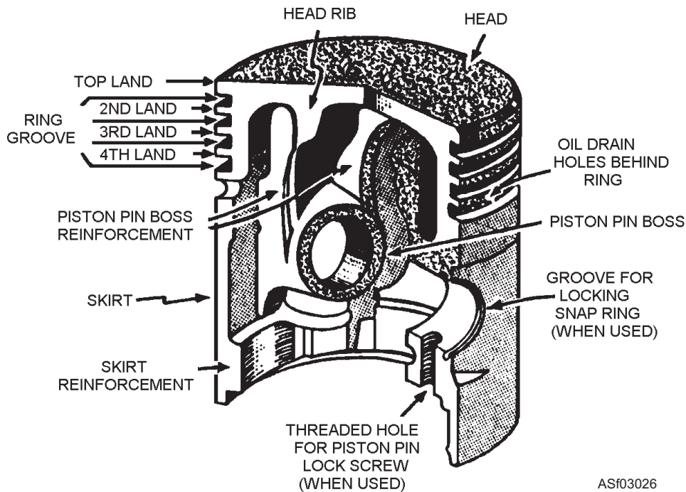
Figure 3-26.—The parts of a piston.
