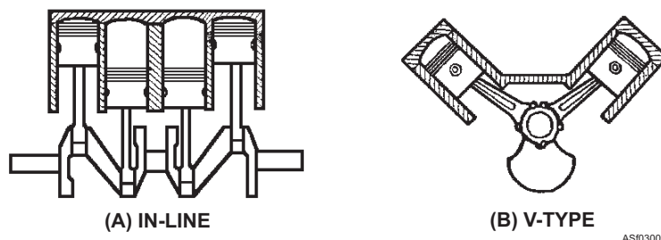
Figure 3-9.—Typical cylinder arrangements.
