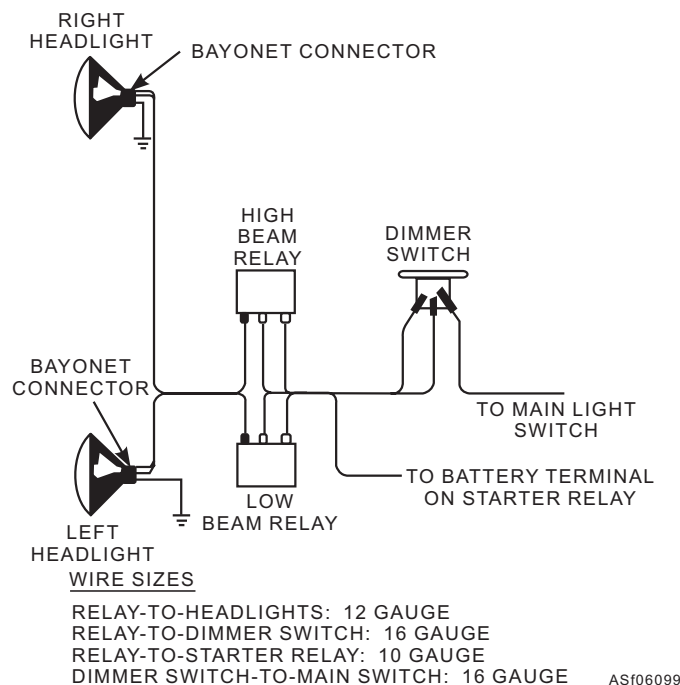
Figure 6-99.—Light relay wiring diagram.
