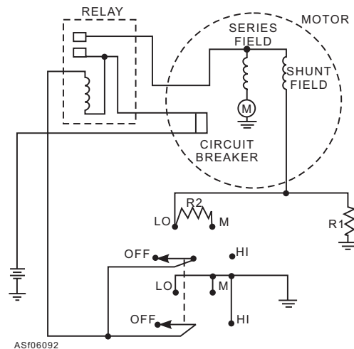
Figure 6-92.—Schematic diagram of a three-speed windshield wiper.
