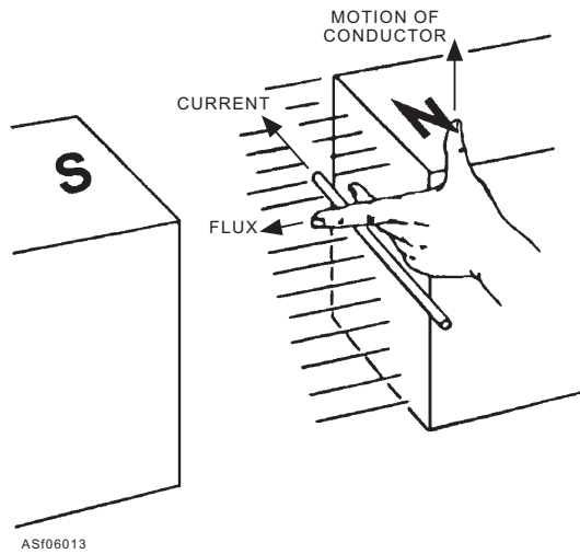
Figure 6-13.—Left-hand rule for generators.
