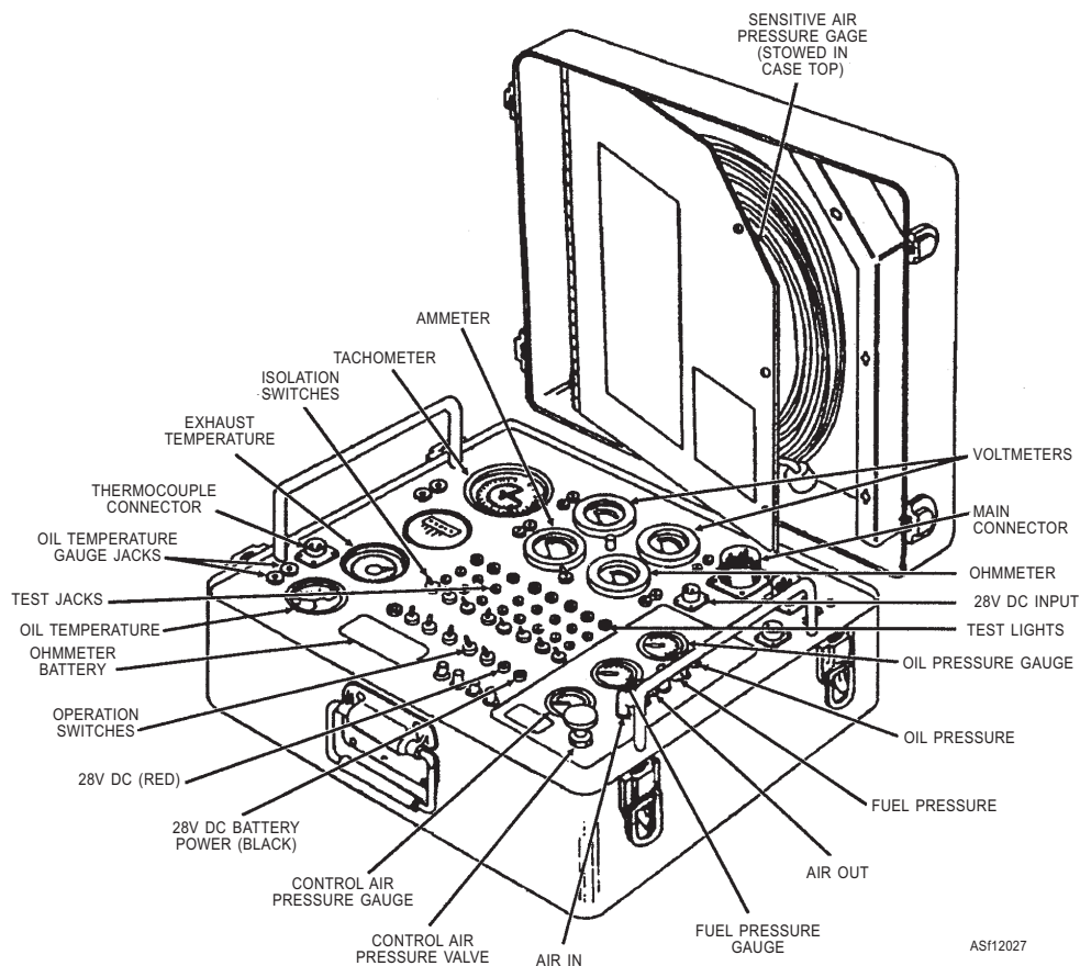
Figure 12-27.—Gas turbine engine analyzer.
