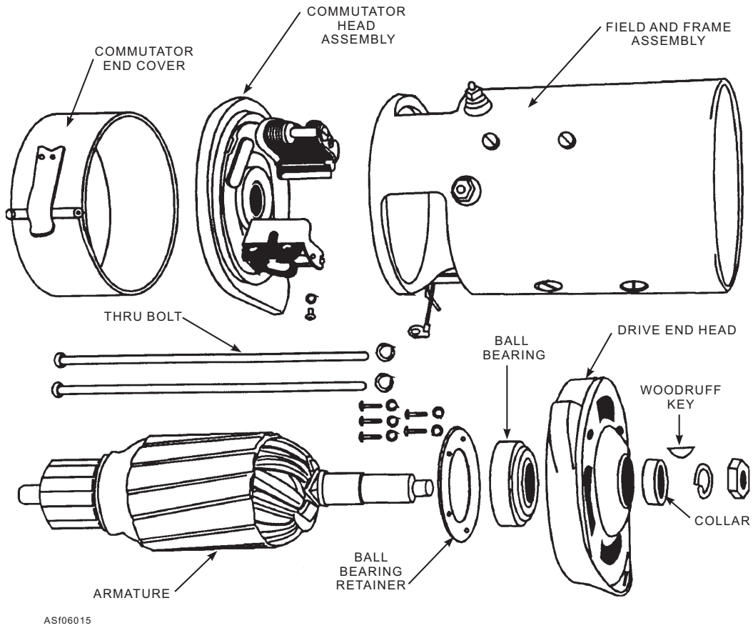
Figure 6-15.—Two-brush, dc generator.
