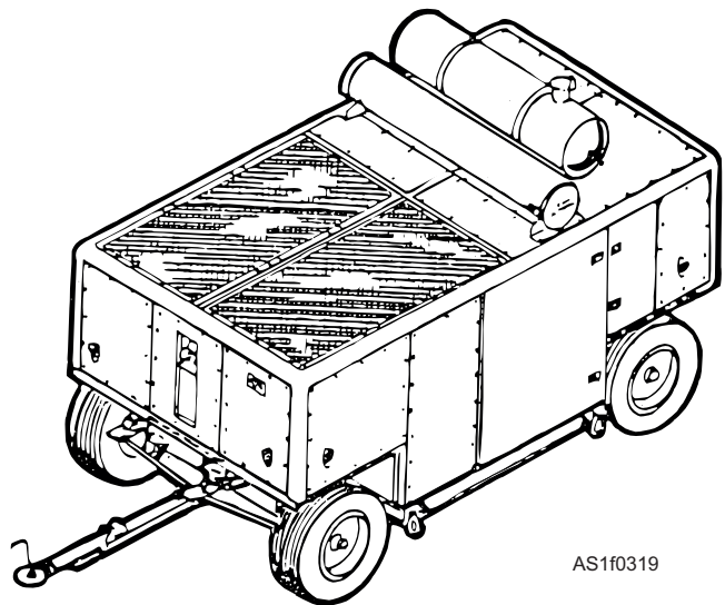
Figure 1-21.—A/M32C-17 mobile air-conditioner.
