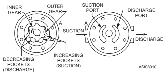
Figure 8-10.—Internal gear pump.
