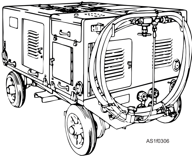
Figure 1-8.—A/M27T-5 portable hydraulic power supply.
