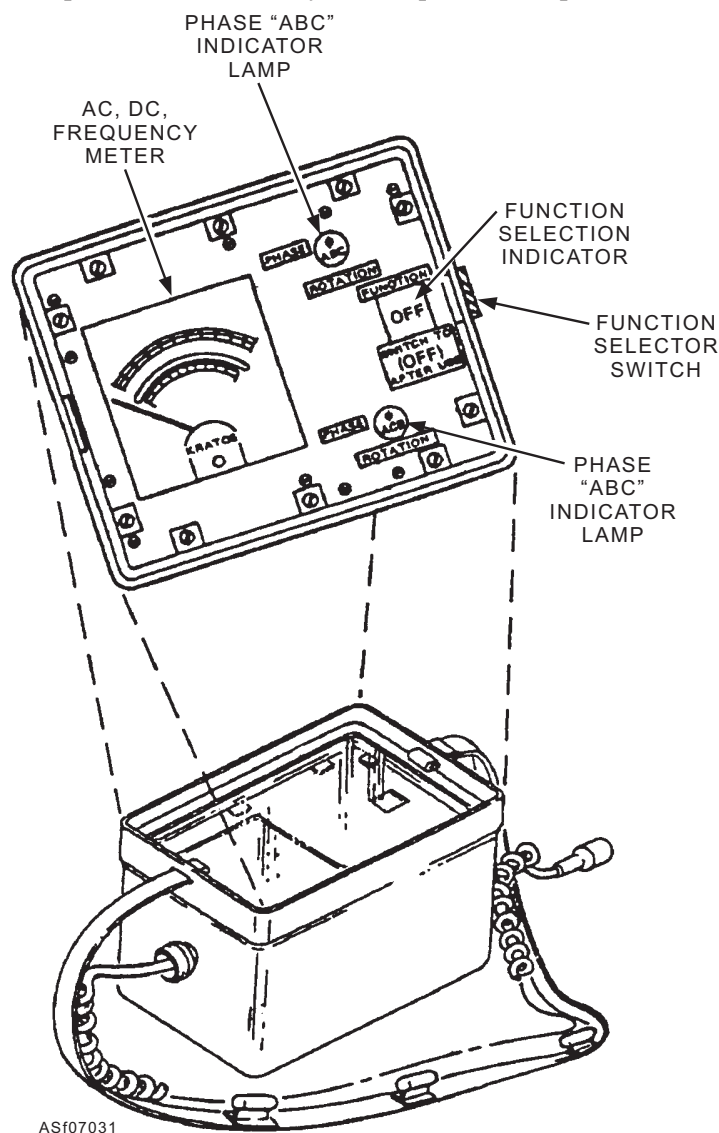
Figure 7-31.—AN/USM-128A electrical test set.
