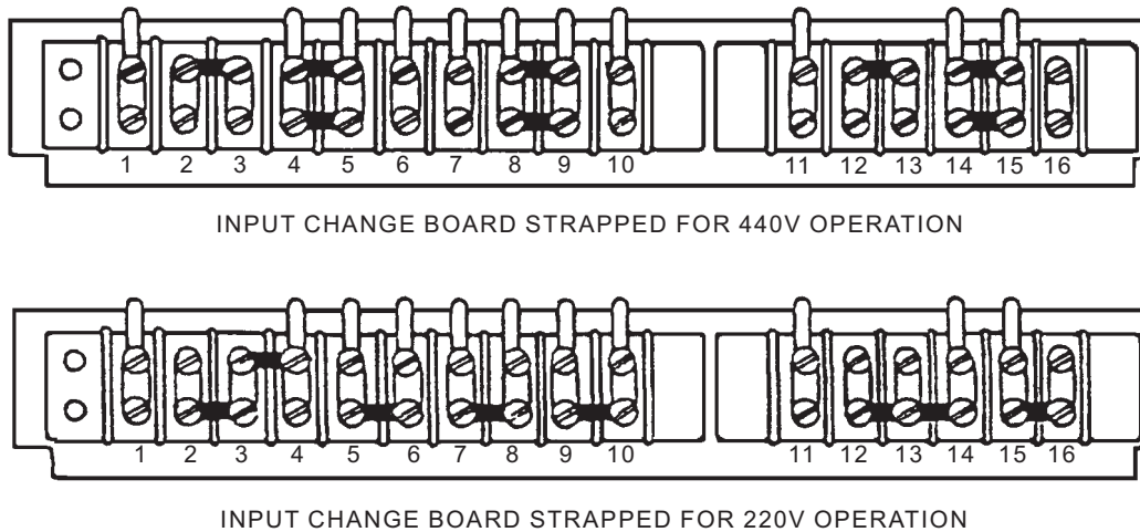
Figure 7-58.—DC input change board.
