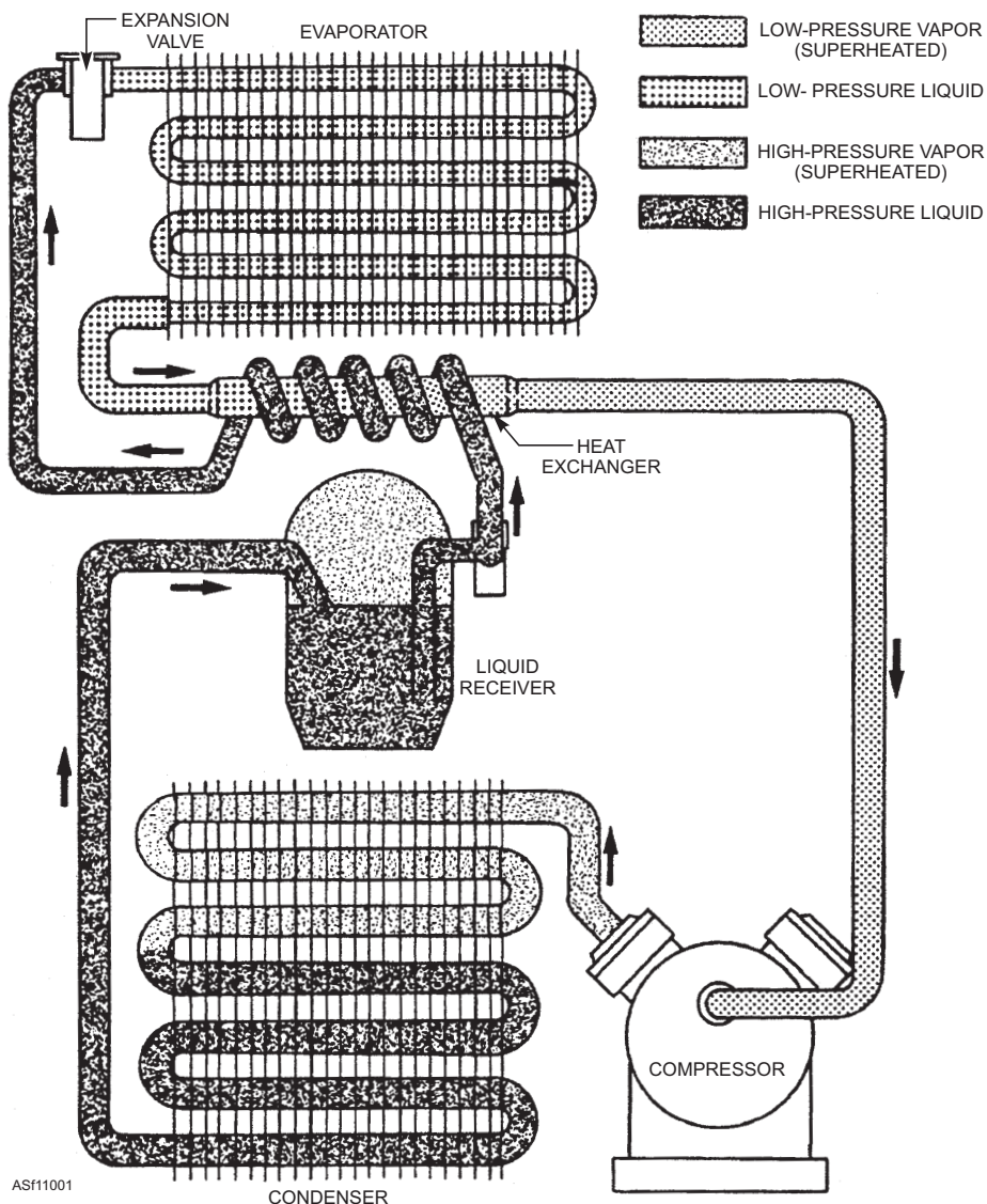
Figure 11-1.—Fundamental refrigeration cycle.
