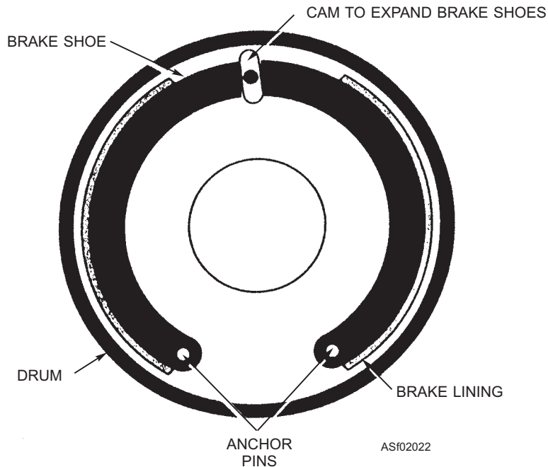
Figure 2-22.—Internal expanding brake.
