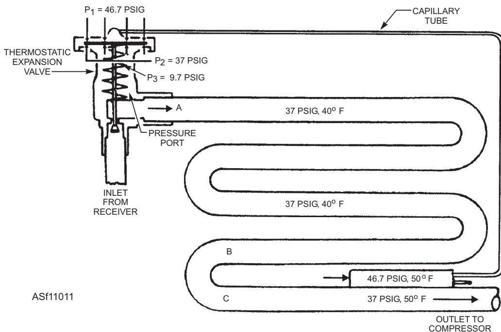
Figure 11-11.—Thermostatic expansion valve and evaporator.
