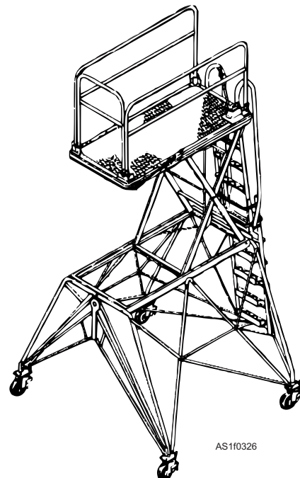
Figure 1-28.—B-5A maintenance platform.
