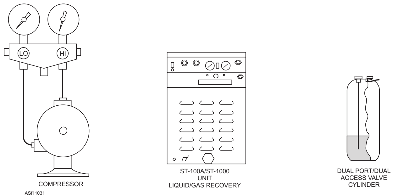
Figure 11-31.—Refrigerant recovery method.
