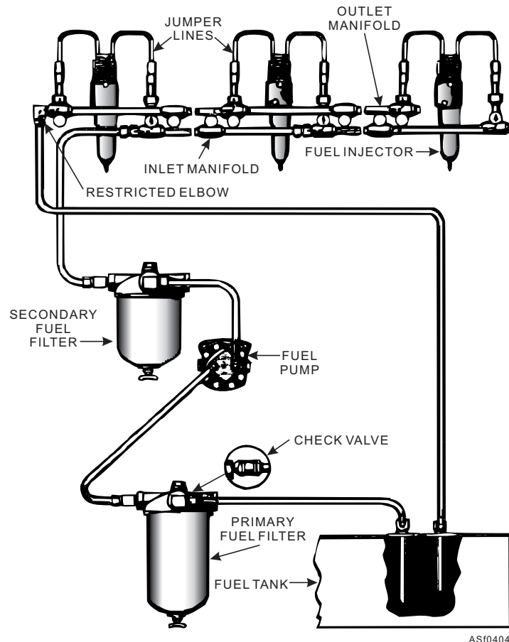
Figure 4-47.—Diagram of typical General Motors diesel fuel system.
