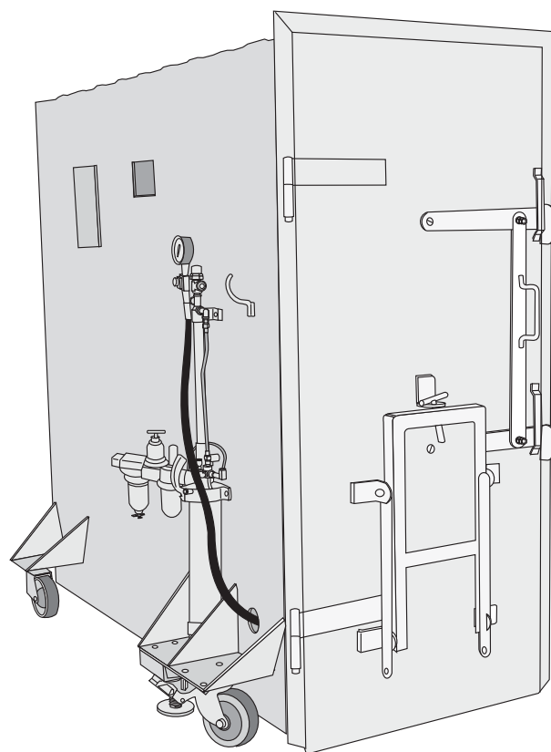
Figure 2-97.—Safety cage for inflation of tires.
