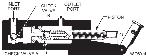
Figure 8-14.—Double-action hydraulic hand pump.
