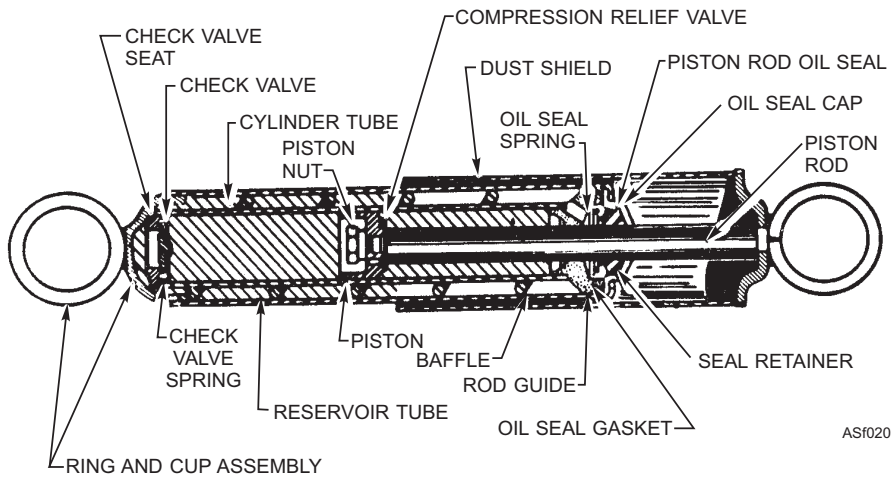
Figure 2-6.—Double-acting shock absorbers.
