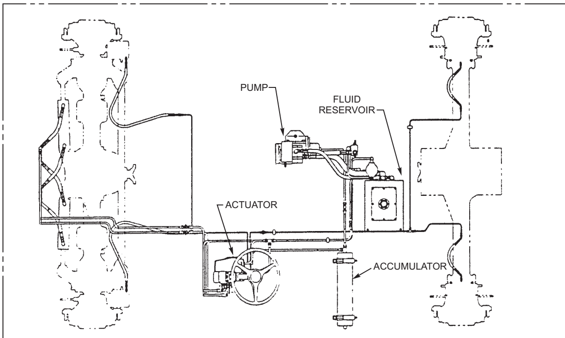
Figure 2-41.—Hydraulic system of the A/S32A-37 tow tractor.
