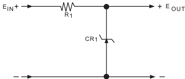
Figure 7-6.—Zener diode voltage regulating circuit.
