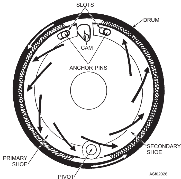
Figure 2-26.—Primary and secondary brake shoes—self-energizing action.
