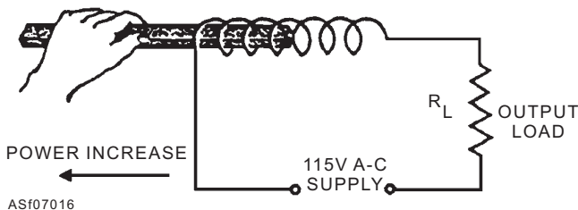
Figure 7-16.—Varying coil inductance mechanically.
