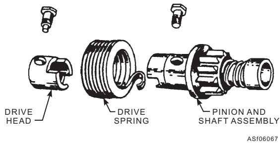
Figure 6-67.—Bendix drive construction.
