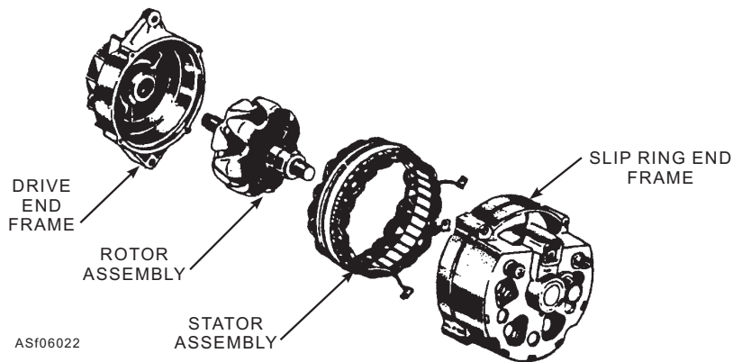
Figure 6-22.—A disassembled alternator.
