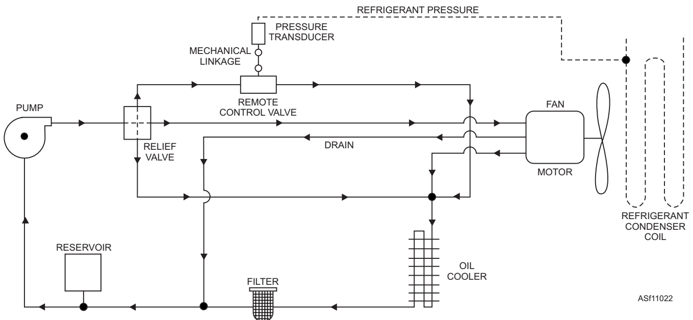
Figure 11-22.—Hydraulic system.
