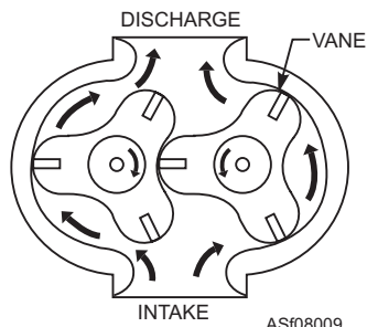
Figure 8-9.—Lobe pump.
