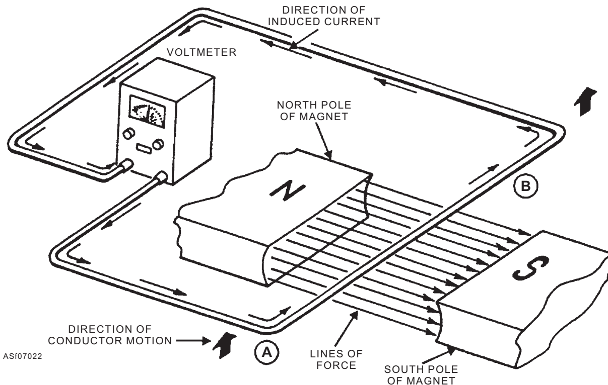
Figure 7-22.—Electromagnetic induction principles.
