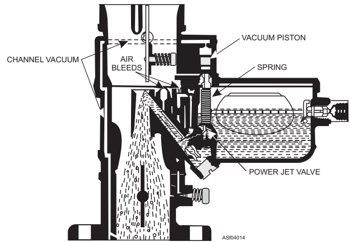
Figure 4-14.—Power jet full load circuit.
