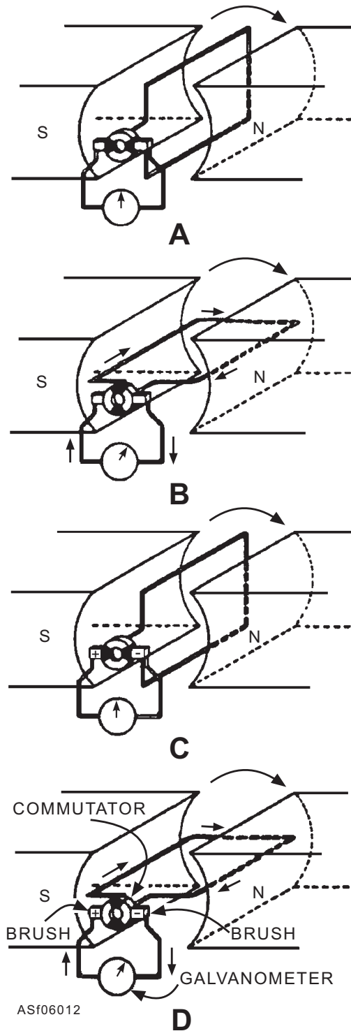
Figure 6-12.—Generating direct-current electrical energy.
