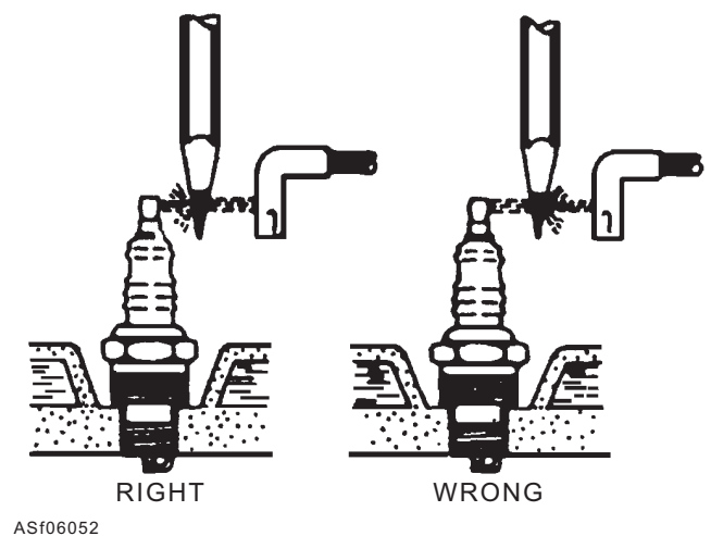
Figure 6-52.—One method of checking coil polarity.
