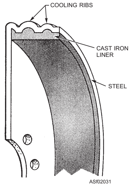
Figure 2-31.—Sectional view of a brake drum.
