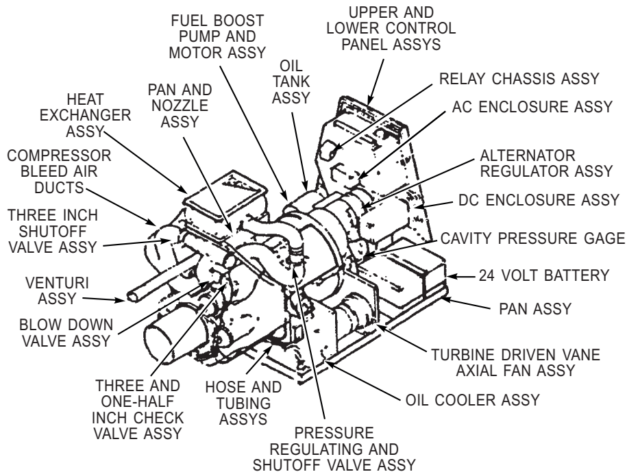
Figure 12-23.—A/M47A-4 flyaway assembly.
