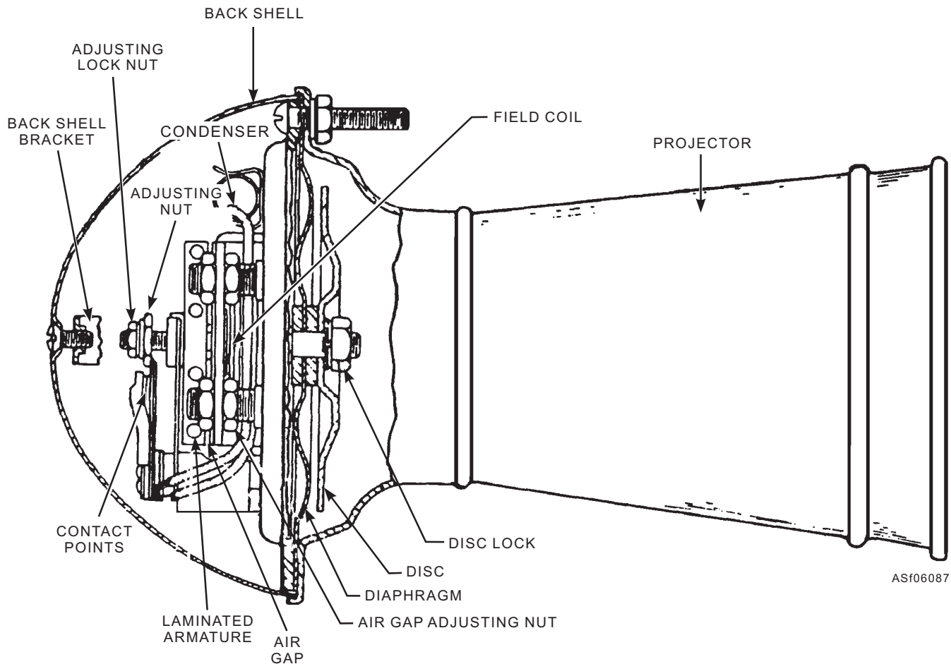
Figure 6-87.—Electrical vibrator-type horn.
