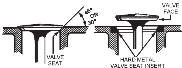
Figure 3-43.—Valve head and set angle.
