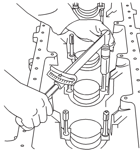
Figure 3-11.—Torque wrench in use, tightening main bearing stud of an engine.
