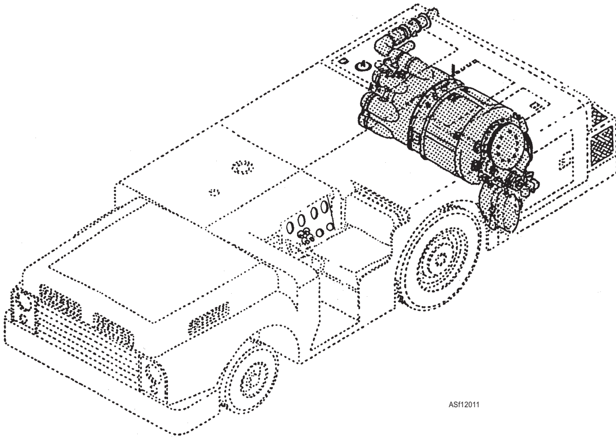
Figure 12-11.—GTCP-100 gas turbine engine in enclosure.
