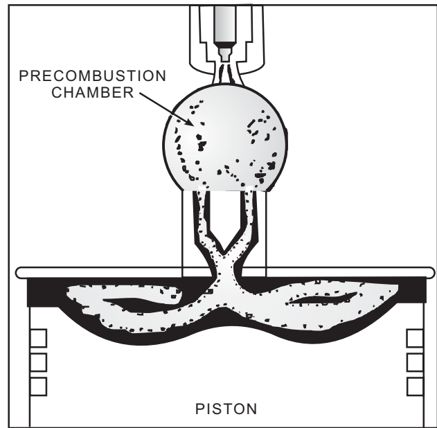
Figure 4-28.—Diesel engine precombustion chamber.
