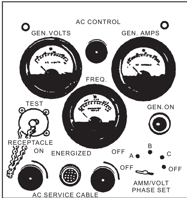
Figure 7-46.—AC Control panel.
