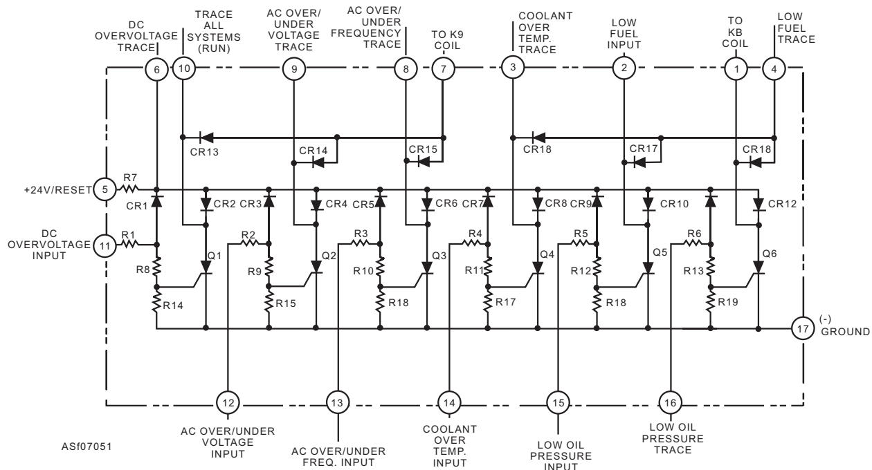
Figure 7-51.—NC-8A fault board.
