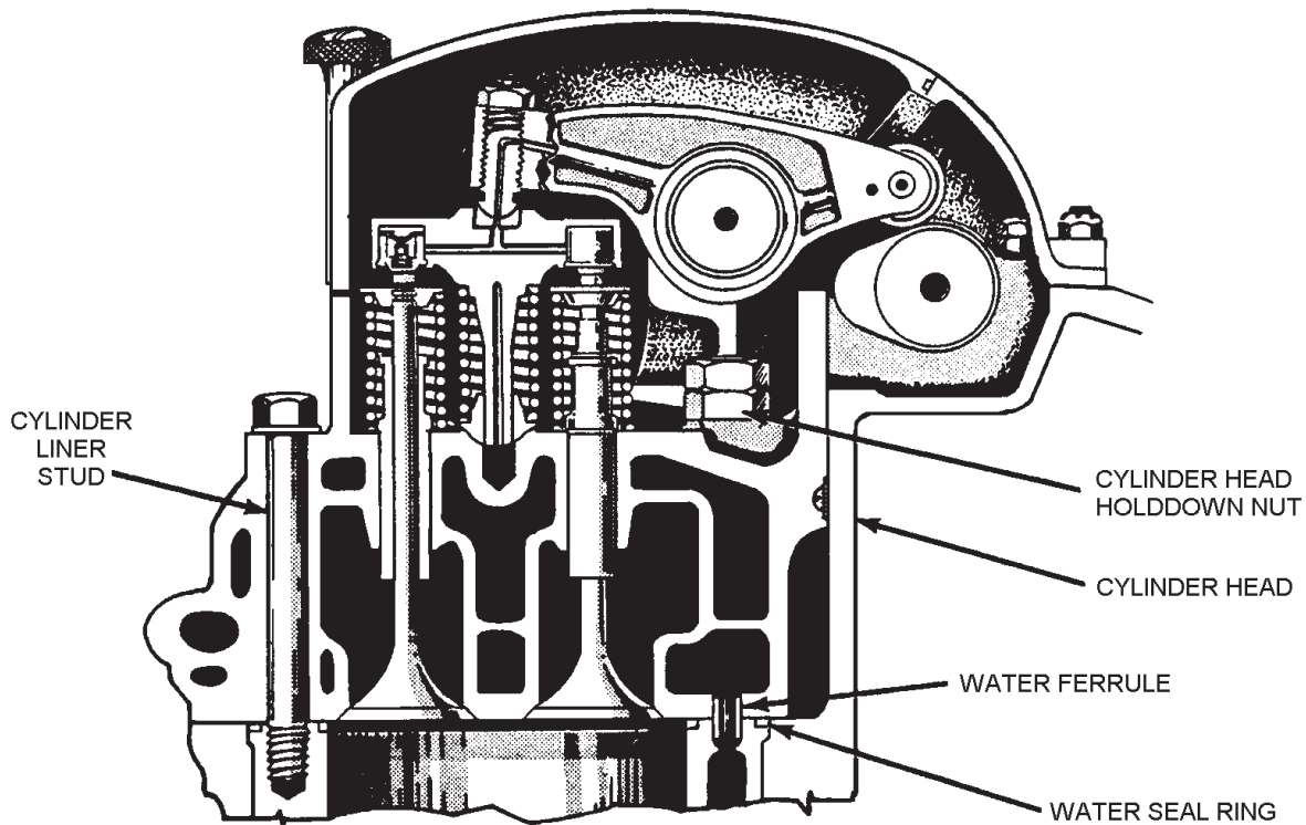
Figure 3-22.—Cylinder head for overhead valve engine.
