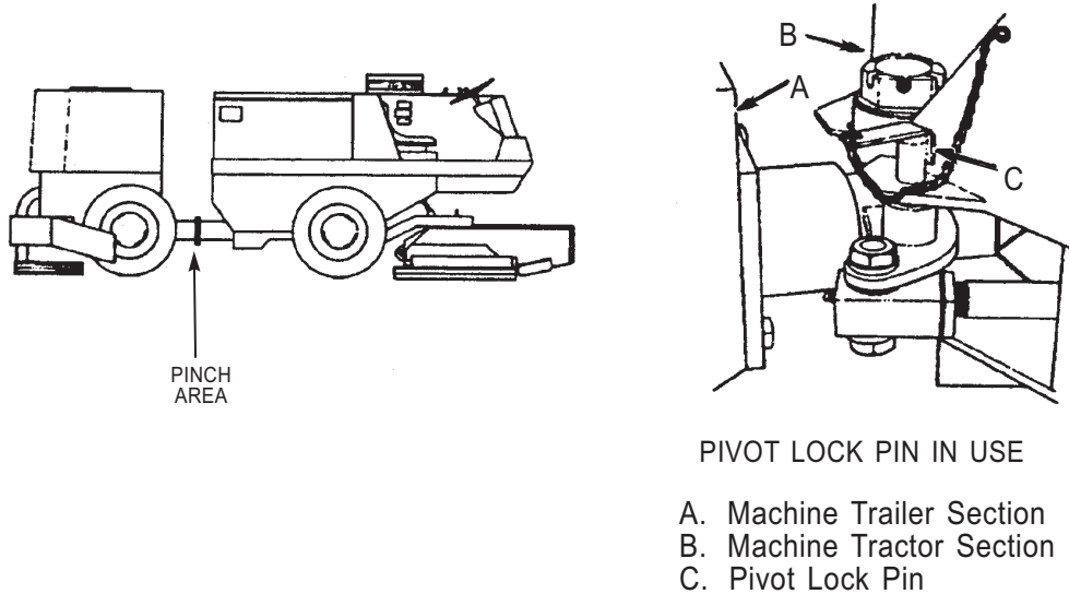
Figure 13-14.—Pinch area and pivot lock pin.
