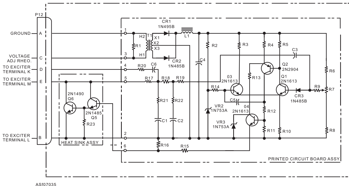
Figure 7-35.—An ac voltage regulator (VR2) simplified schematic.
