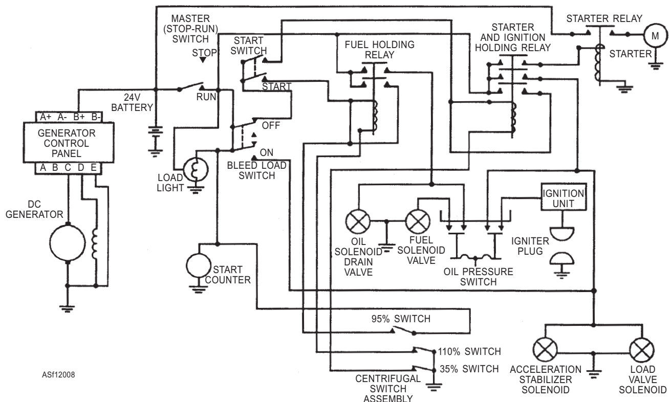
Figure 12-8.—Electrical system.
