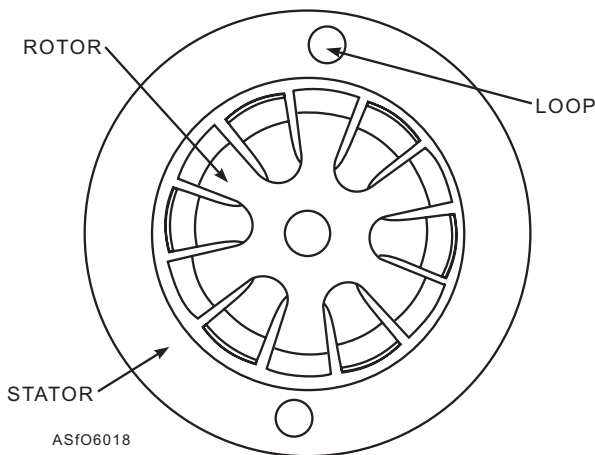
Figure 6-18.—A basic alternator with six pairs of poles in the rotor.
