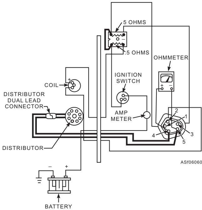
Figure 6-60.—Harness connector Nos. 4 and 5 tests.
