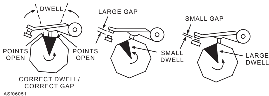
Figure 6-51.—Relationship of dwell and point gap.
