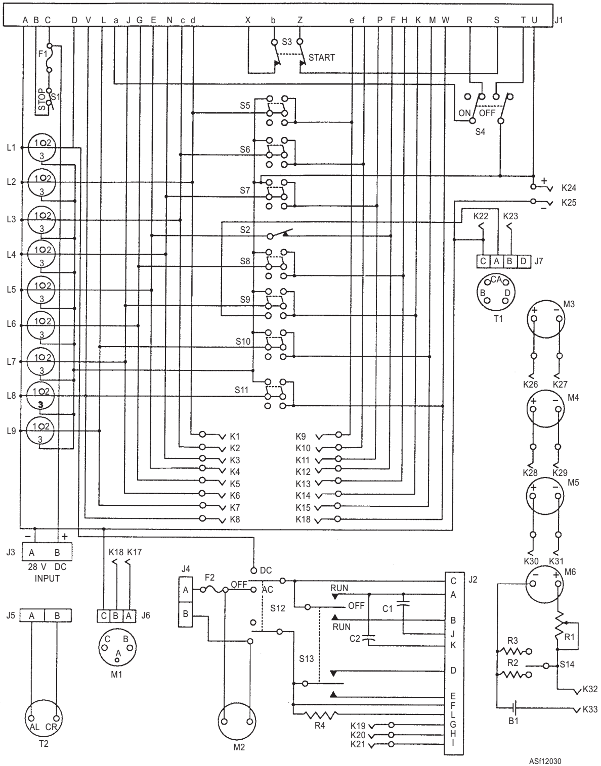
Figure 12-30.—Analyzer electrical schematic.
