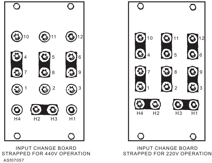
Figure 7-57.—AC input change board.
