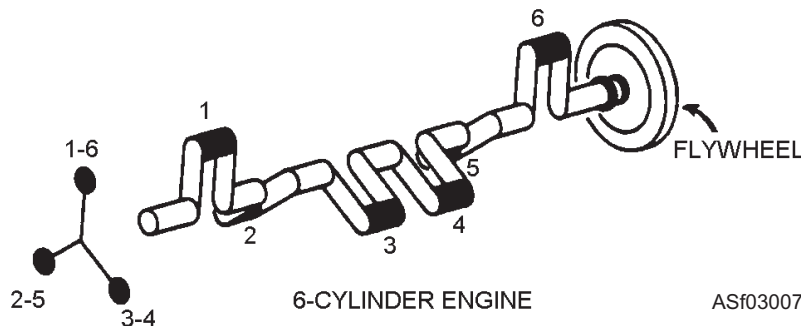
Figure 3-7.—Crankshaft for a 6-cylinder engine.
