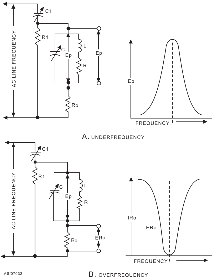
Figure 7-32.—Electrical frequency control circuits.
