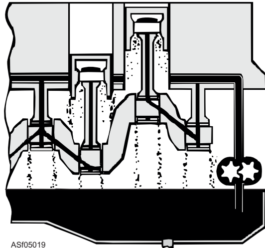
Figure 5-19.—Full force-feed lubrication system.
