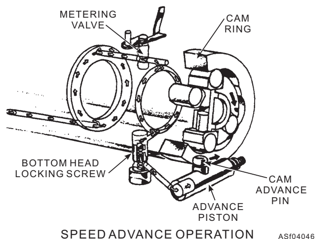
Figure 4-46.—Fuel flow in speed advance operation.
