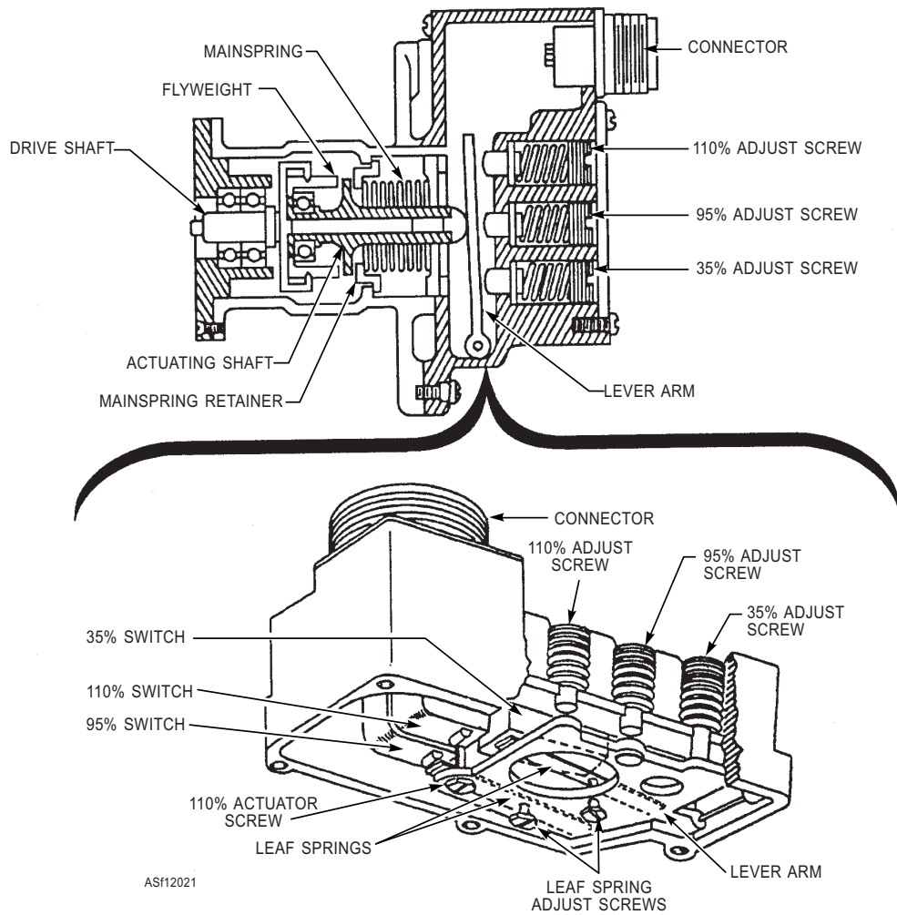
Figure 12-21.—Centrifugal switch assembly.
