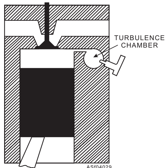
Figure 4-29.—Diesel engine turbulence combustion chamber.
