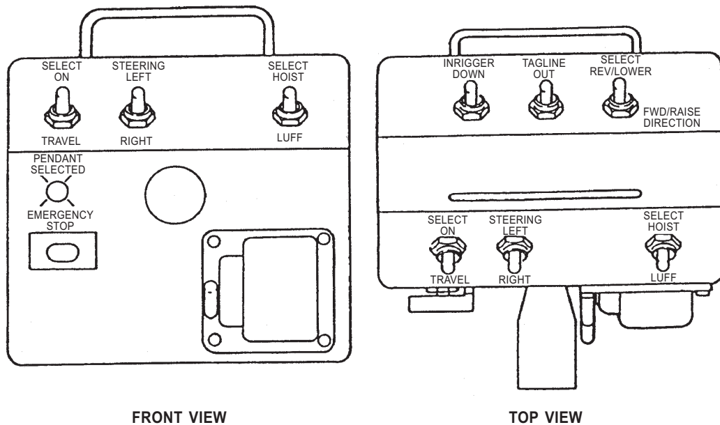
Figure 13-3.—Pendant control box.
