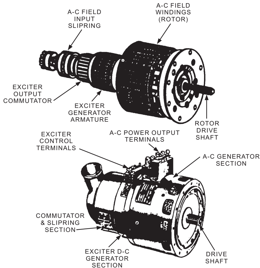
Figure 7-29.—An ac generator pictorial.
