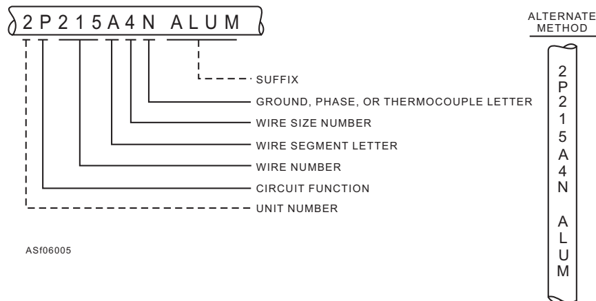
Figure 6-5.—Alphanumeric wire identification code.
