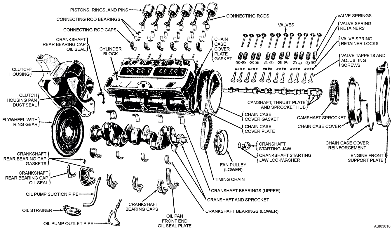
Figure 3-16.—Cylinder block and components.
