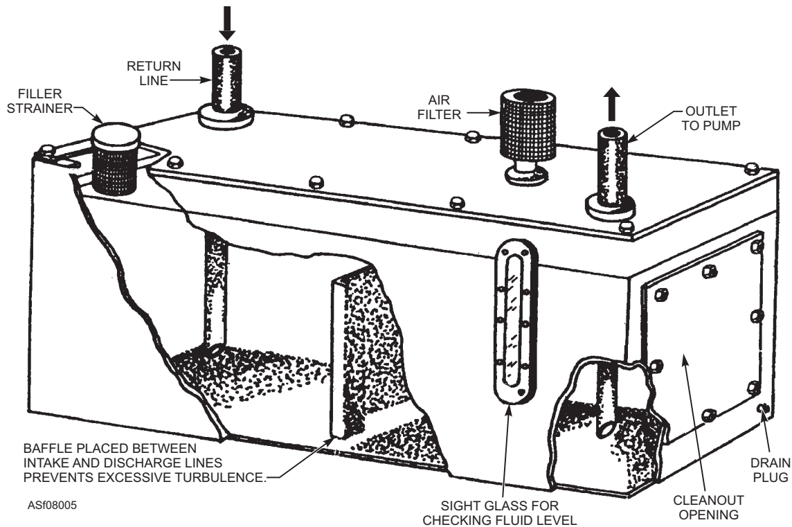
Figure 8-5.—Typical hydraulic reservoir.
