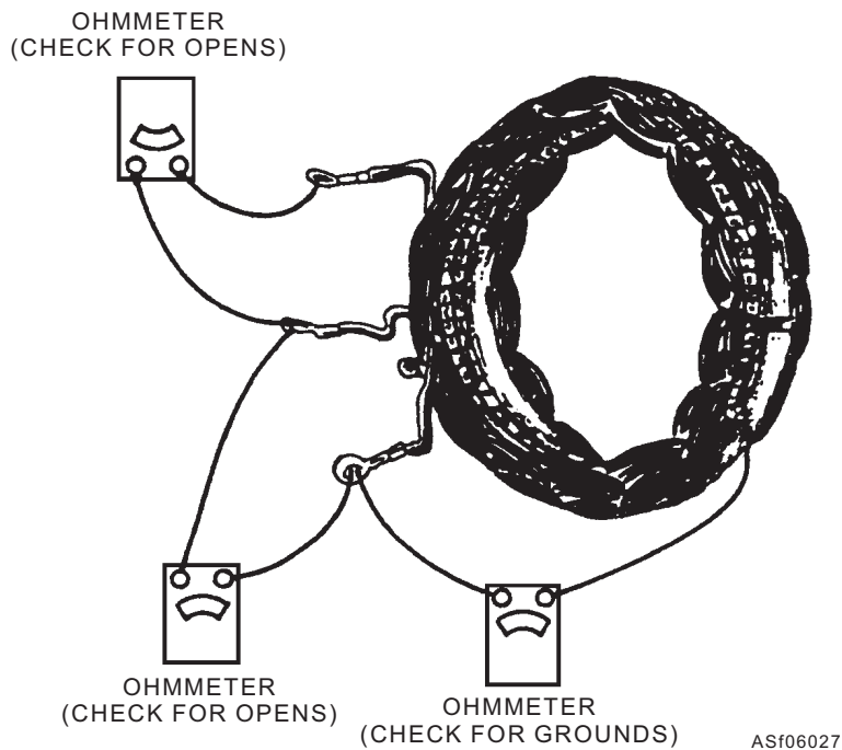
Figure 6-27.—Testing the stator for opens and grounds.
