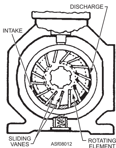
Figure 8-12.—Vane pump.
