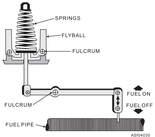
Figure 4-30.—Simple mechanical governor.
