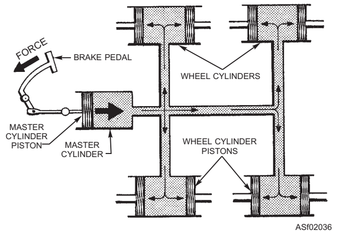
Figure 2-36.—Operation of hydraulic brake system.
