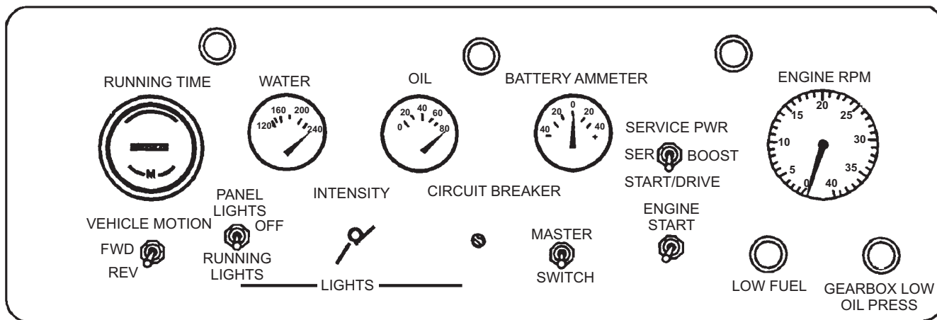
Figure 7-41.—Engine control panel.
