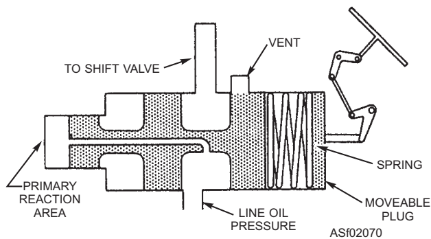
Figure 2-70.—Throttle valve.
