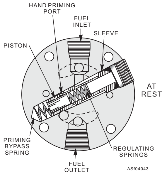
Figure 4-43.—Regulating piston at rest.
