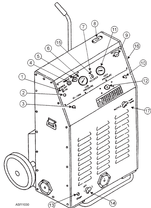
Figure 11-30.—Refrigerant recovery-recycle units.
