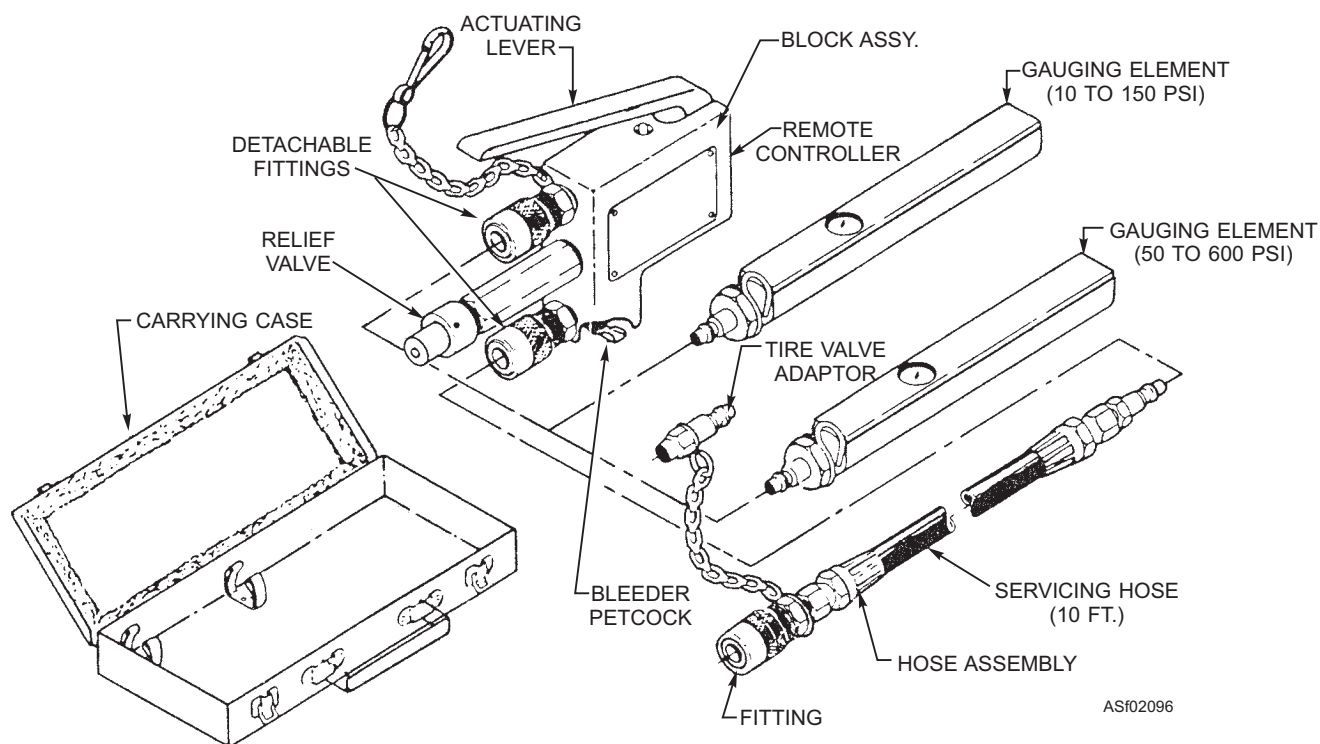
Figure 2-96.—Tire inflator assembly kit.
