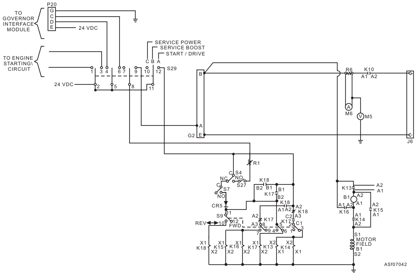
Figure 7-42.—Vehicle propulsion system.
