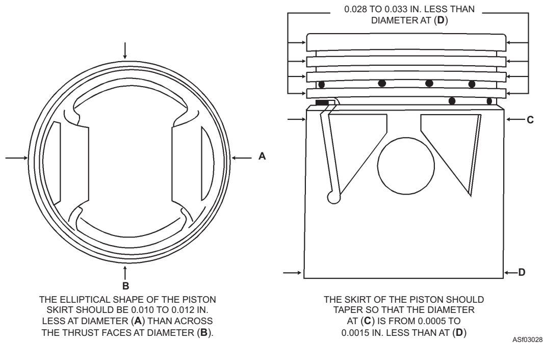
Figure 3-28.—Cam-ground piston.
