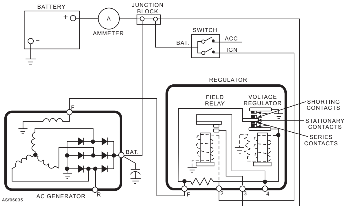
Figure 6-35.—Ac charging circuit using a vibrating-contact regulator.
