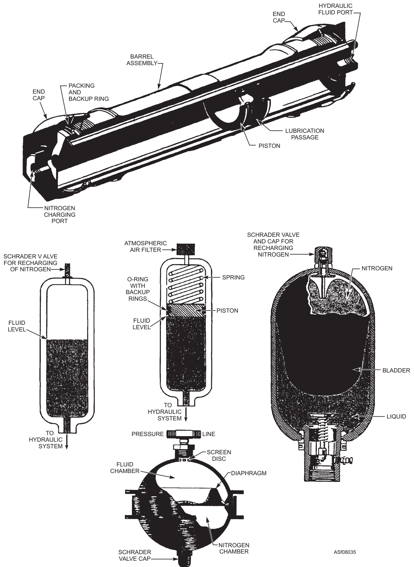
Figure 8-35.—Typical accumulators.
