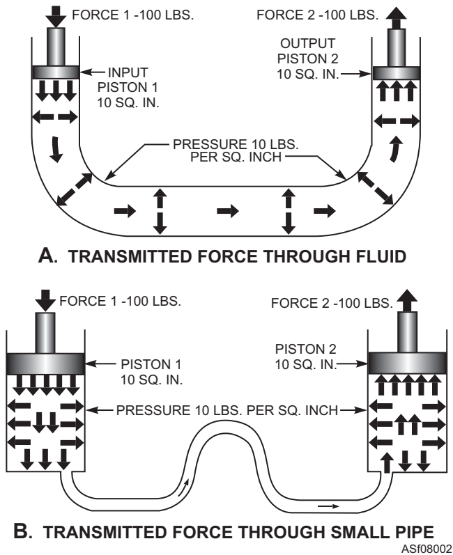
Figure 8-2.—Force transmitted from piston to piston.
