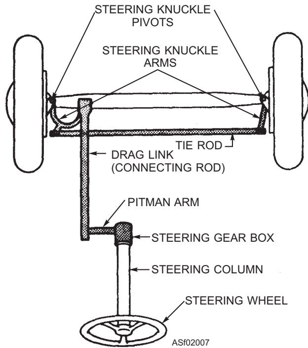
Figure 2-7.—Diagram of a steering mechanism.
