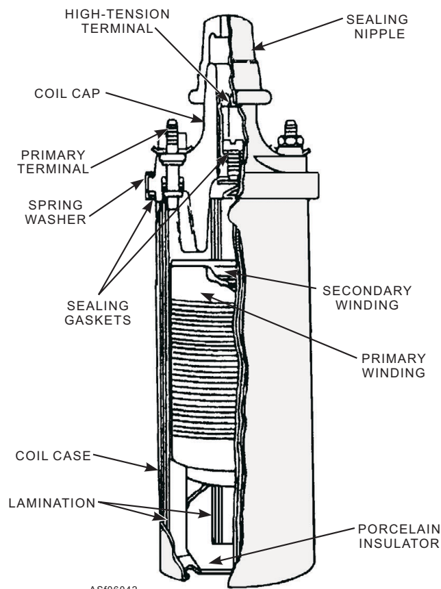
Figure 6-42.—Cutaway view of an ignition coil.
