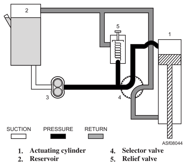
Figure 8-44.—Hydraulic system with a relief valve incorporated.
