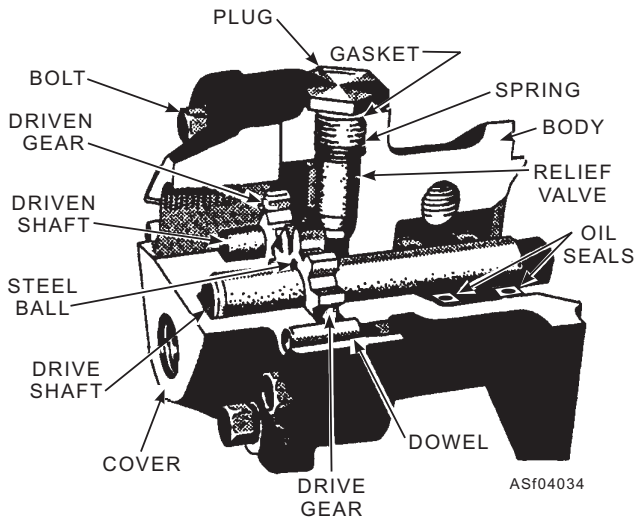
Figure 4-34.—Typical gear fuel pump assembly.
