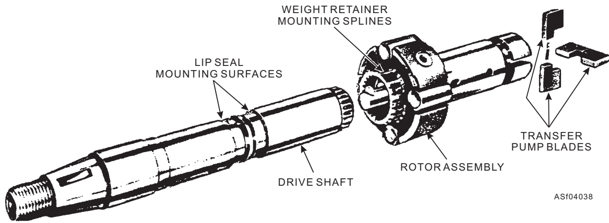
Figure 4-38.—Pump rotating parts (Model DC).
