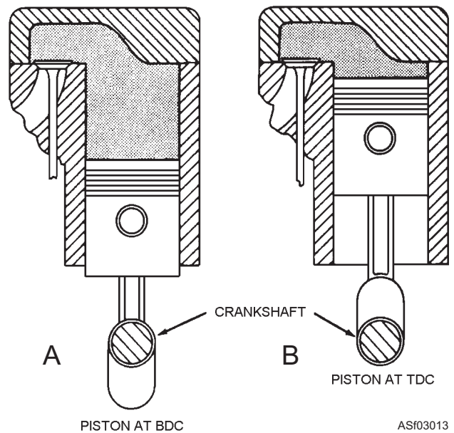
Figure 3-13.—Compression ratio is ratio between views (A) and (B).
