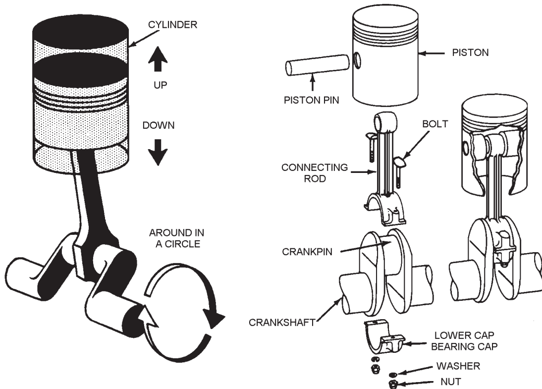
Figure 3-2.—Cylinder, piston, connecting rod, and crankshaft for a 1-cylinder engine.
