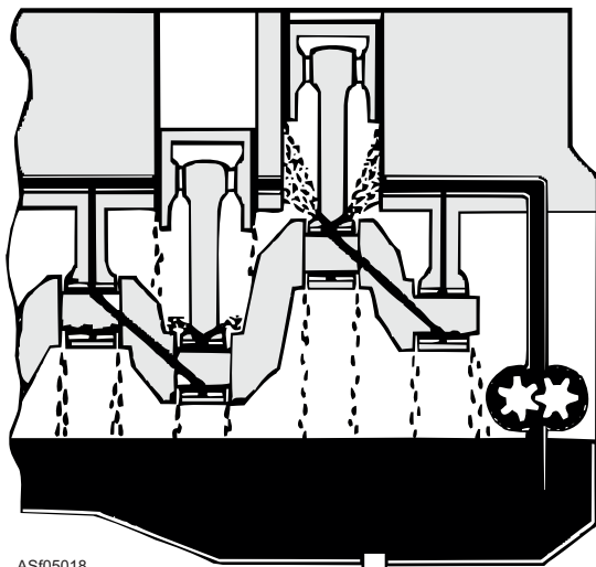
Figure 5-18.—Force-feed lubrication system.
