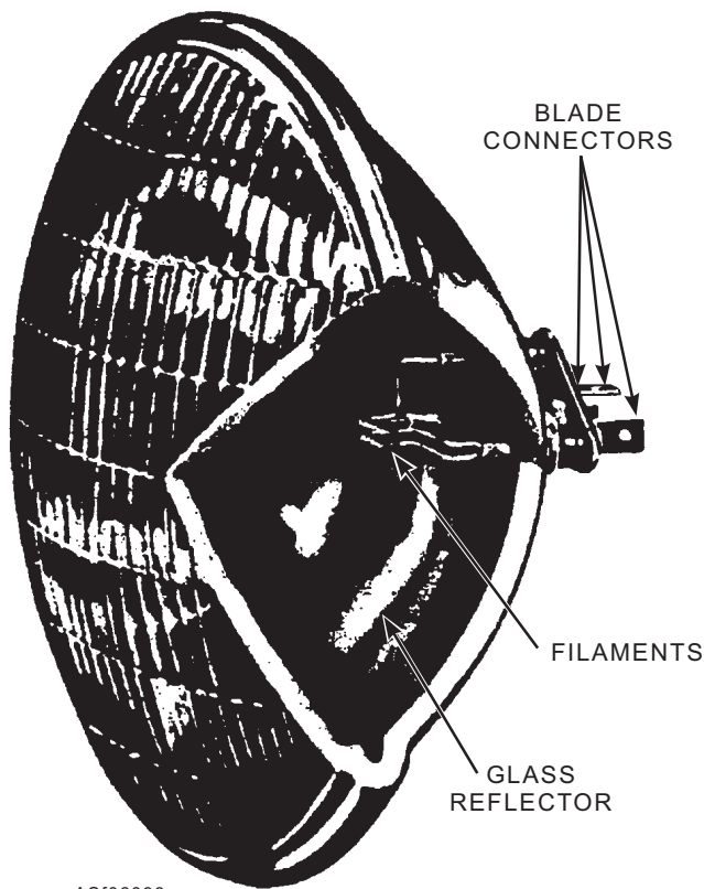
Figure 6-93.—Cutaway view of a sealed beam headlight.
