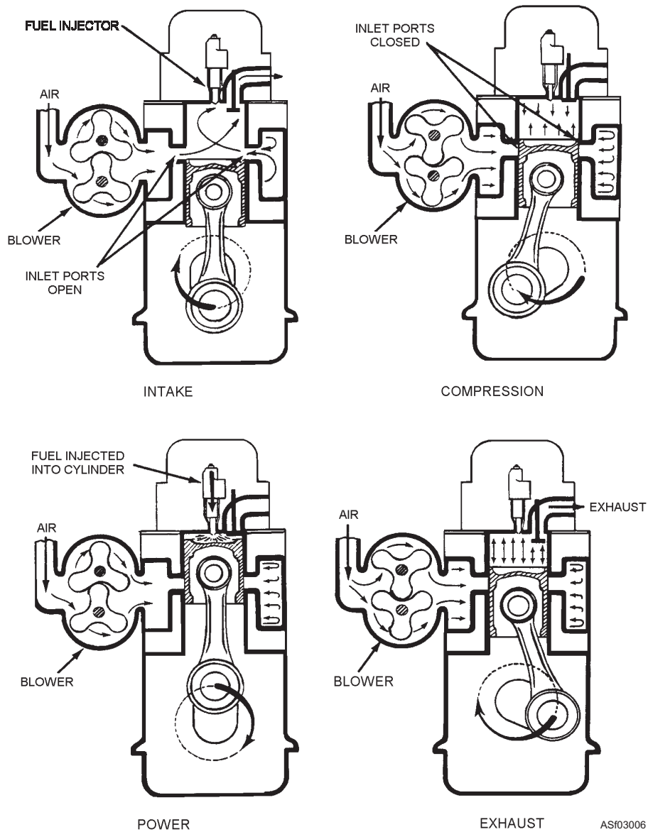
Figure 3-6.—Two-stroke cycle in a diesel engine.
