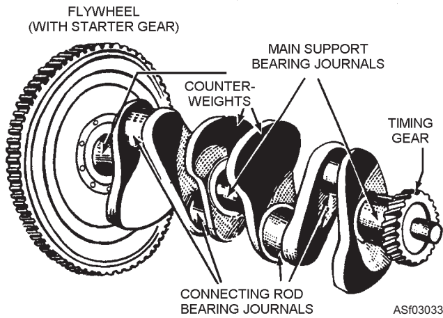
Figure 3-33.—Crankshaft of a 4-cylinder engine.
