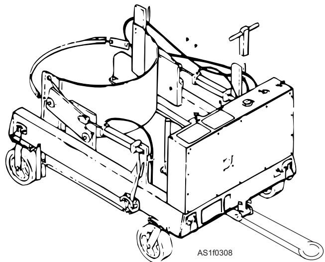
Figure 1-10.—A/M27M-10 hydraulic fluid dispensing unit.
