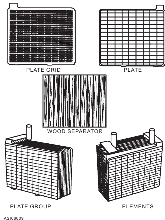
Figure 6-9.—Cell element construction.
