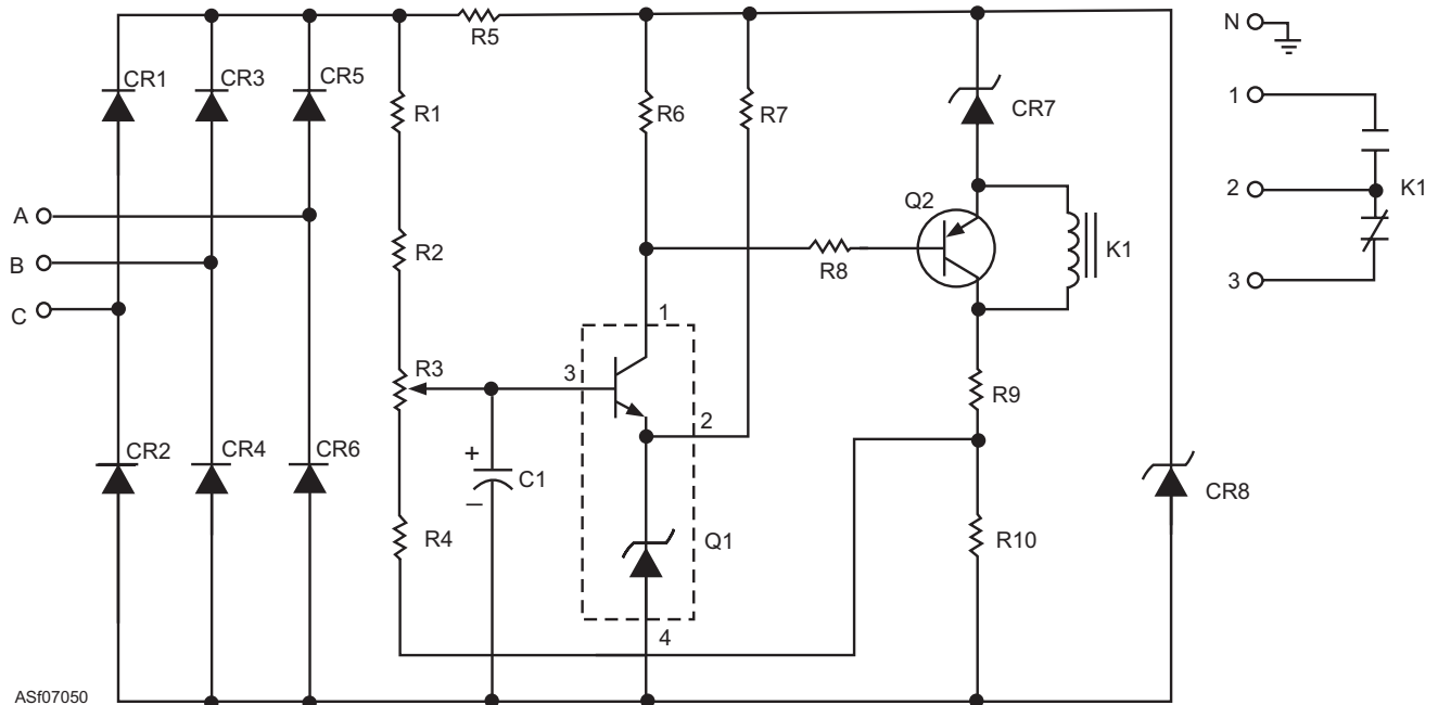
Figure 7-50.—Ac overvoltage relay, simplified schematic.
