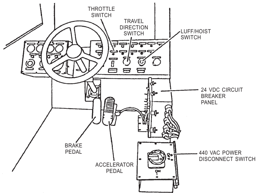
Figure 13-2.—Operator's cab.
