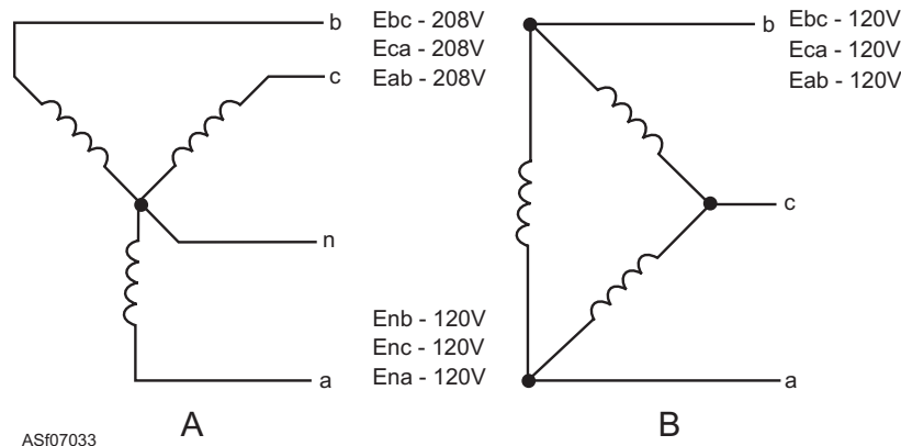
Figure 7-33.—Wye-delta voltage relationships.
