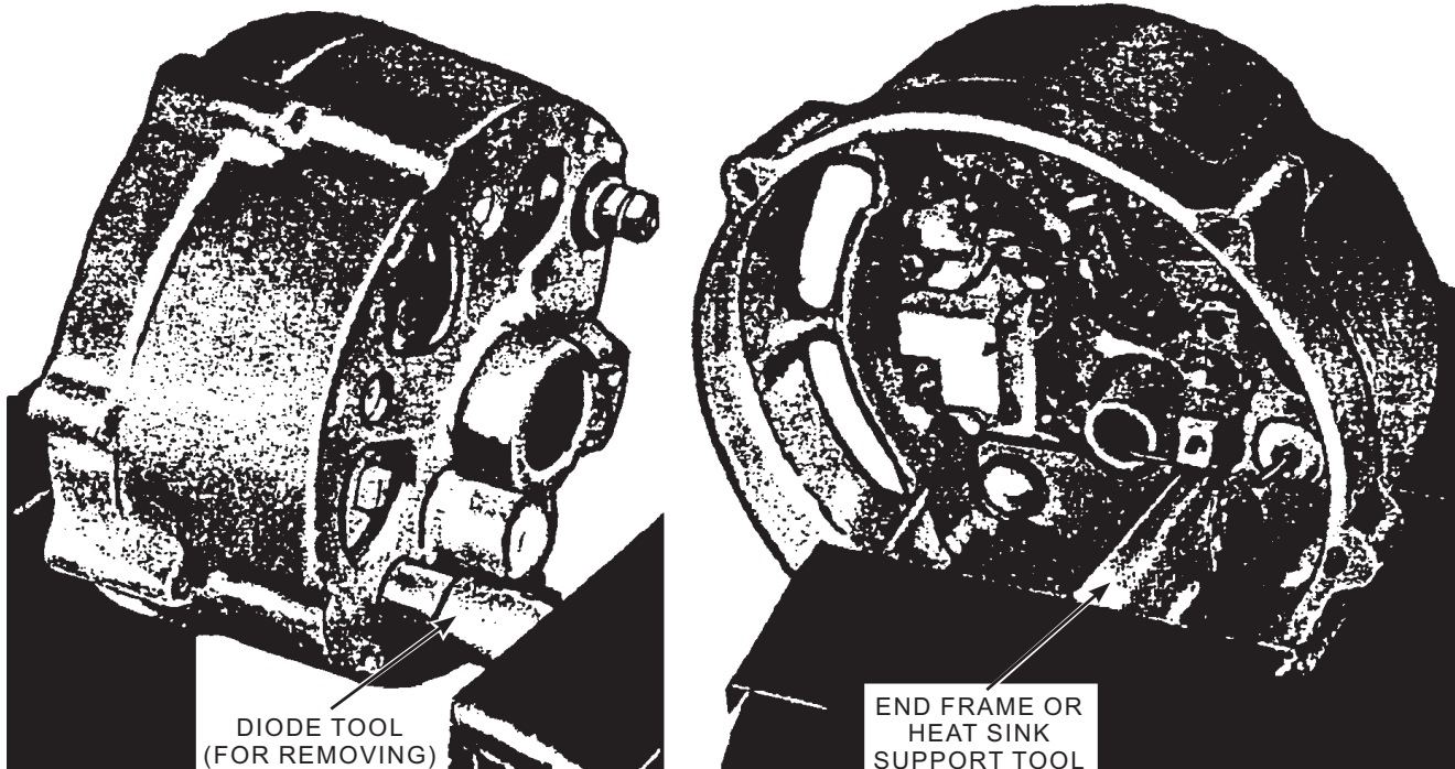
Figure 6-30.—Removing diodes.
