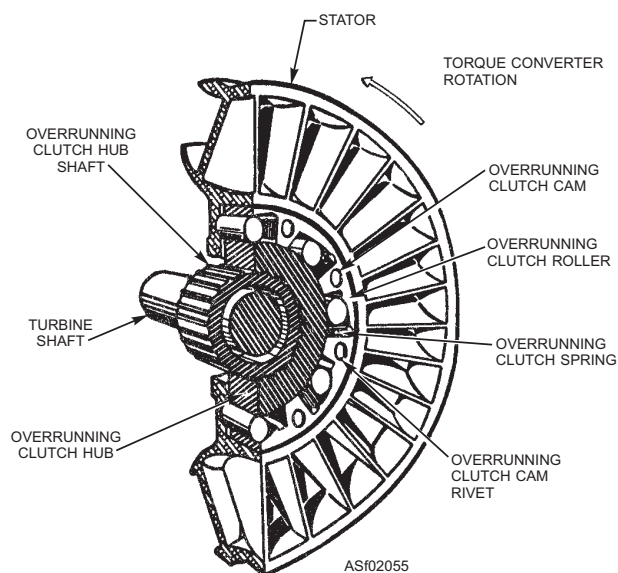
Figure 2-55.—Roller-type overrunning clutch.
