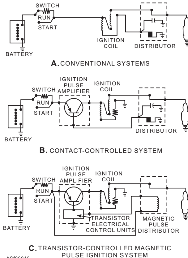
Figure 6-46.—Comparison of the three basic ignition systems.
