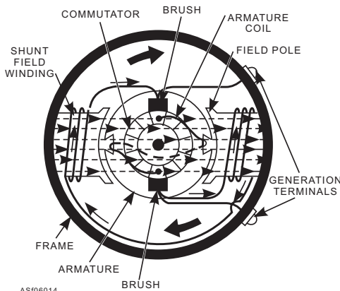
Figure 6-14.—A shunt-wound generator.
