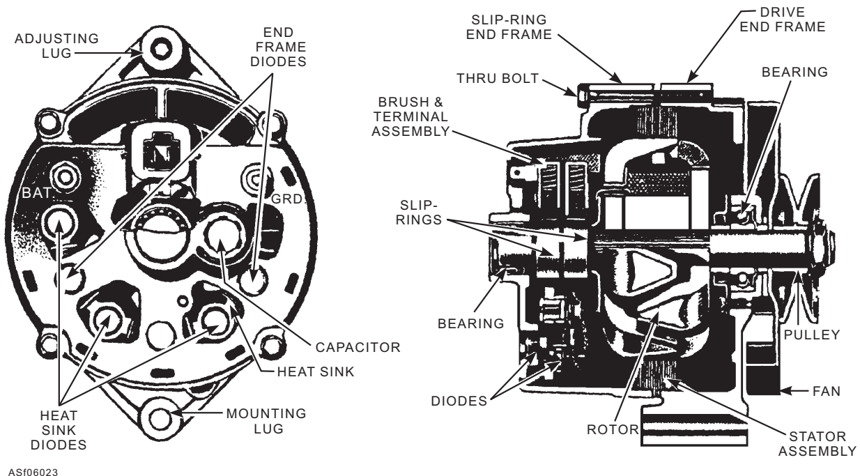
Figure 6-23.—An alternator.
