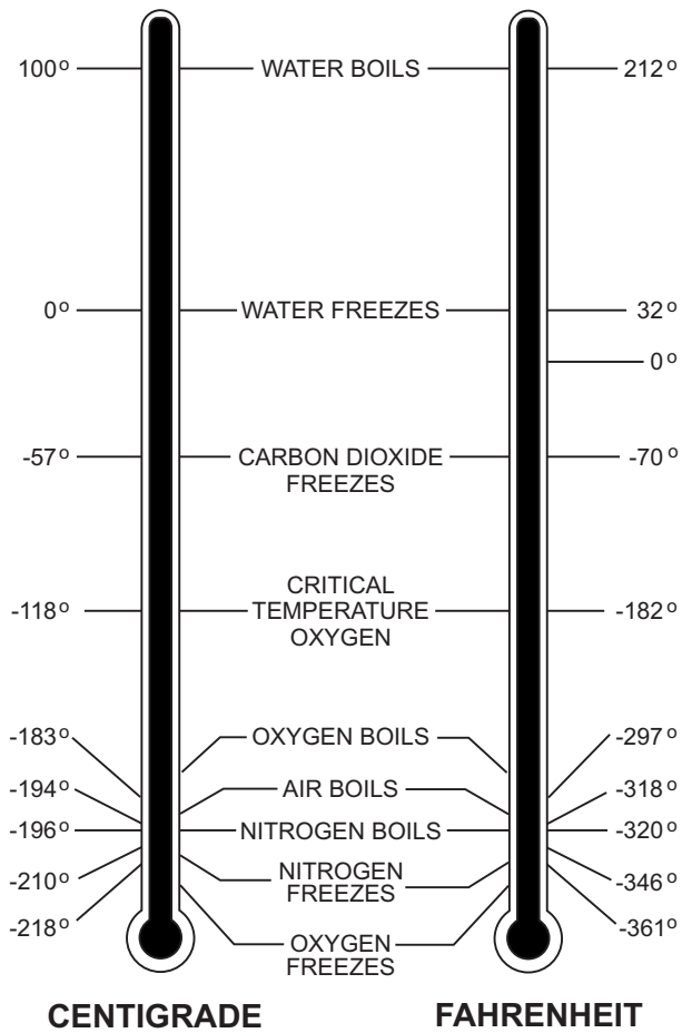
Figure 10-1.—Comparative temperature chart. ASF10001
