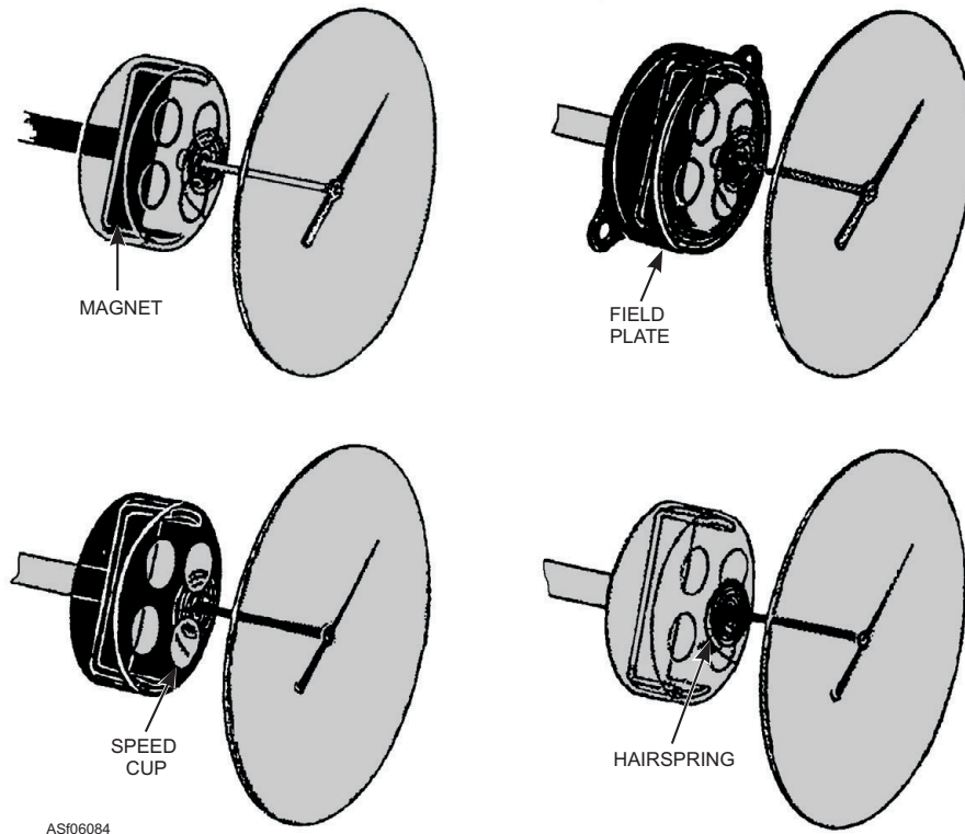
Figure 6-84.—Sectional view of indicating portion of the speedometer.
