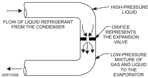
Figure 11-9.—Expansion valve principle.
