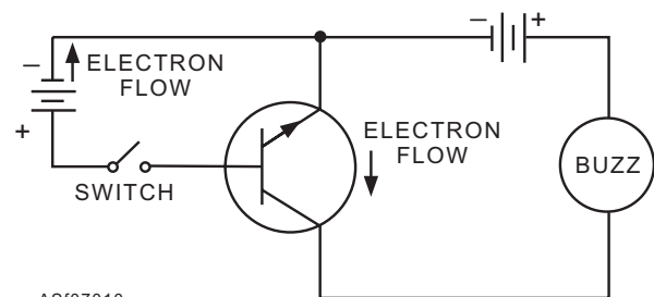
Figure 7-10.—Simple circuit using a transistor as a switch.
