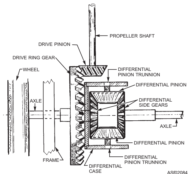
Figure 2-84.—Rear axles and differential.
