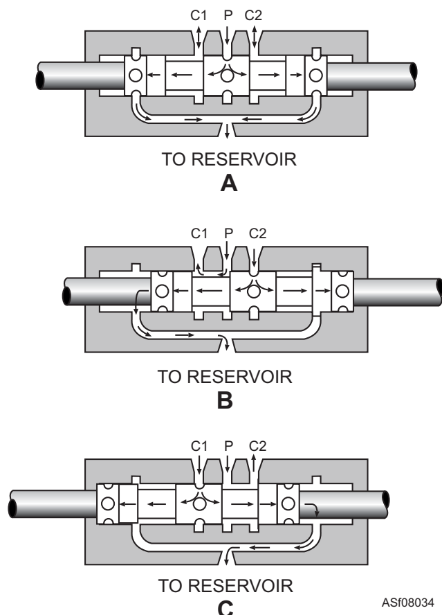
Figure 8-34.—Open-center directional control valve.
