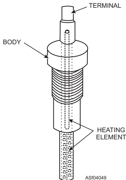
Figure 4-49.—Glow plug.
