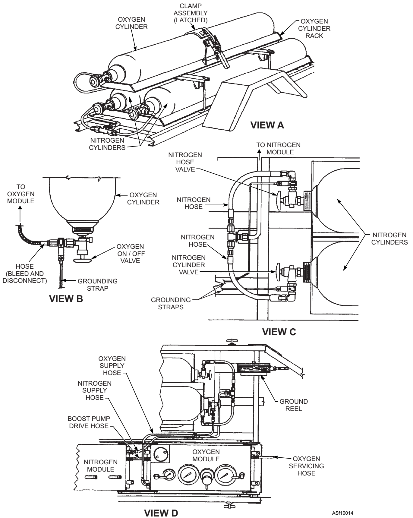
Figure 10-14.—A/U26U-1 gas storage system.
