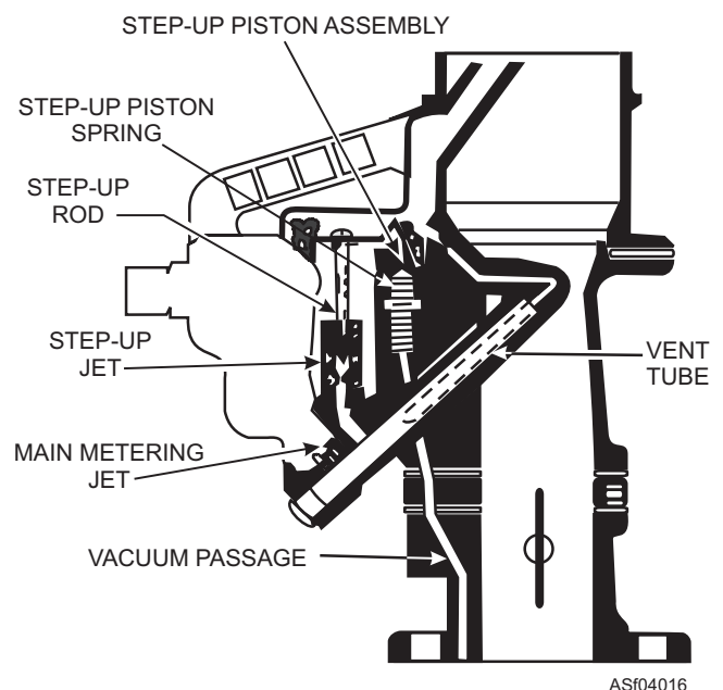
Figure 4-16.—Vacuum set-up high-speed circuit.
