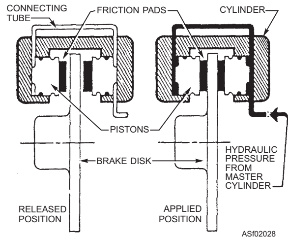
Figure 2-28.—Sectional view of a disc brake in released and applied position.
