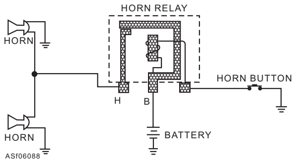
Figure 6-88.—Dual horns and relay circuit.
