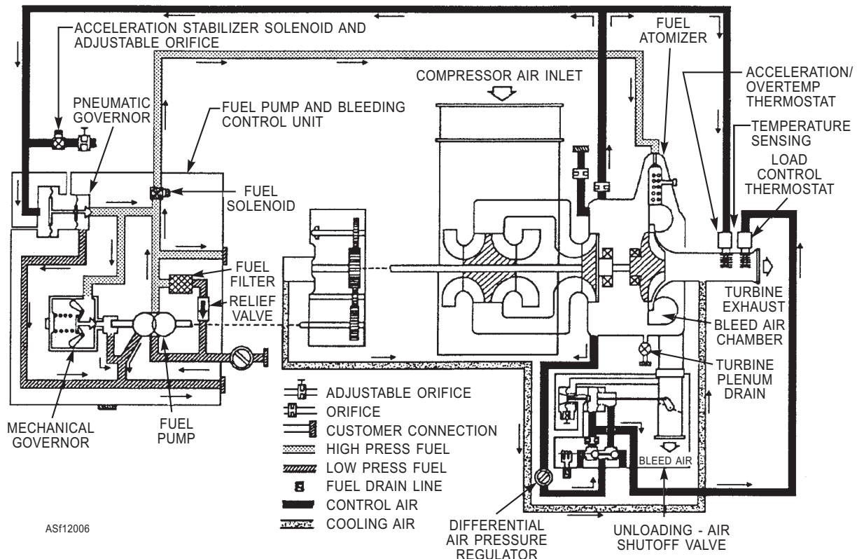
Figure 12-6.—Fuel and bleed-air control system.
