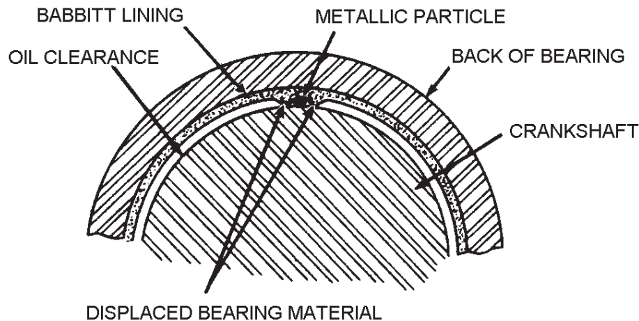
ASf03060 Figure 3-60.—Effect of a metallic particle embedded in bearing material (Babbitt lining).
