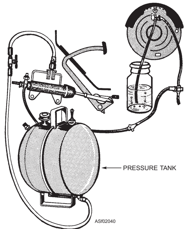
Figure 2-40.—Bleeding hydraulic system—pressure method.
