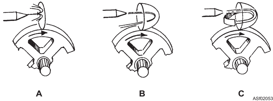
Figure 2-53.—Effects of oil jetstream on a flat surface and on a curved surface.
