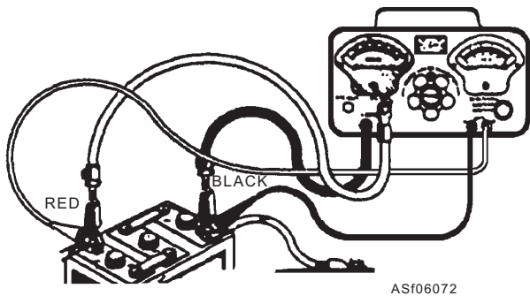
Figure 6-72.—Tester connections for a battery capacity test.
