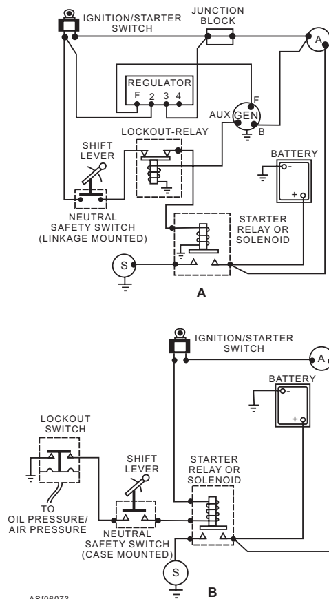
Figure 6-73.—Voltmeter connections for checking starting system circuit resistance.
