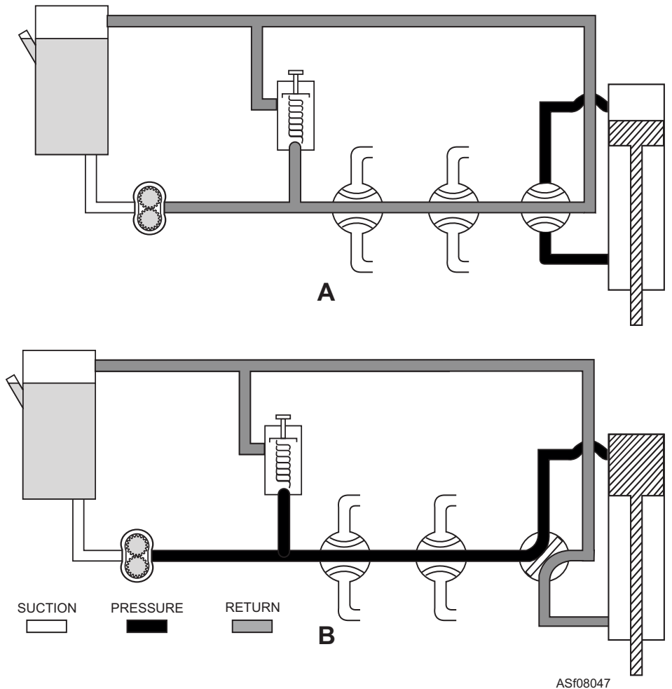
Figure 8-47.—Basic open-center system.
