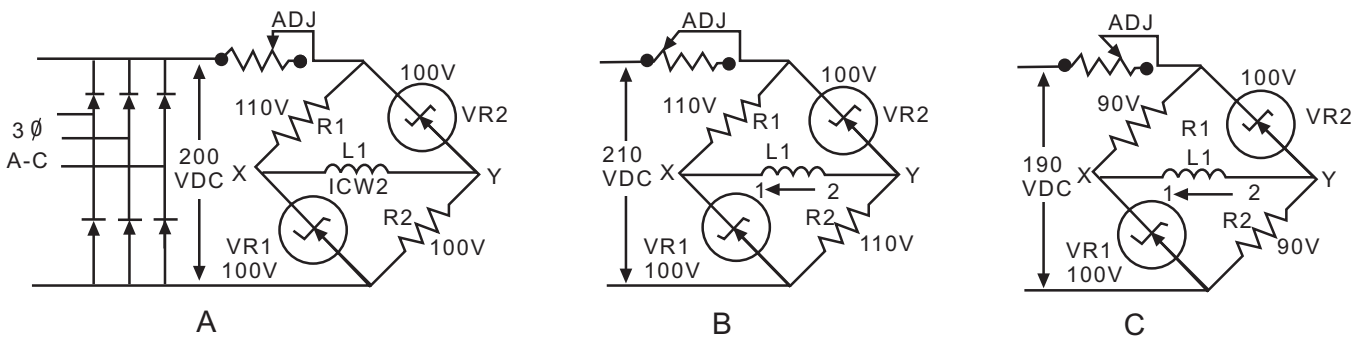
Figure 7-20.—Views of line voltage-sensing bridge (BRDG).
