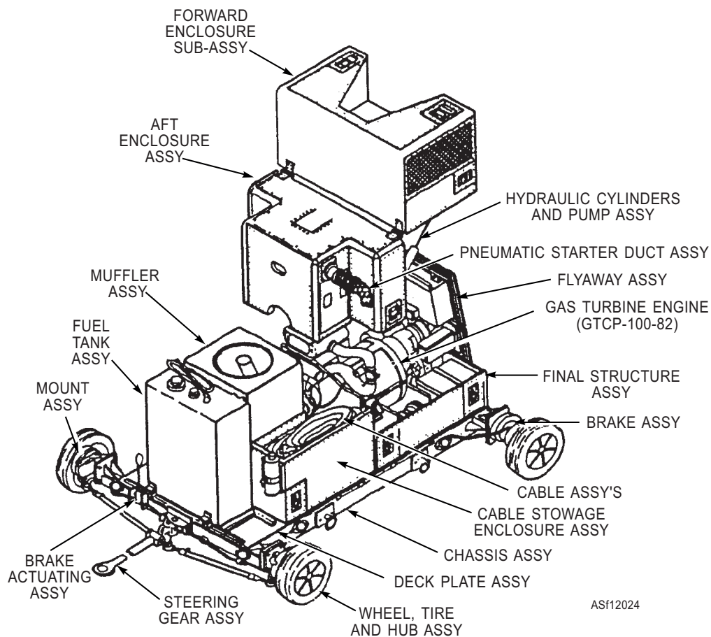
Figure 12-24.—Model A/M47A-4 compressor power unit.
