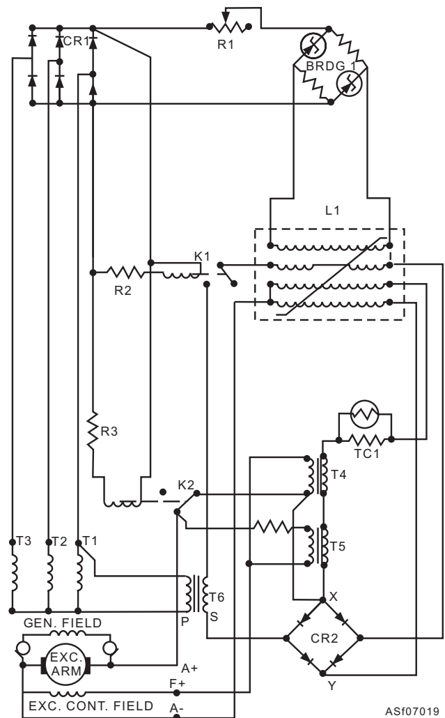
Figure 7-19.—Typical solid-state regulator.
