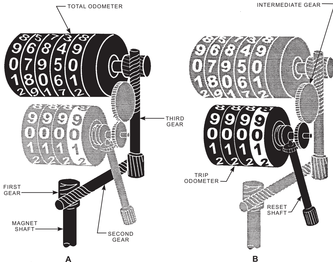
Figure 6-85.—(A) Total odometer; (B) Trip odometer.
