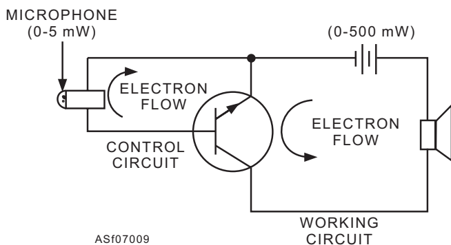
Figure 7-9.—Basic amplifying circuit.
