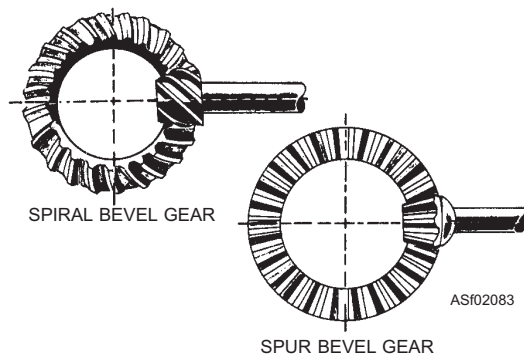
Figure 2-83.—Ring gear and pinion.
