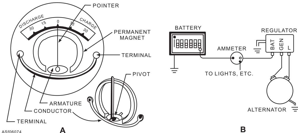
Figure 6-74.—(A) Simplified automotive ammeter; (B) Wiring diagram showing ammeter in the charging circuit.
