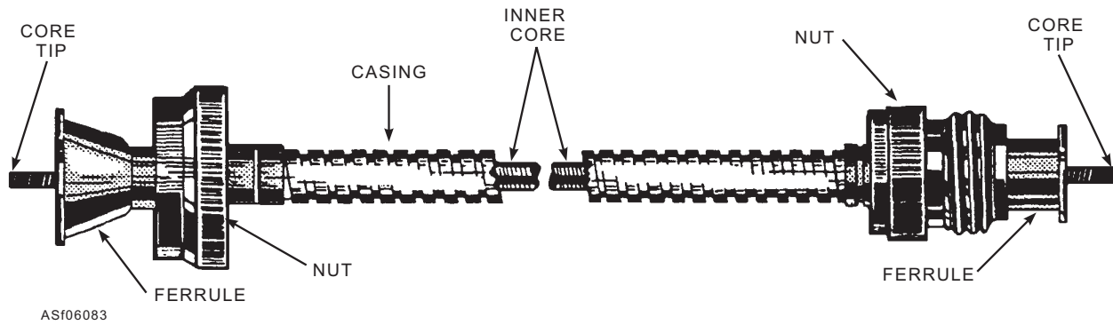
Figure 6-83.—Speedometer and tachometer drive shaft.
