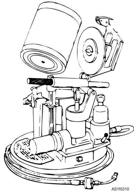
Figure 1-12.—H-250-1 hydraulic fill unit.
