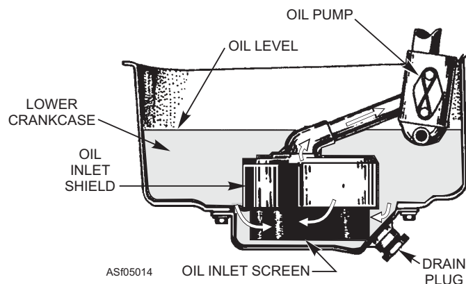
Figure 5-14.—Fixed oil strainer.
