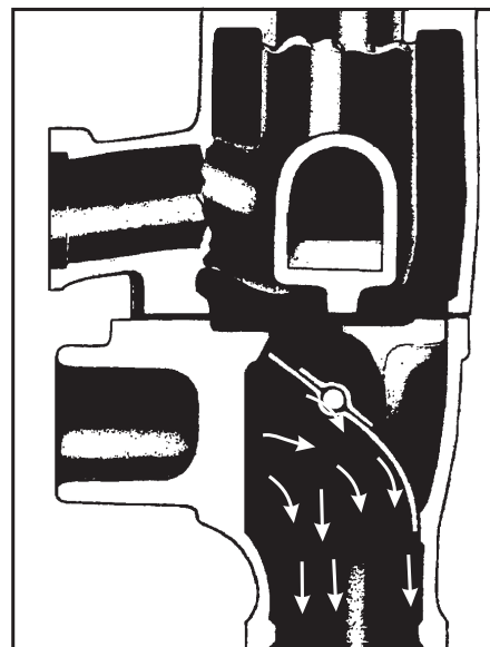
Figure 4-24.—Flow of exhaust gases around intake manifold.
