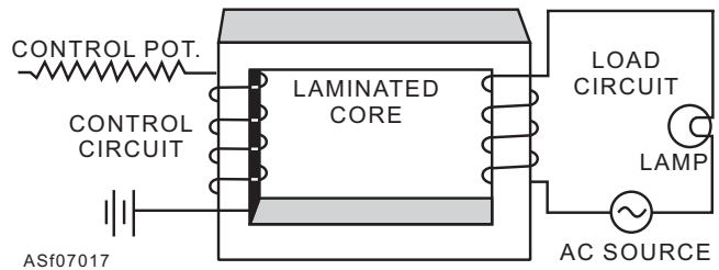
Figure 7-17.—A basic magnetic amplifier.
