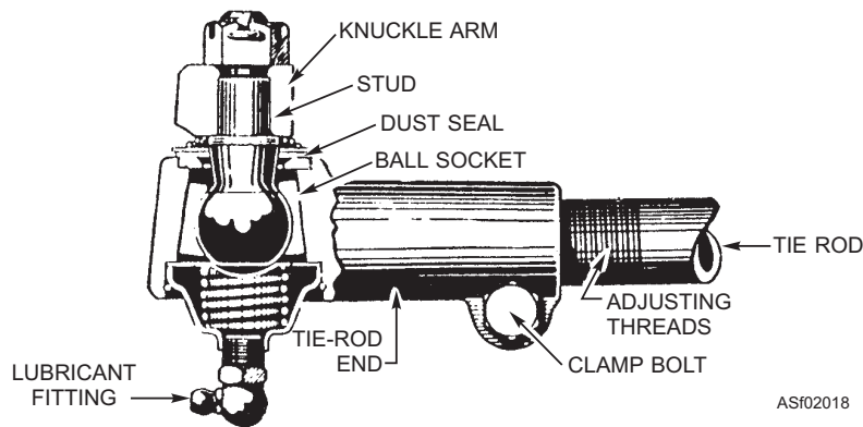
Figure 2-18.—Tie rod end showing clamp bolt and adjusting threads.
