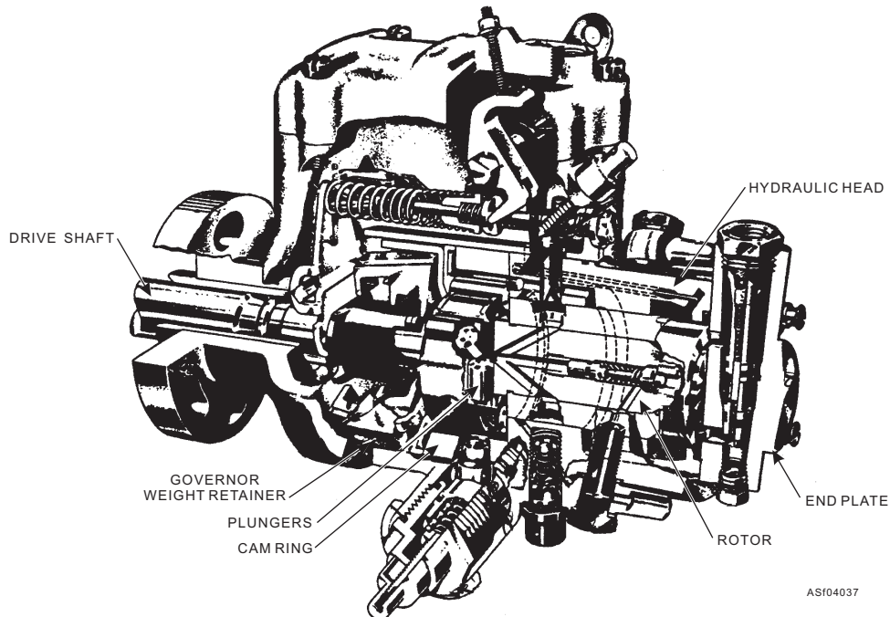
Figure 4-37.—Roosa Master fuel injection pump (Model DC).
