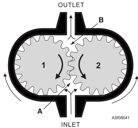
Figure 8-41.—Gear-type motor.
