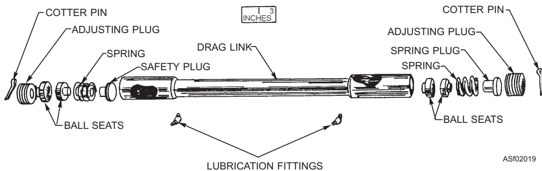
Figure 2-19.—Drag link assembly—exploded view.
