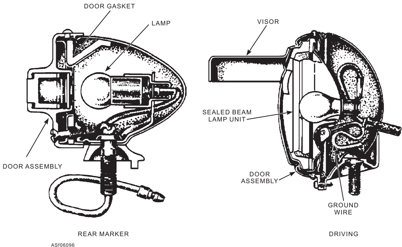
Figure 6-96.—Rear marker and blackout driving lights.
