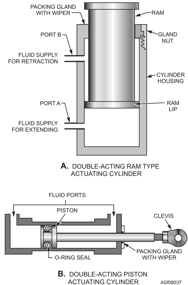
Figure 8-37.—Typical cross-sectional view of a double-acting actuating cylinder.
