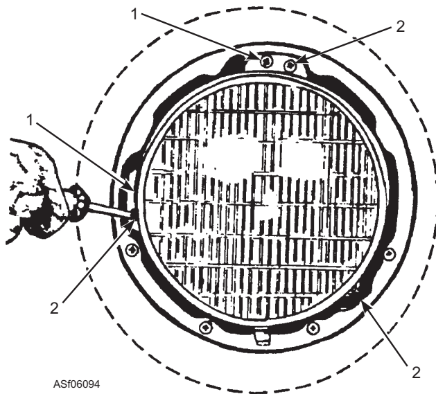
Figure 6-94.—Sealed beam headlight installation.
