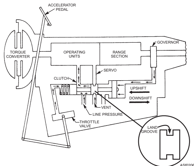
Figure 2-69.—Shift valve.
