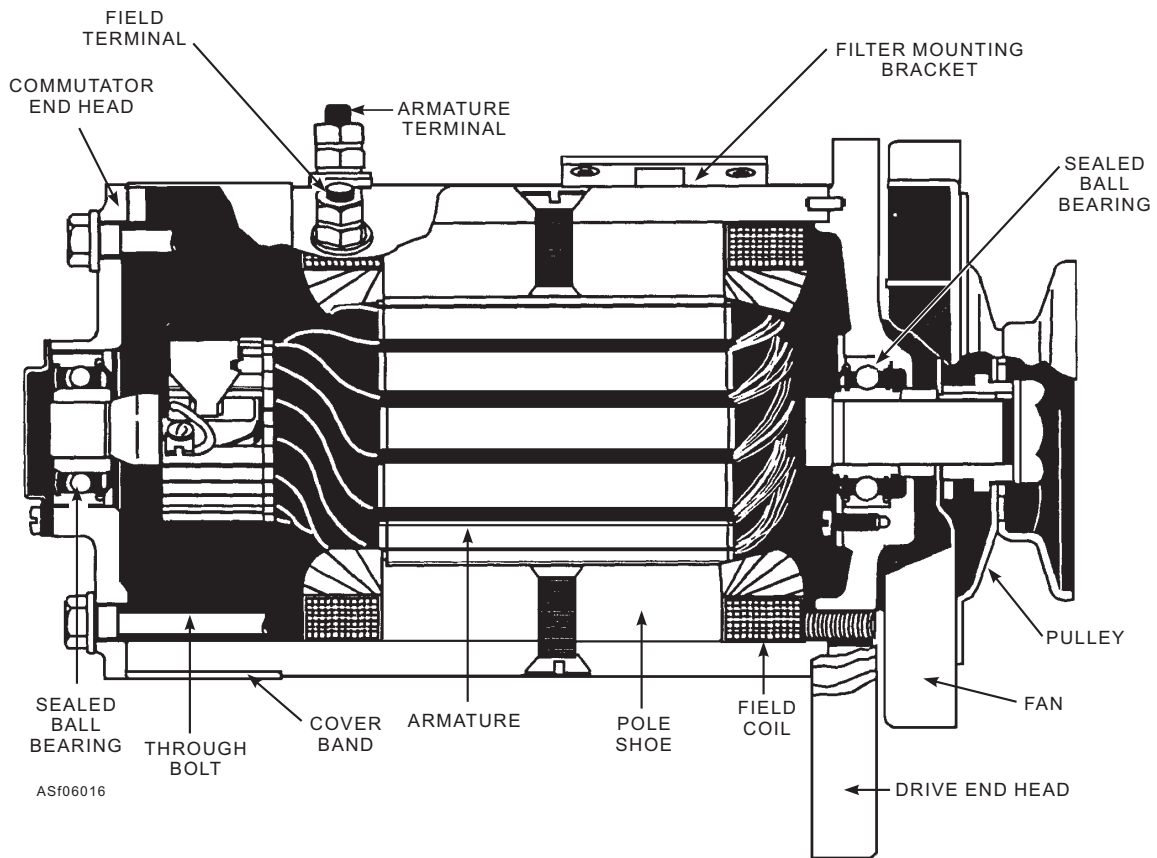
Figure 6-16.—Sectional view of dc generator.
