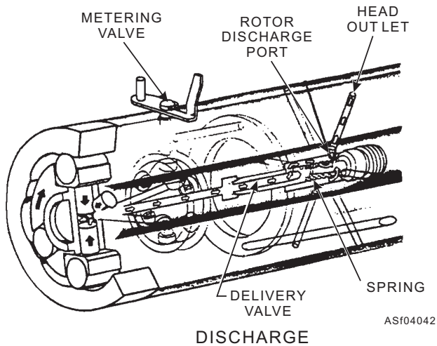
Figure 4-42.—Rotor in discharge position (DC pump).
