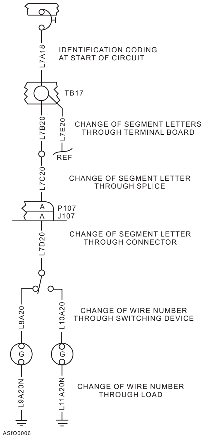
Figure 6-6.—Example of wire identification code use.
