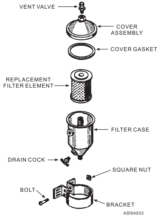
Figure 4-33.—Fuel filter assembly with replaceable element.
