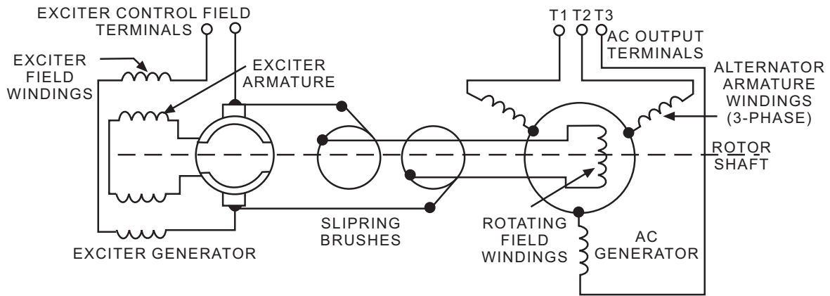
A TYPICAL AC GENERATOR (SCHEMATIC)
