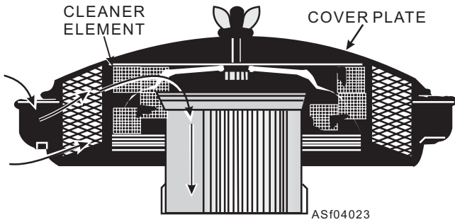
Figure 4-23.—Dry-type air cleaner.
