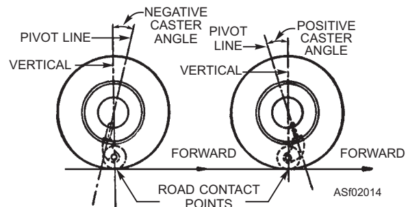
Figure 2-14.—A. Negative caster; B. positive caster.
