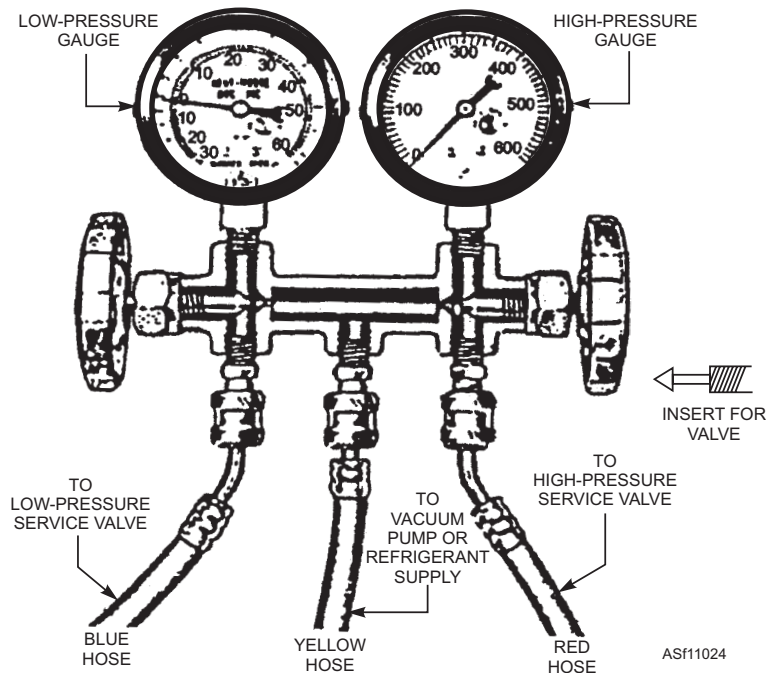
Figure 11-24.—Internal view of refrigerant manifold test set.
