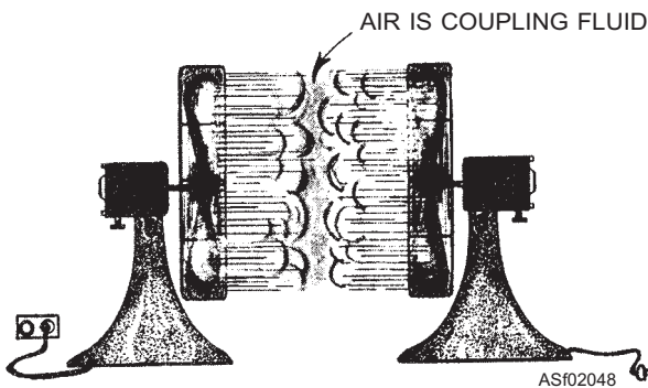
Figure 2-48.—Basic fluid coupling, using air in place of fluid.
