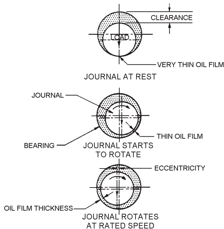
Figure 3-59.—Oil clearance between bearing and shaft.
