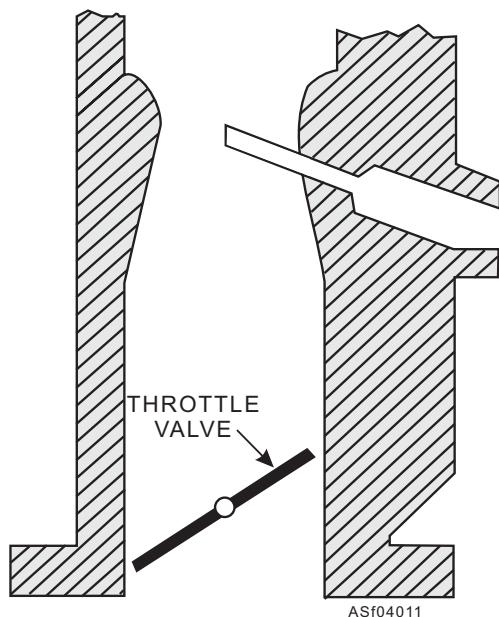
Figure 4-11.—Simplified carburetor with throttle valve.
