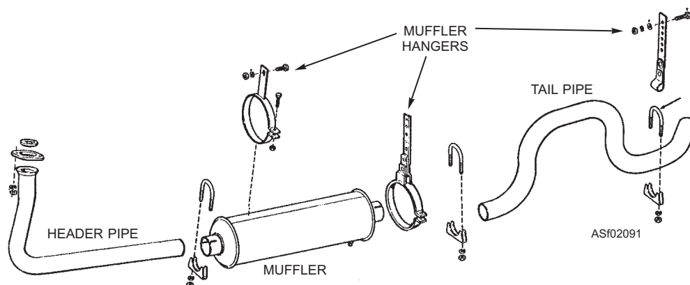
Figure 2-91.—Typical exhaust system.
