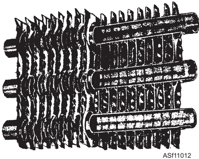
Figure 11-12.—Construction detail of an evaporator.
