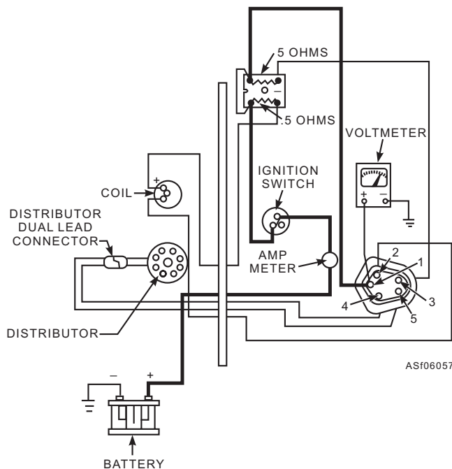
Figure 6-57.—Harness connector No. 1 test.
