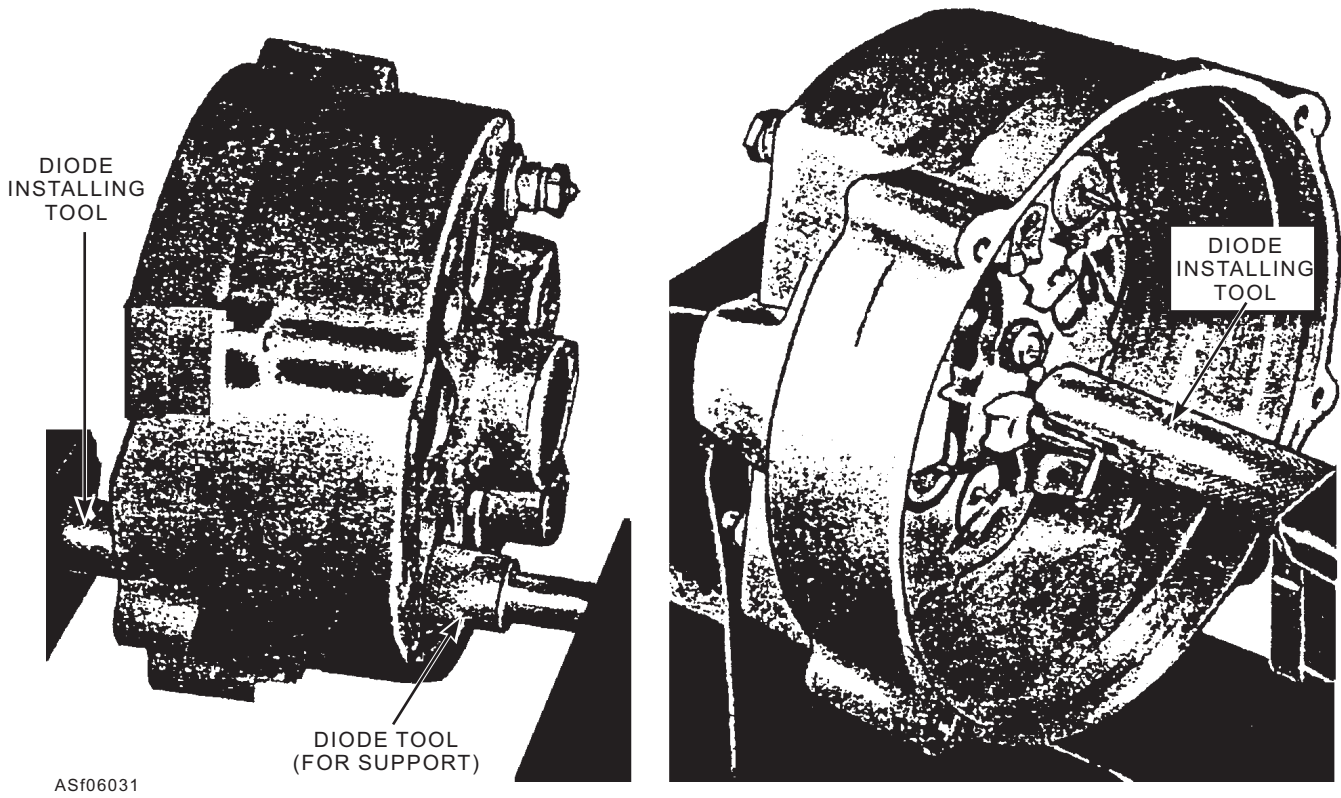
Figure 6-31.—Installing diodes.
