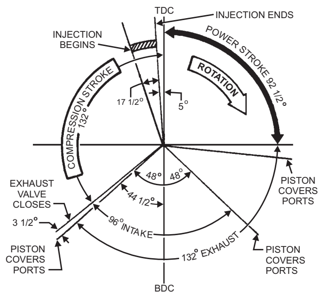
2-STROKE VALVE TIMING DIAGRAM
