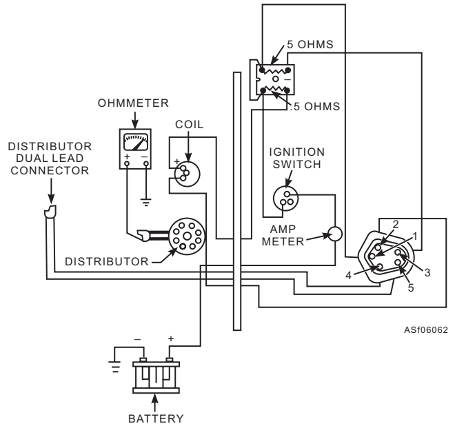
Figure 6-62.—Pickup coil ground test.
