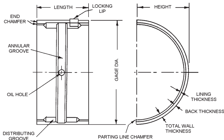
Figure 3-58.—Typical sleeve-type bearing half.
