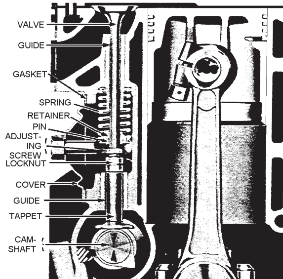
Figure 3-38.—L-head valve operating mechanism.
