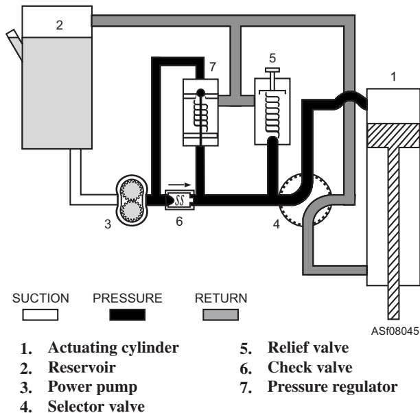
Figure 8-45.—Hydraulic system with a relief valve and regulator incorporated.
