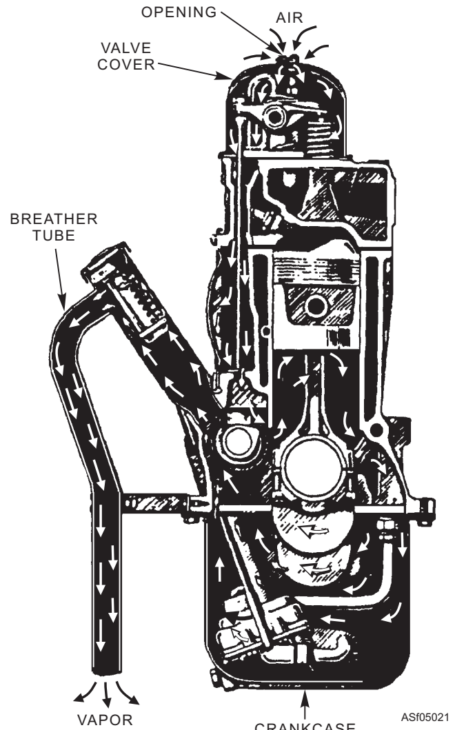
Figure 5-21.—Crankshaft breather tube.
