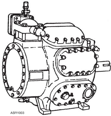
Figure 11-3.—Reciprocating open compressor.
