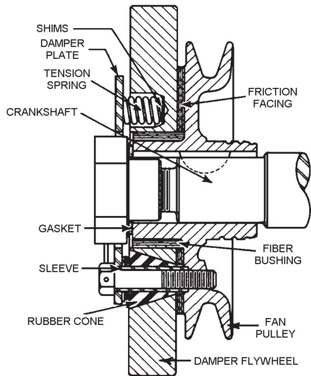
Figure 3-35.—Sectional view of a typical vibration damper.
