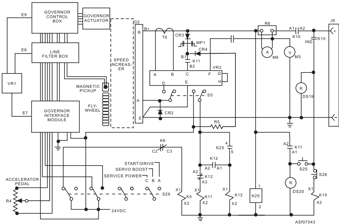
Figure 7-43.—Engine governor and dc power control.
