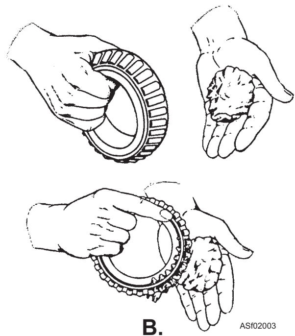
Figure 2-3.—Packing wheel bearings.
