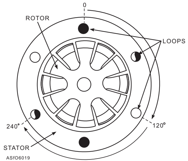
Figure 6-19.—A three-phase alternator.
