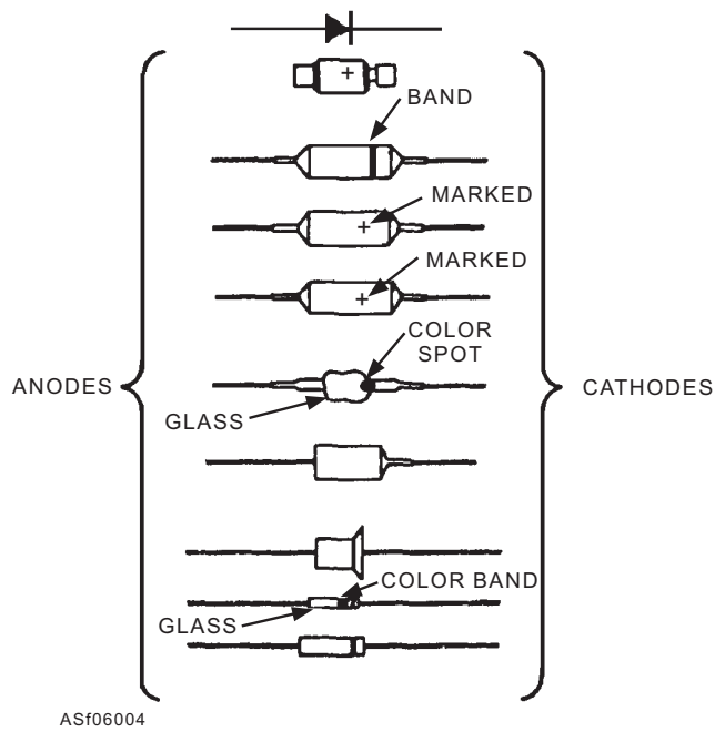
Figure 7-4.—PN diode identification.
