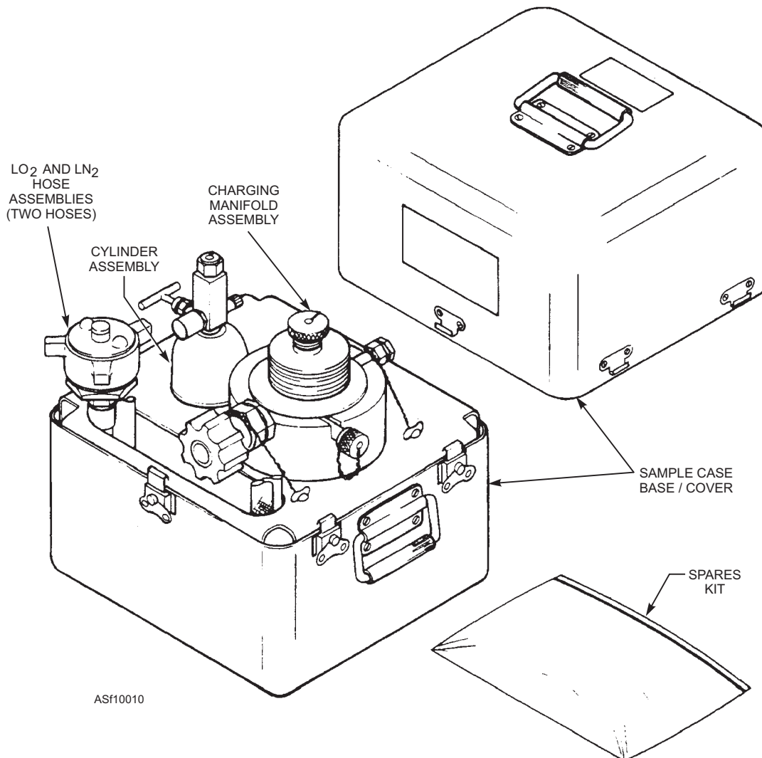
Figure 10-10. —FCS 2001 cryogenic sampler.
