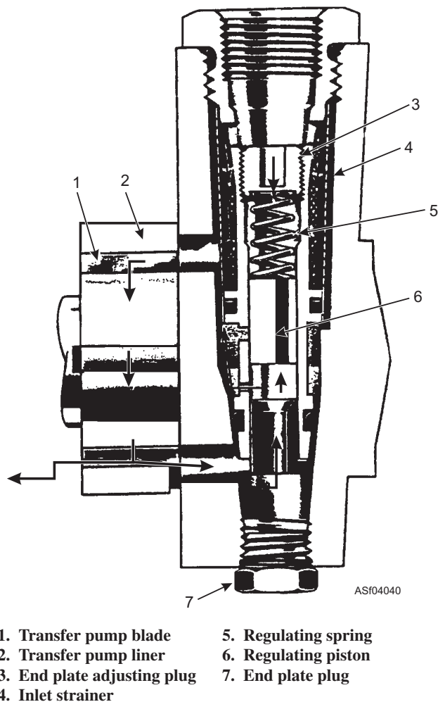
Figure 4-40.—Transfer pump (Model DC).
