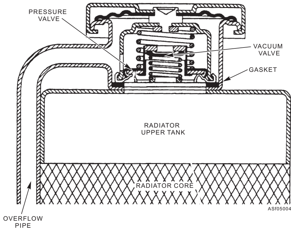
Figure 5-4.—Radiator pressure cap.
