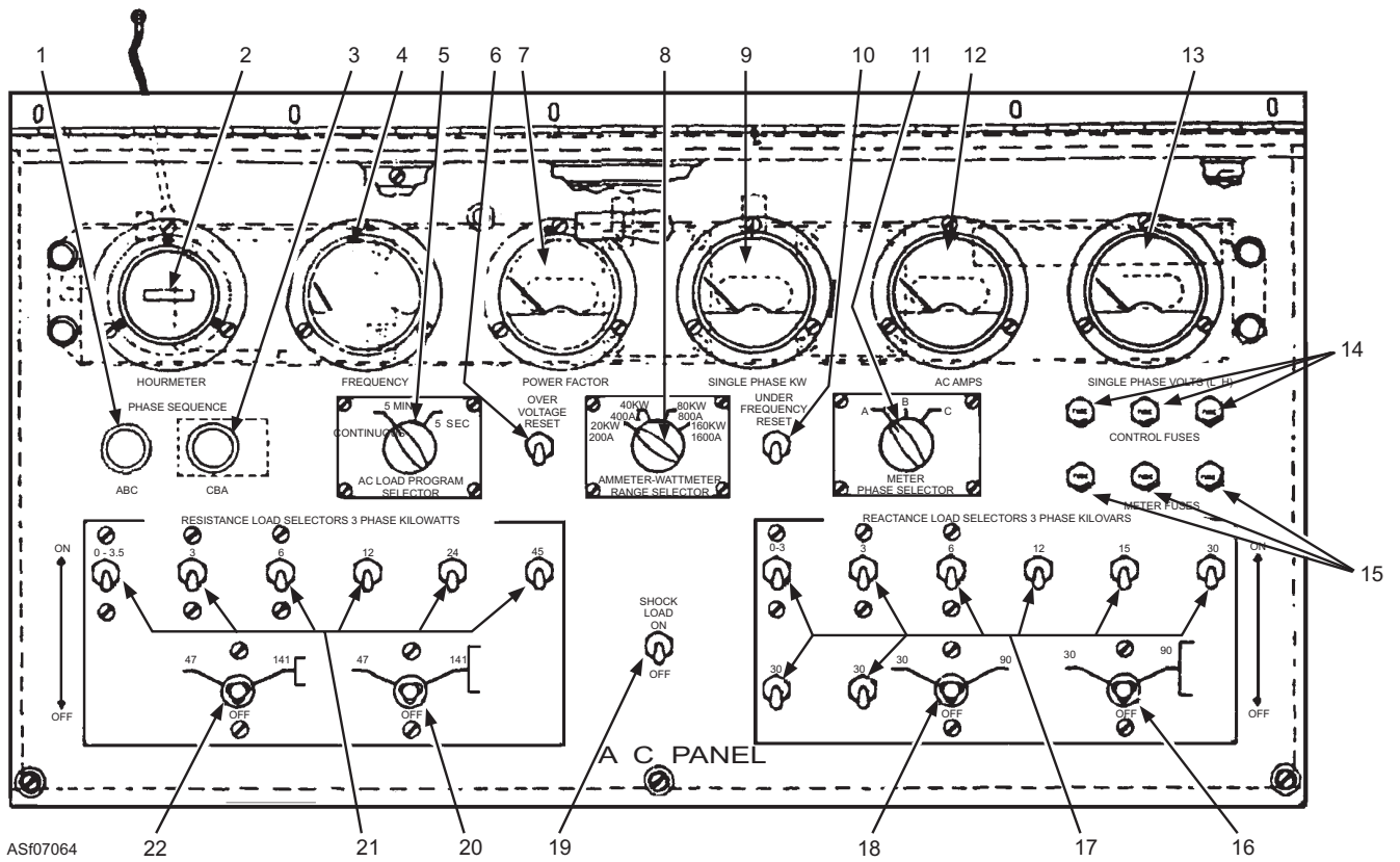
Figure 7-64.—AC control panel.
