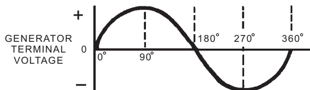
Figure 7-23.—Output voltage of an elementary generator during one revolution.
