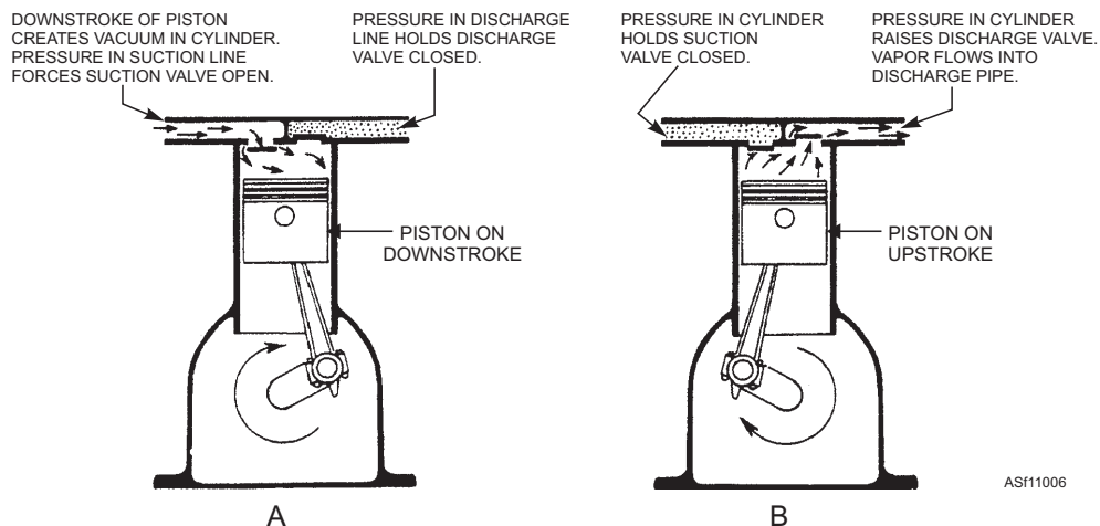
Figure 11-6.—Operating cycle of a reciprocating compressor.
