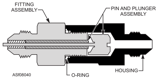
Figure 8-40.—Pressure gauge snubber.
