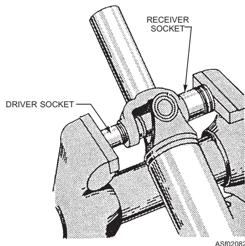
Figure 2-82.—Universal joint removal.
