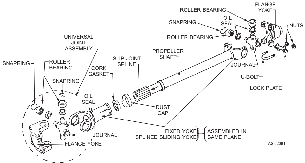
Figure 2-81.—Propeller shaft assembly.
