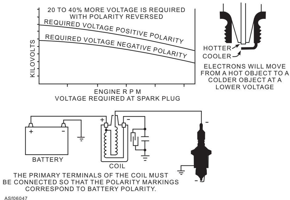
Figure 6-47.—Correct coil polarity and current flow for a negative grounded system.
