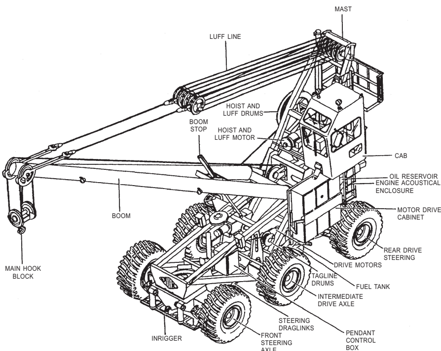
Figure 13-1.—A/S32A-36A amphibious assault crash crane (AACC).
