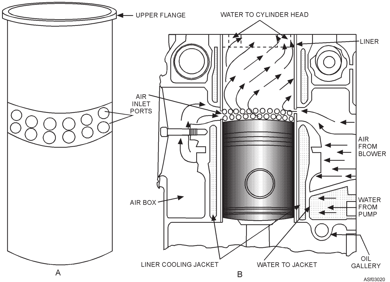
Figure 3-20.—(A) Dry-type liner for 2-cycle General Motors series engines. (B) Section through series 71 block.
