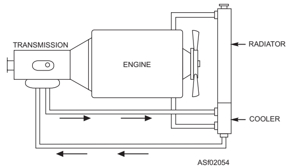
Figure 2-54.—Typical radiator-type oil cooler.
