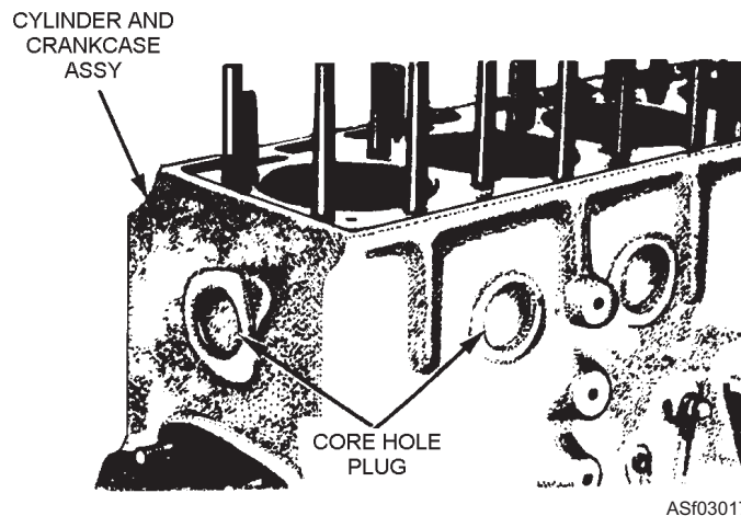
Figure 3-17.—Core hole plugs installed in cylinder block.
