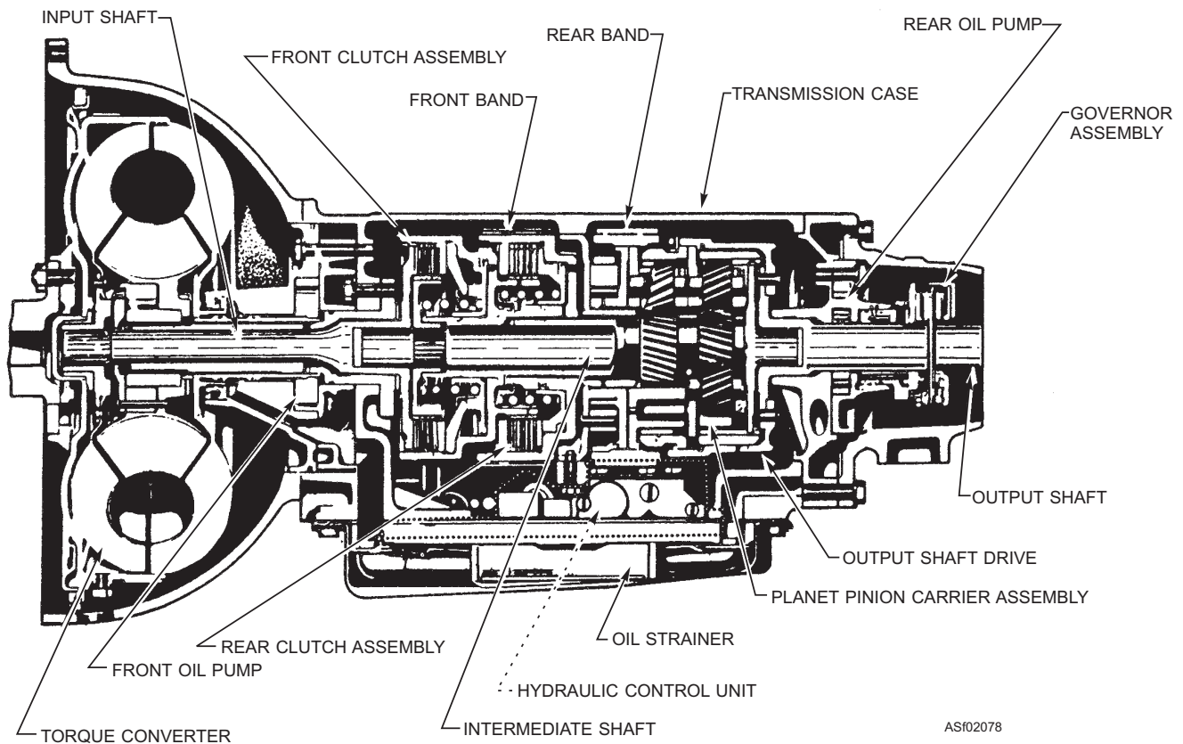
Figure 2-78.—Typical automatic transmission.
