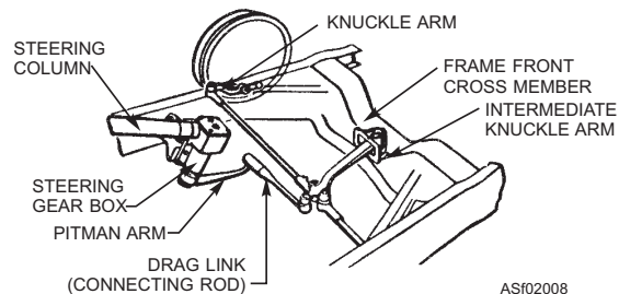
Figure 2-8.—Steering assembly.
