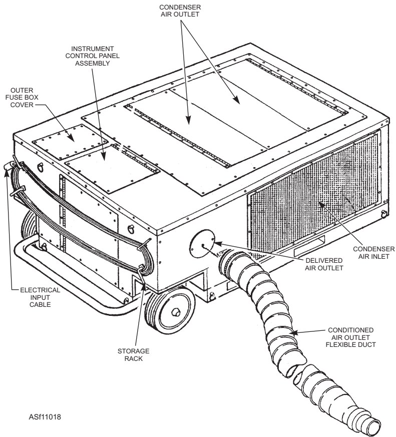
Figure 11-18.—A/M32C-21 trailer-mounted air-conditioning unit, electric-powered.
