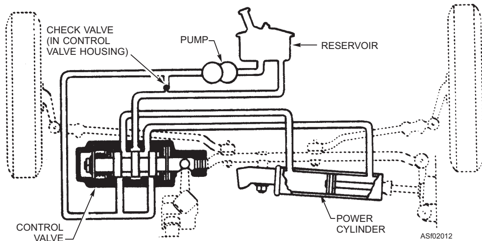
Figure 2-12.—Power steering system.
