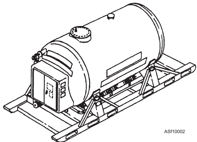
Figure 10-2.—2,000 gallon capacity liquid oxygen storage tank. ASF10002
