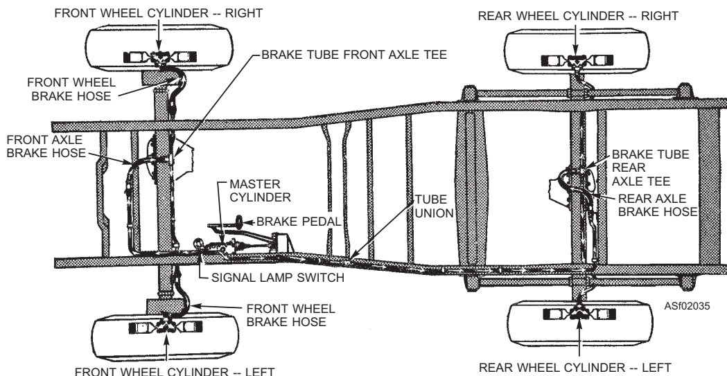
Figure 2-35.—Typical hydraulic brake system.
