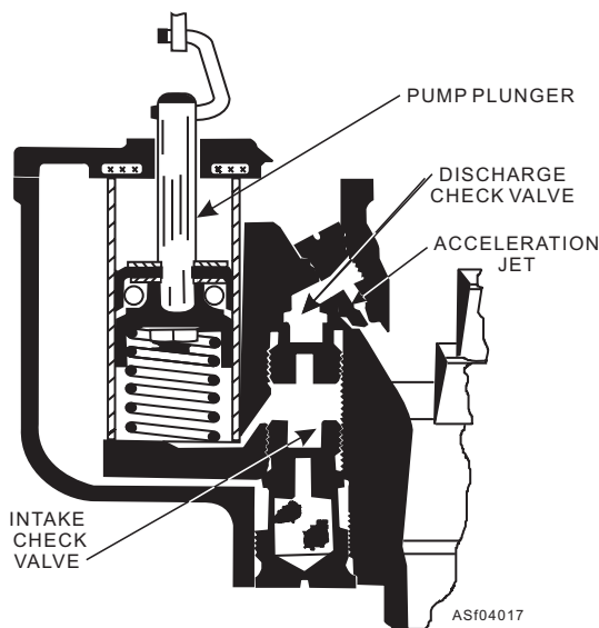
Figure 4-17.—Carburetor accelerator pump circuit.
