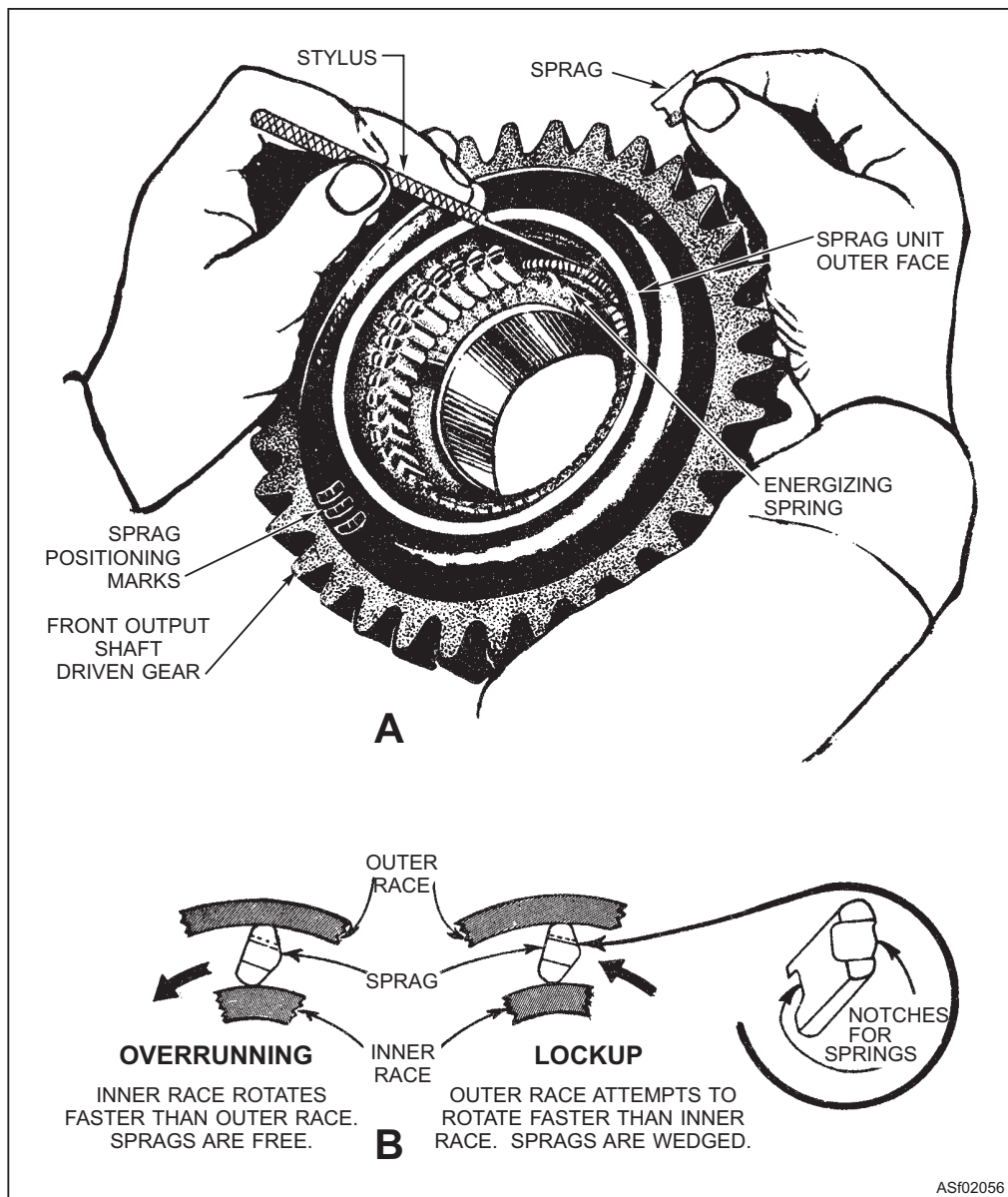
Figure 2-56.—Typical sprag assembly, overrunning clutch.
