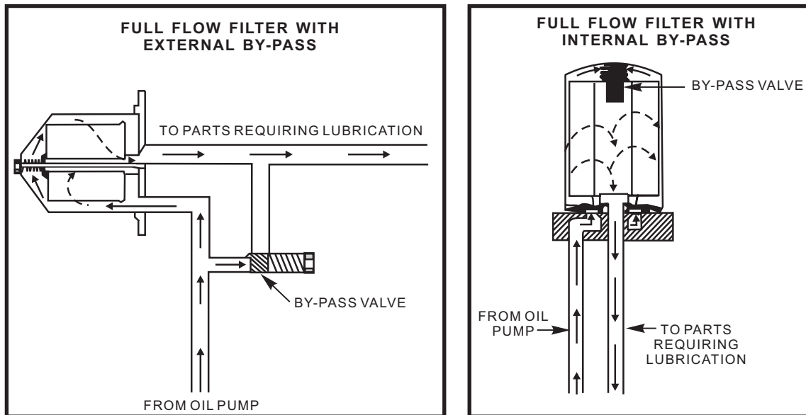
Figure 5-15.—Full flow filters.
