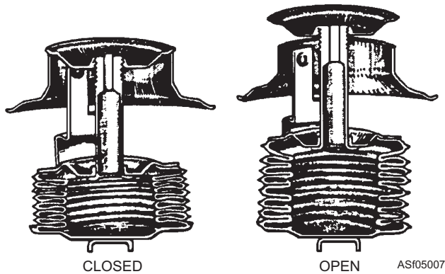
Figure 5-7.—Bellows thermostat.
