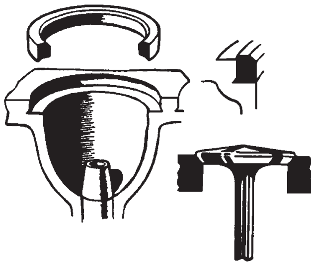
Figure 3-44.—Valve seat insert.
