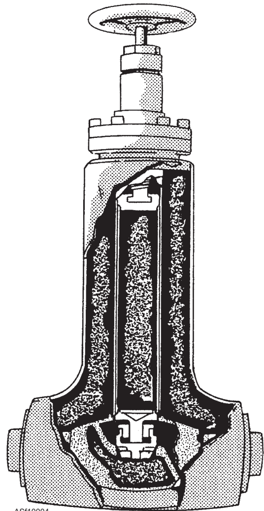
Figure 10-4.—Vacuum insulated cryogenic globe valve.
