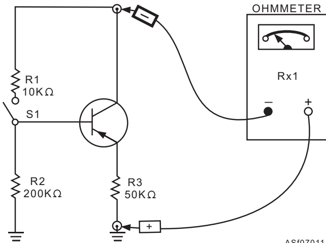
Figure 7-11.—Testing a transistor's gain with an ohmmeter.
