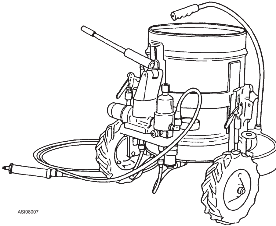
Figure 8-7.—Fluid Service Cart, Model 310.
