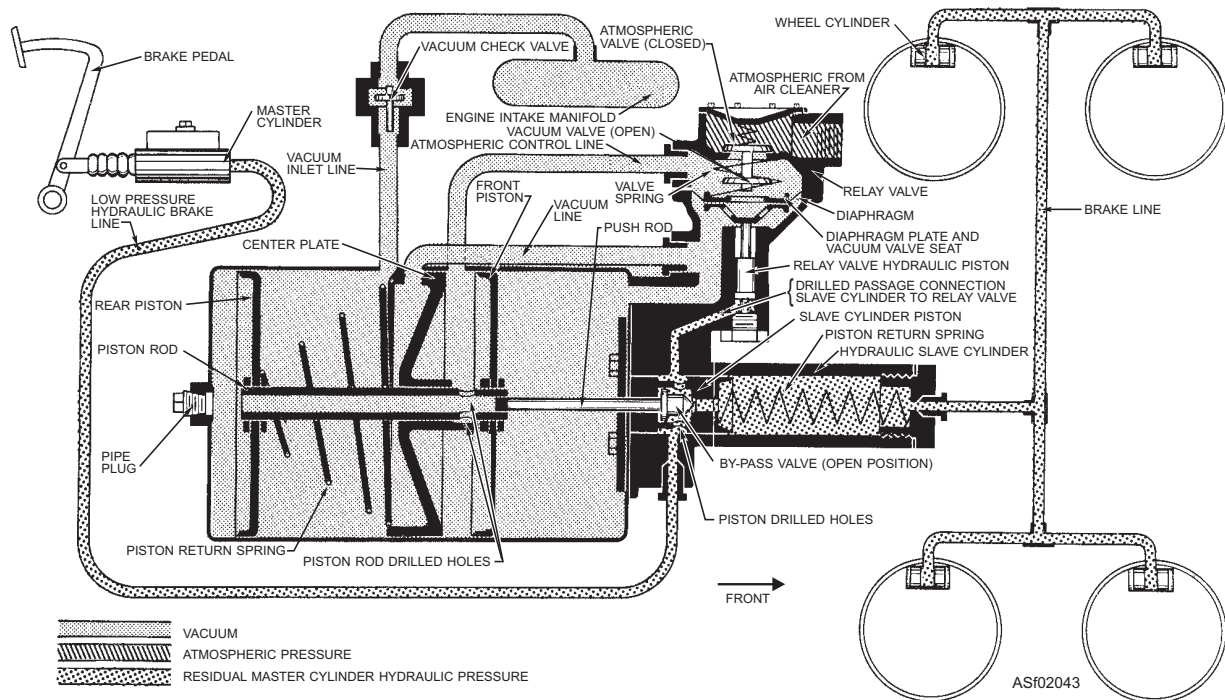
Figure 2-43.—Hydrovac operation—released position.
