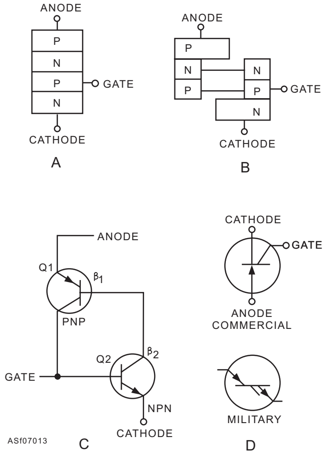
Figure 7-13.—Silicon-controlled rectifier—(A) physical PNPN structure; (B) two transistor analogy; (C) SCR internal circuitry; (D) SCR symbols.
