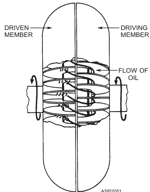
Figure 2-51.—Fluid coupling oil flow “bounce back” effect.
