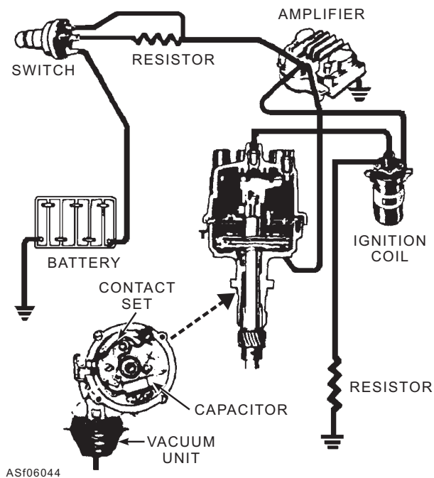
Figure 6-44.—Contact controlled transistor battery ignition system.
