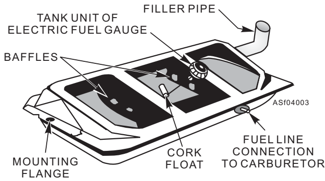
Figure 4-3.—Fuel tank with top cut away.
