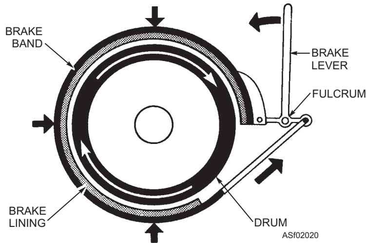
Figure 2-20.—External contracting brake.
