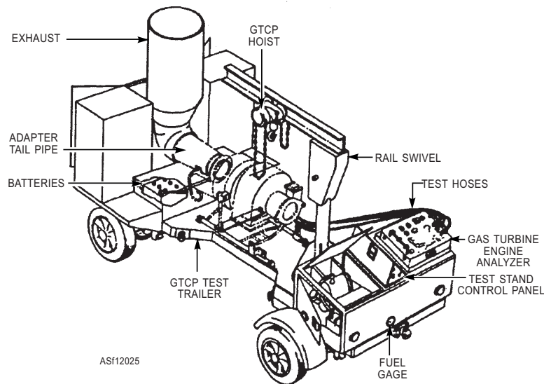
Figure 12-25.—Gas turbine engine test stand.
