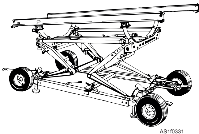
Figure 1-33.—4000A engine removal trailer.
