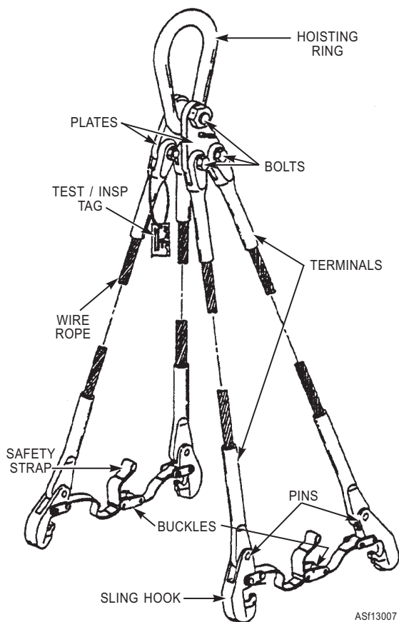
Figure 13-7.—A typical aircraft hoisting sling.
