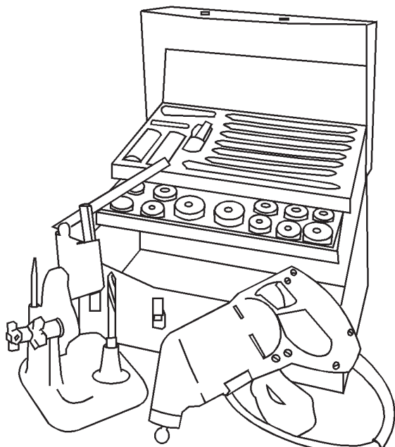
Figure 3-49.—Valve seat grinding equipment.
