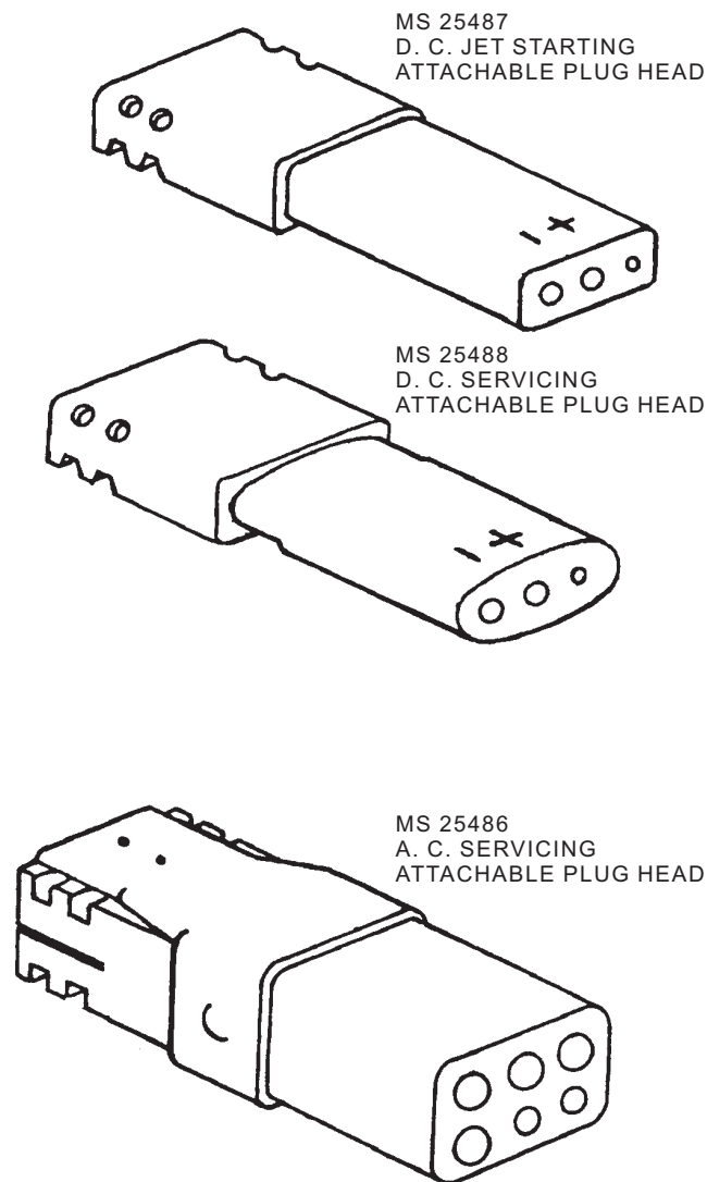
Figure 7-59.—Models of attachable head plugs.
