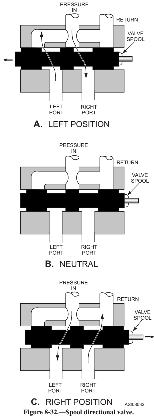
Figure 8-32.—Spool directional valve.
