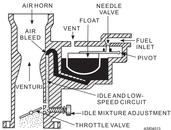
Figure 4-13.—A simple idle and low-speed circuit.
