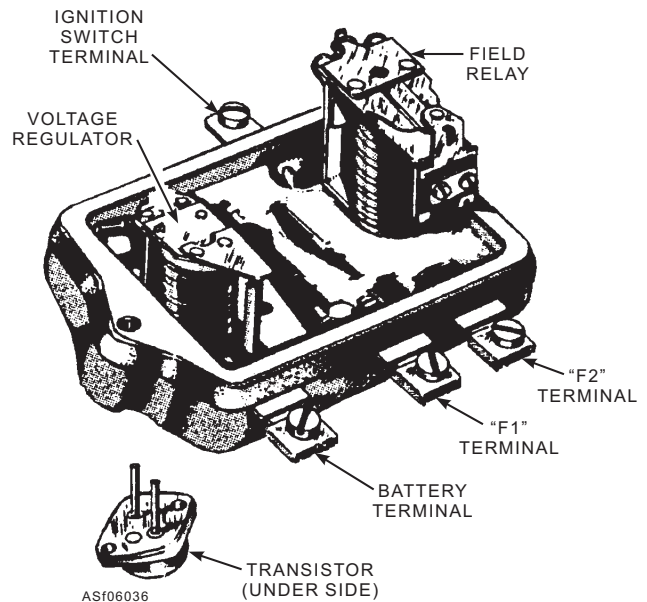
Figure 6-36.—Semitransistorized regulator.
