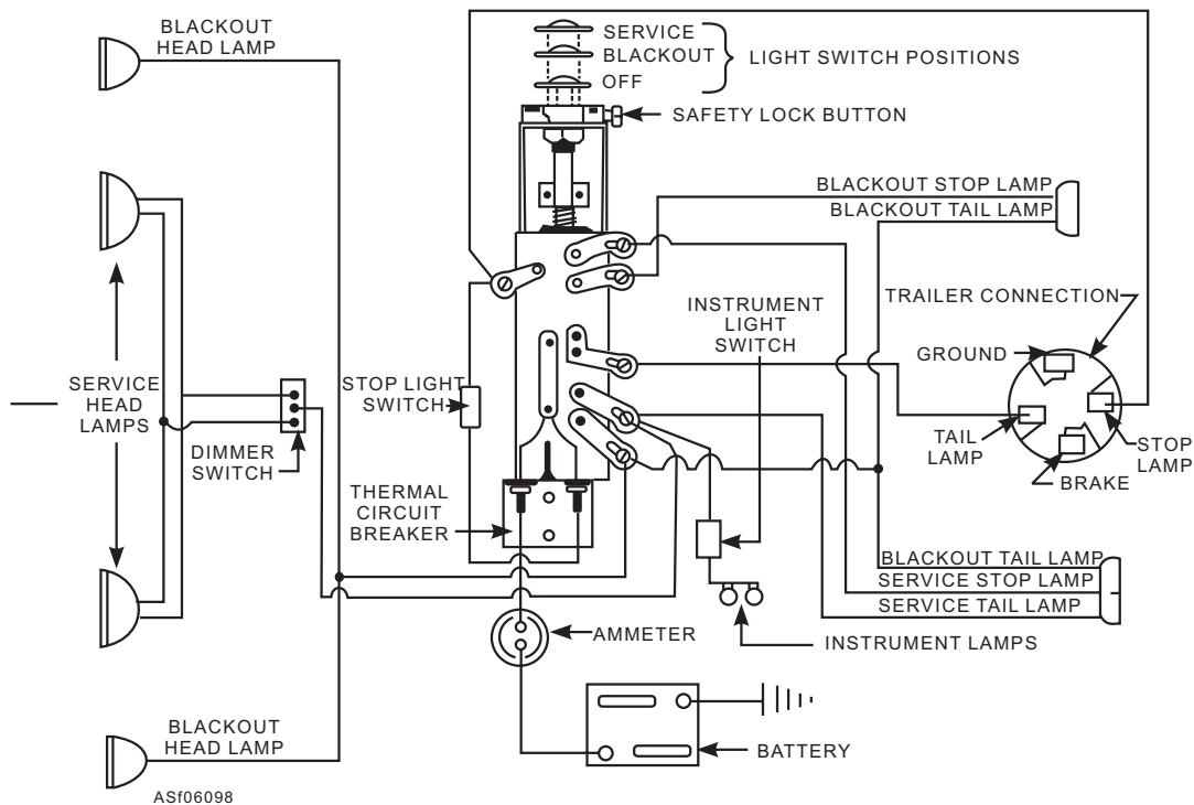
Figure 6-98.—Blackout light switch and connection.
