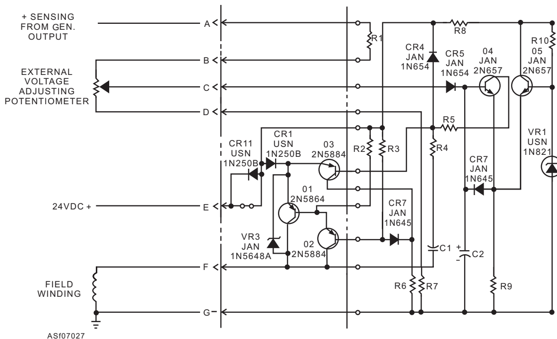
Figure 7-27.—Simplified solid-state dc voltage regulator.
