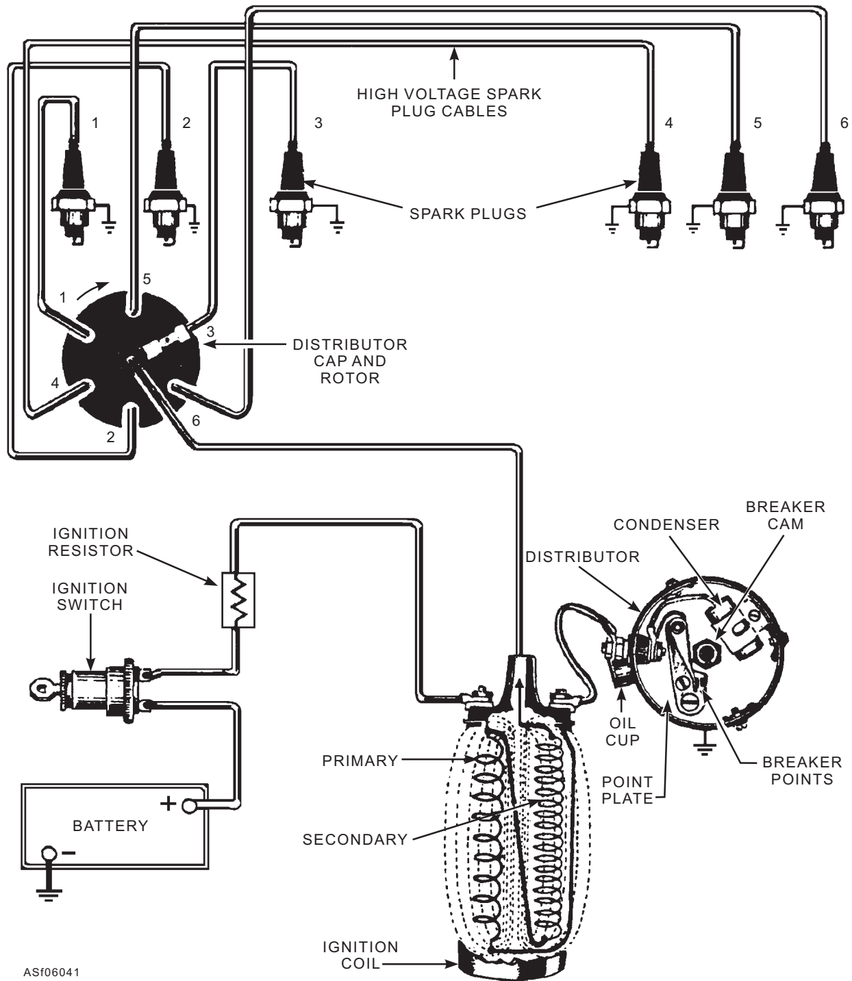
Figure 6-41.—Conventional battery ignition system.
