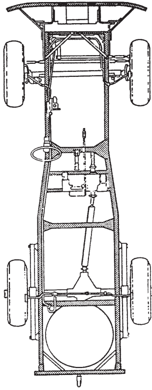
A. AUTOMOTIVE TYPE FRAME
