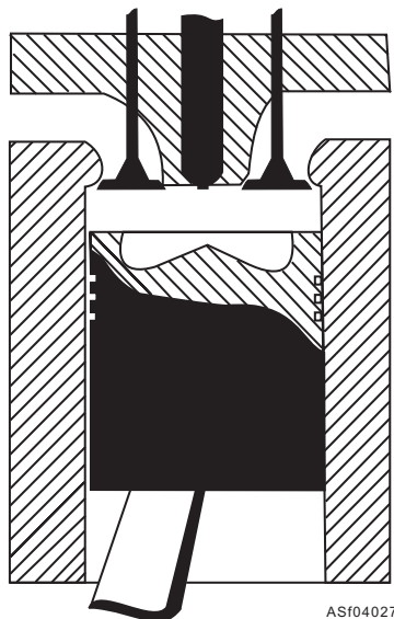
Figure 4-27.—Diesel engine open combustion chamber.
