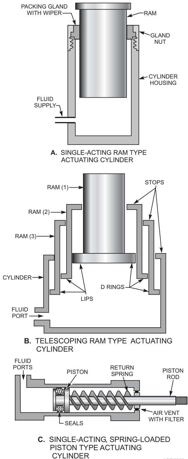
Figure 8-36.—Single-acting actuating cylinders.
