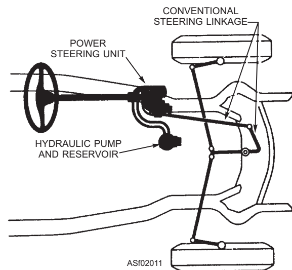
Figure 2-11.—Diagram of a power steering unit.
