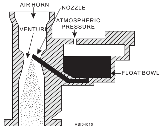
Figure 4-10.—Simplified carburetor.
