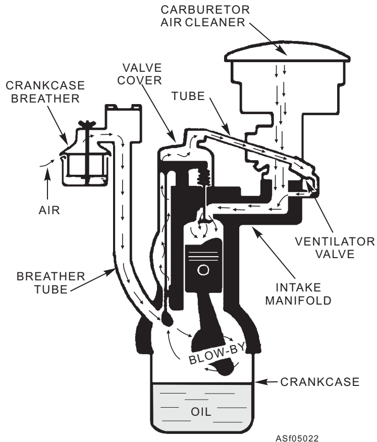
Figure 5-22.—Positive crankshaft ventilation.
