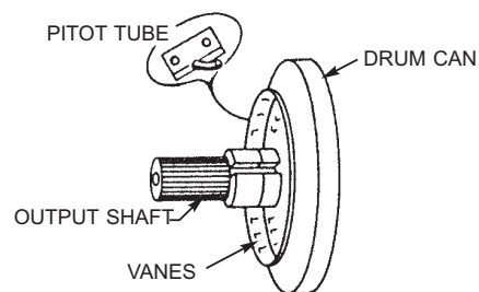
B. FLUID VELOCITY GOVERNOR
