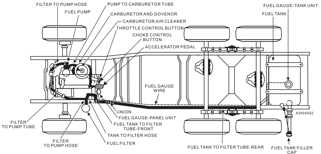
Figure 4-2.—Typical fuel system for a gasoline engine.
