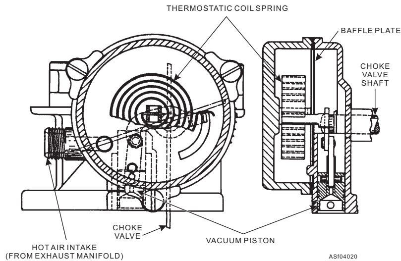
Figure 4-20.—Automatic choke.
