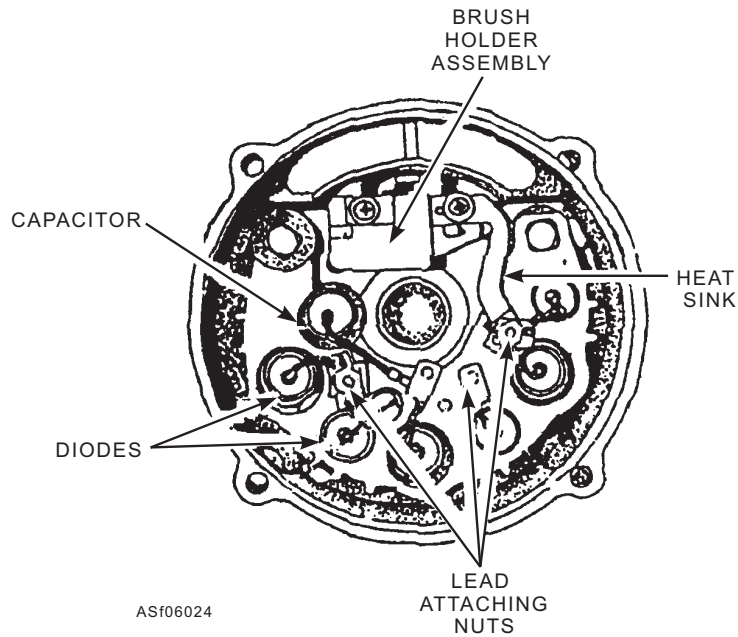
Figure 6-24.—View of an ac generator slip ring end frame assembly.
