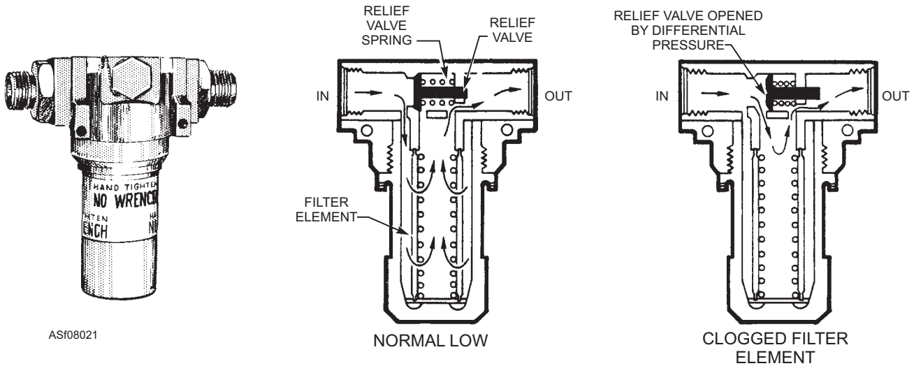
Figure 8-21.—Micronic filter.
