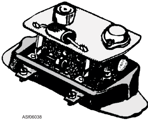
Figure 6-38.—Fully transistorized regulator.
