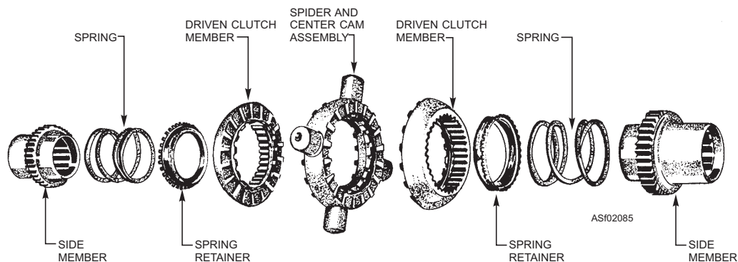
Figure 2-85.—No-spin differential disassembled.
