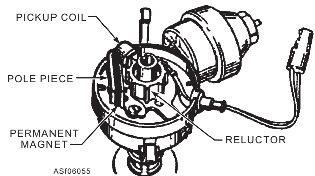
Figure 6-55.—Distributor used with transistorized ignition system.
