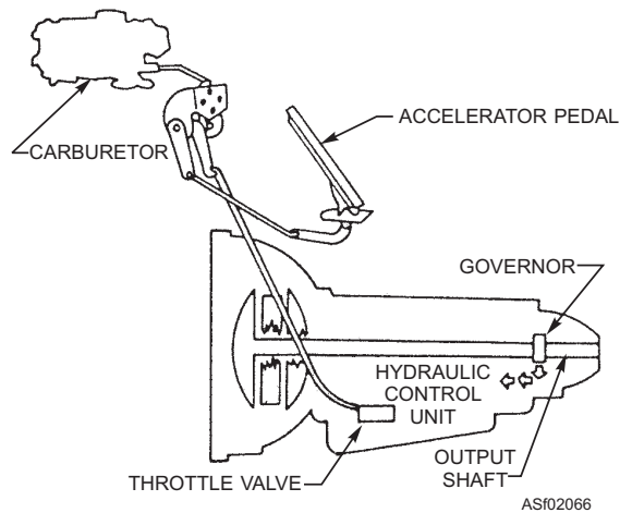
Figure 2-66.—Typical throttle valve and linkage.
