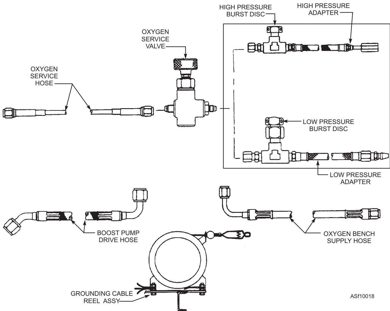
Figure 10-18.—Oxygen/nitrogen servicing/interface equipment.
