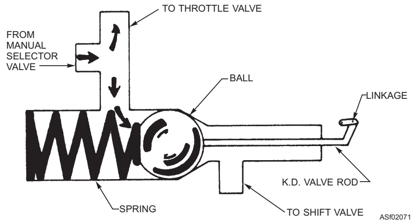
Figure 2-71.—Kickdown valve (separate valve arrangement).
