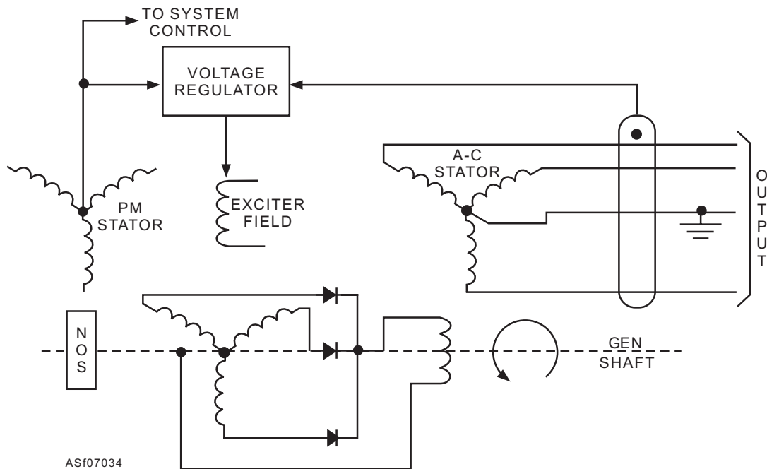
Figure 7-34.—Diagram of a brushless ac generator excitation system.
