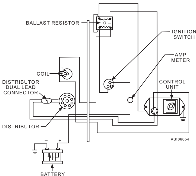
Figure 6-54.—Electronic ignition system.
