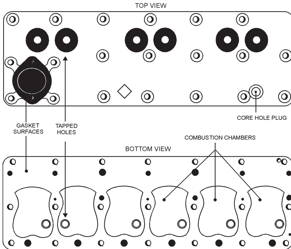
Figure 3-21.—Cylinder head for L-head engine.
