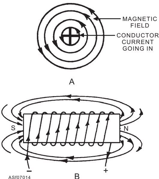
Figure 7-14.—Magnetic field of a current-carrying conductor.
