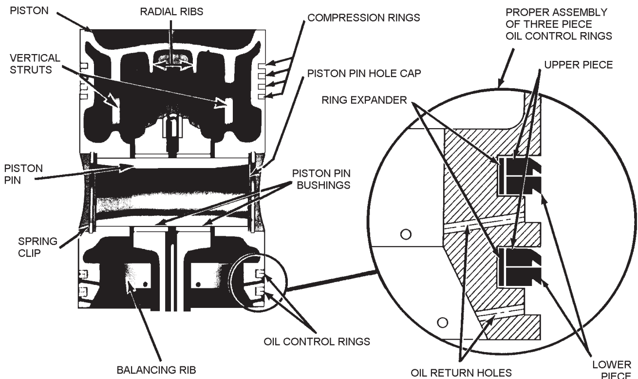
Figure 3-27.—Piston assembly of General Motors series 71 diesel engine.
