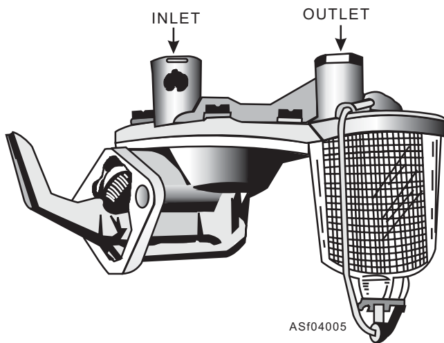
Figure 4-5.—Fuel pump with attached filter bowl.
