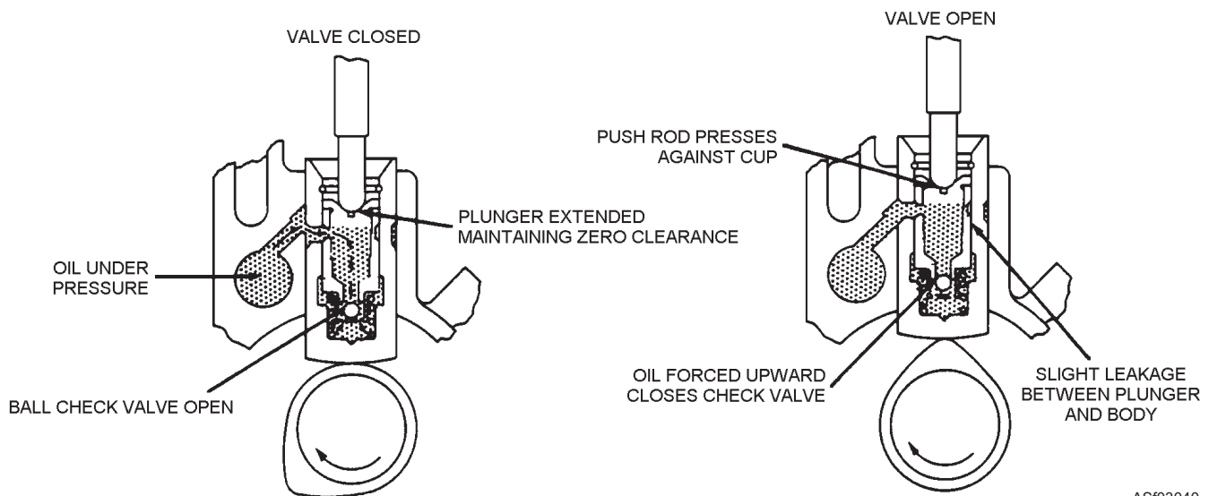
Figure 3-40.—Operation of a hydraulic valve tappet or lifter.
