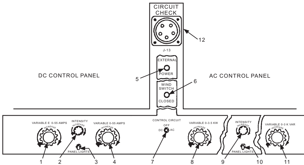
Figure 7-62.—Master control panel.
