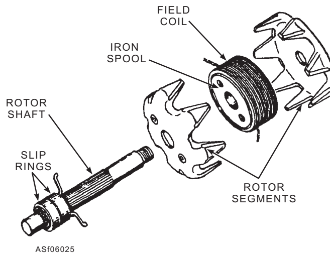
Figure 6-25.—Exploded view of an alternator rotor.
