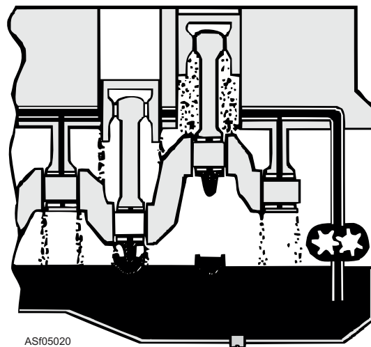
Figure 5-20.—Combination splash force-feed lubrication system.
