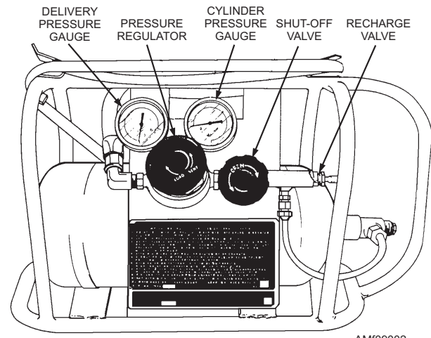
Figure 9-2.—Portable high-pressure nitrogen cylinder.
