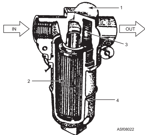
Figure 8-22.—Full flow, bypass hydraulic filter.
